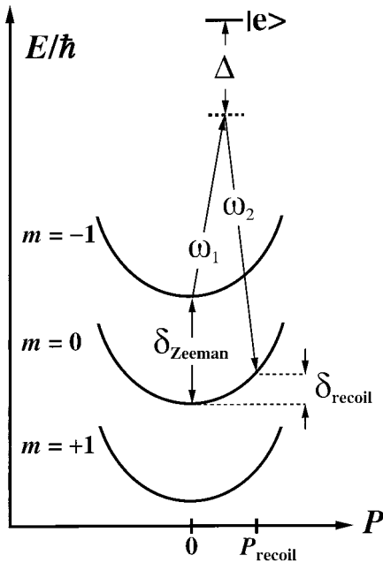
Fig. 1. Principle of the Raman output coupler. Energy conservation requires a relative detuning, \delta = \omega_2 - \omega_1 , between the Raman lasers. Total energy as a function of atomic momentum is plotted, where the parabolas correspond to kinetic energy P^2/2M .
