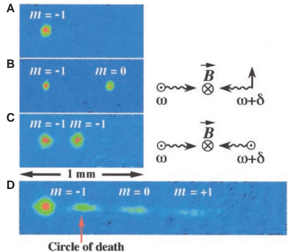
Fig. 2. (A) Condensate before the application of a Raman pulse. (B) \Delta m = +1 transition (19) from a 6\text{-}\mu\text{s} pulse with \delta/2\pi = 6.4 \text{ MHz} . This detuning is chosen to be slightly larger than the 6.27\text{-MHz} resonance frequency to suppress four-photon coupling to the m = +1, 4\hbar k\hat{z} state (25). (C) \Delta m = 0 transition (26) after a 14\text{-}\mu\text{s} Raman pulse with equal laser intensities of 25 \text{ mW/cm}^2 . The relative detuning was \delta/2\pi = -98 \text{ kHz} and the polarizations of both lasers were aligned with \hat{x} . The diagrams to the right of (B) and (C) show the polarization of the lasers with respect to the local magnetic field. We verified that no transitions occurred when incorrect polarizations were used. (D) The rotating magnetic field zero (circle of death) results in Majorana transitions of an output-coupled condensate fraction in the m = 0 state. Arrow denotes physical location of the rotating bias field zero. This is a graphic depiction of Majorana transitions.
