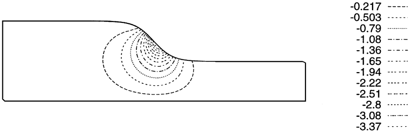
FIG. 5. The total y -velocity v at t = 3.0 . u_{in} = 4.0 .
