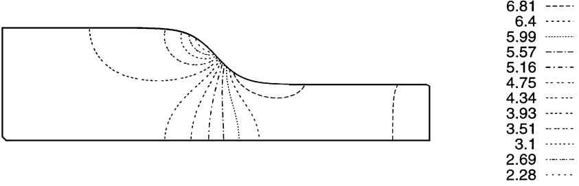
FIG. 4. The total x -velocity u at t = 3.0 . u_{in} = 4.0 .
