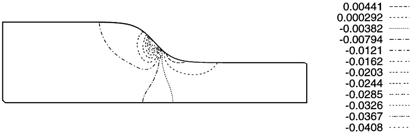
FIG. 6. The incompressible pressure \pi at t = 3.0 . u_{in} = 4.0 .
