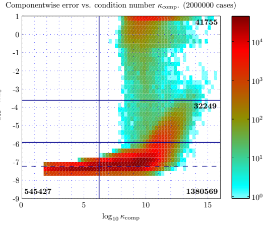
(a) Algorithm 3 with \rho_{\text{thresh}} = 0.5
