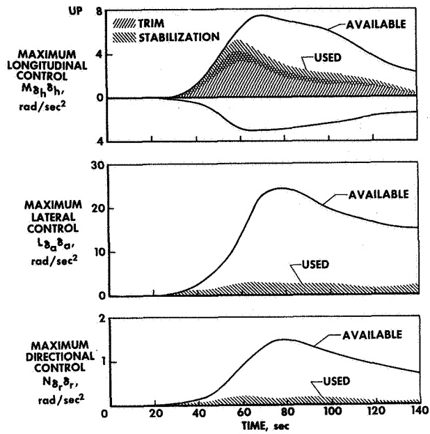
Figure 7.- X-15 reentry controls.
