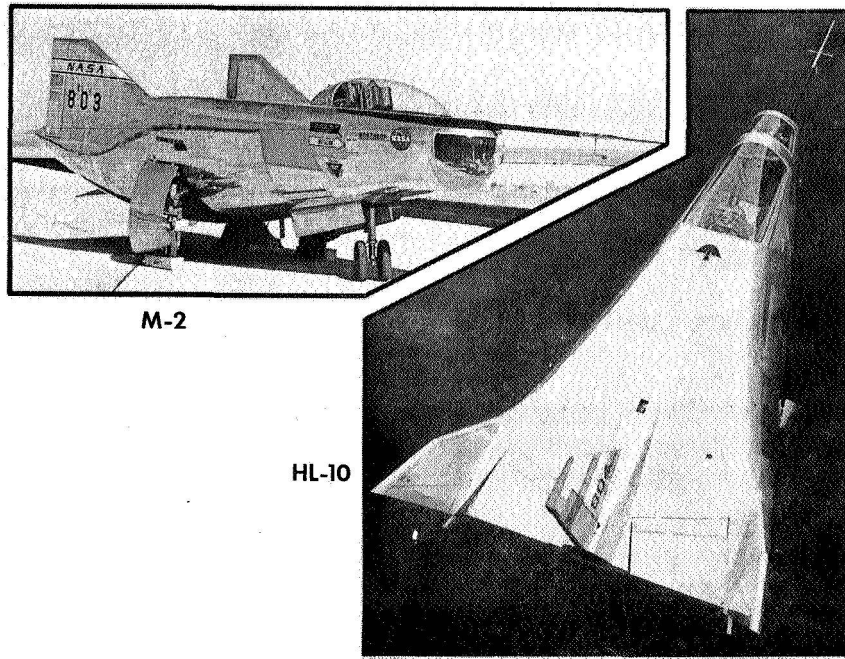
Figure 2.- Lifting-body vehicles.
