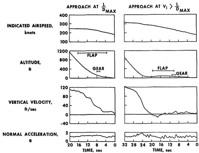
Figure 11.— Comparison of low \frac{L}{D} landing techniques.
