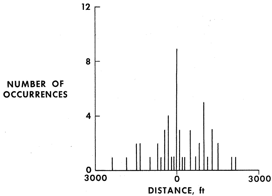
Figure 10.- X-15 touchdown dispersion.
