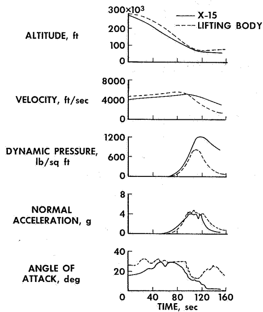
Figure 4. Comparison of X-15 reentry and lifting-body abort recovery.
