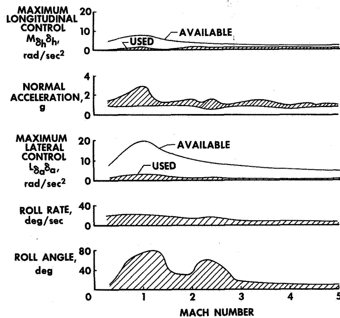
Figure 8.- X-15 maneuvering experience during glide to base.
