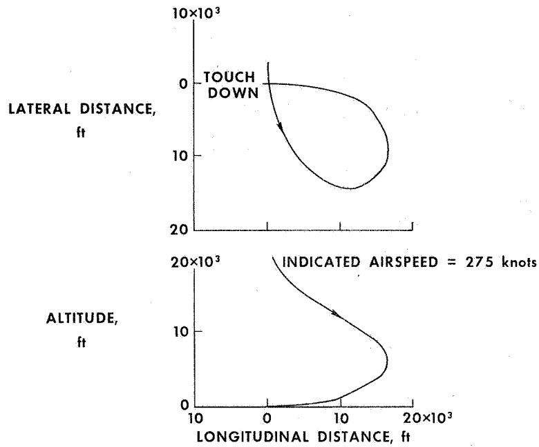
Figure 9.- Typical low \frac{L}{D} circular landing pattern. \frac{L}{D}_{max} = 2.8 ; \frac{W}{S} = 75 lb/sq ft.
