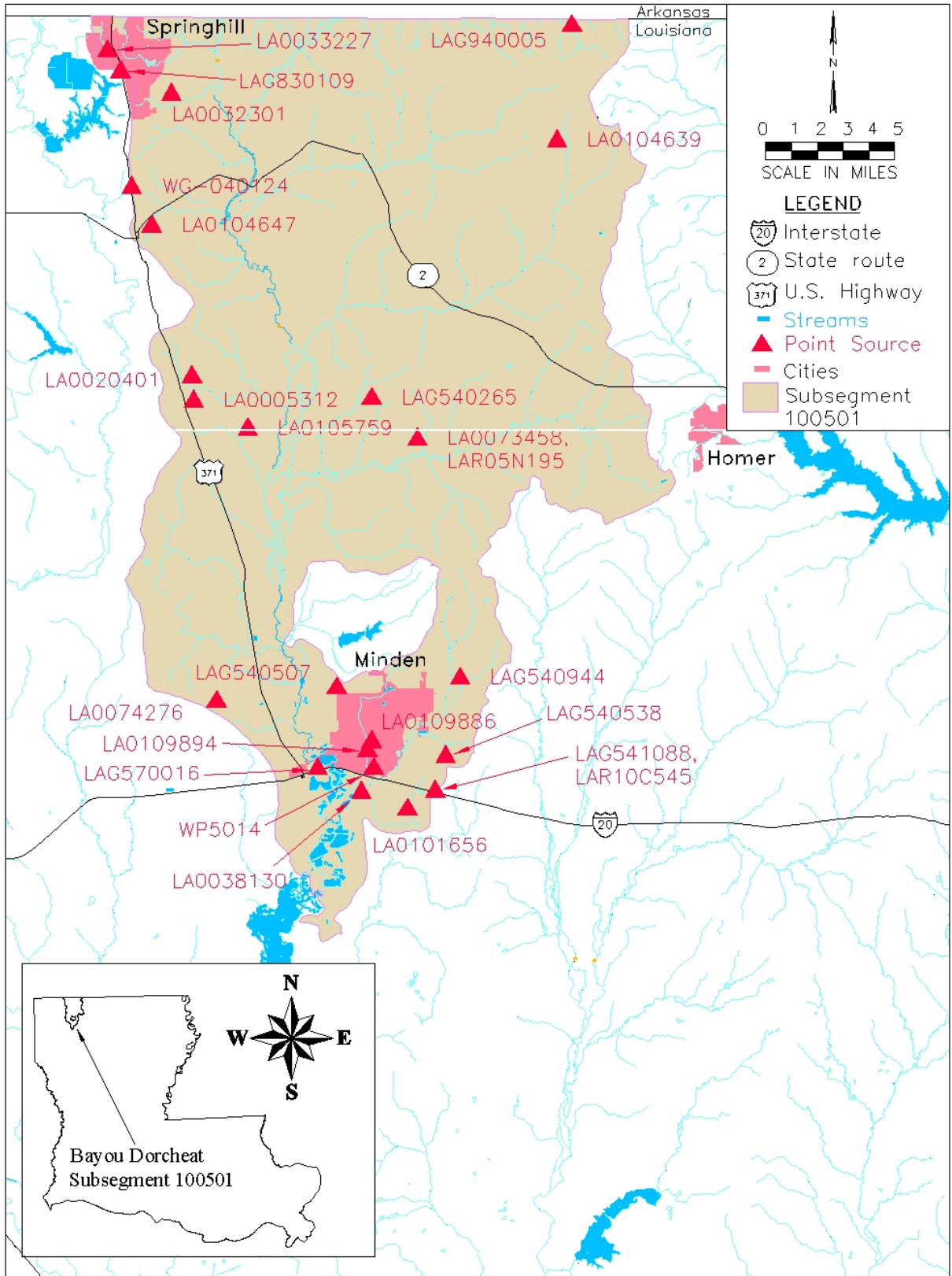
A.3. Point sources in Subsegment 100501.
