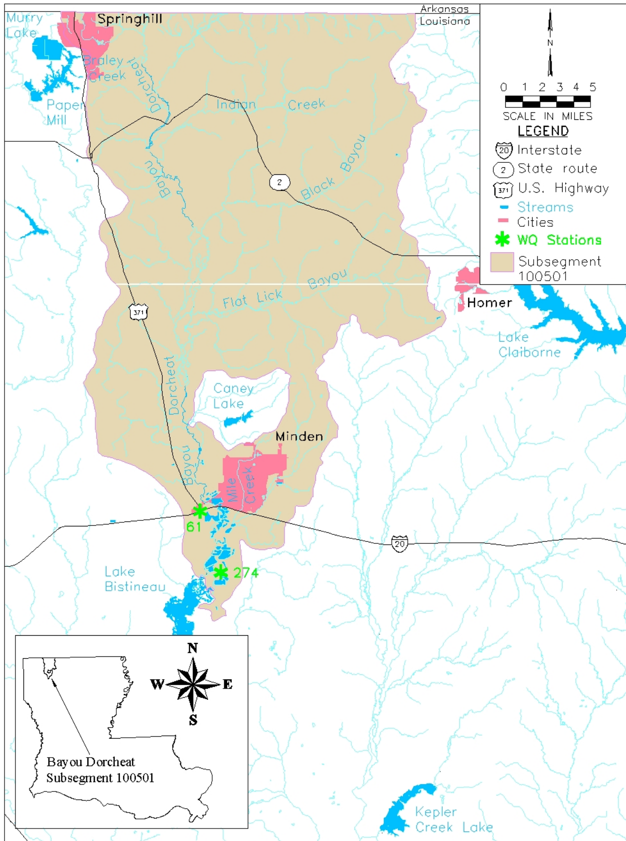
Figure A.1. Bayou Dorcheat watershed map.
