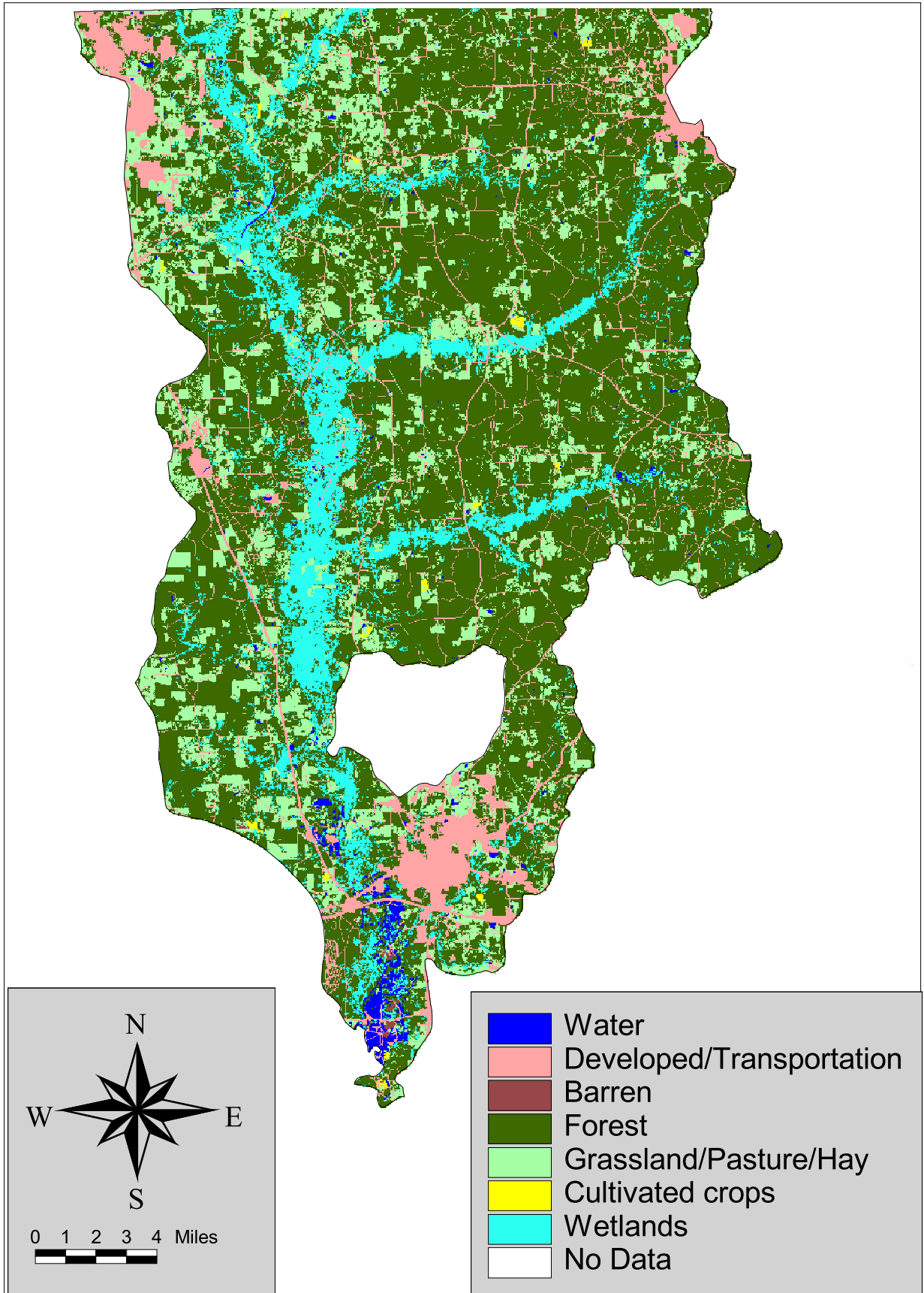
Figure A.2. Land use for subsegment 100501.
