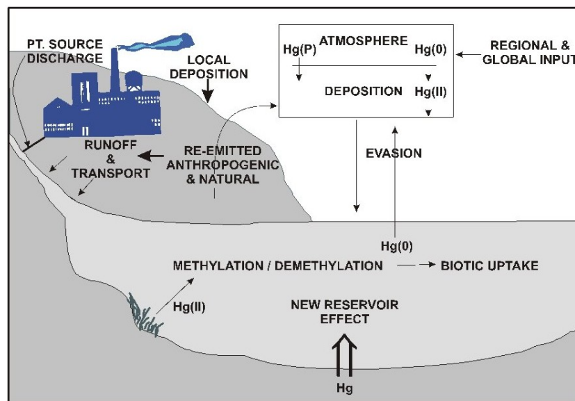
Figure 4.1. General mercury cycle showing atmospheric transport and deposition; point source, nonpoint source, and natural background contributions; and the effects of new reservoirs on mercury release into the environment.
