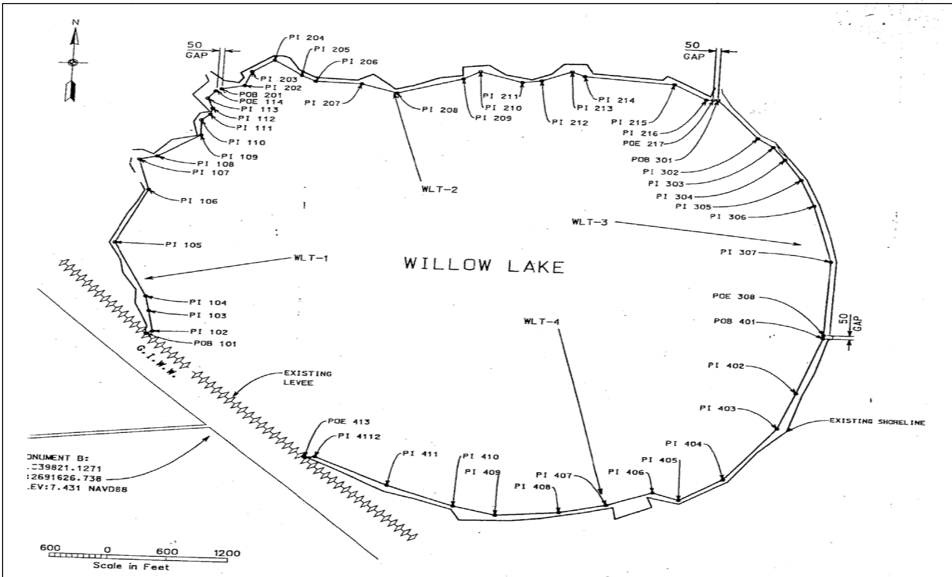
Figure 5. As-built location of earthen terraces within the Willow Lake area of the Sweet/Willow Lake Hydrologic Restoration (CS-11b) project area.
