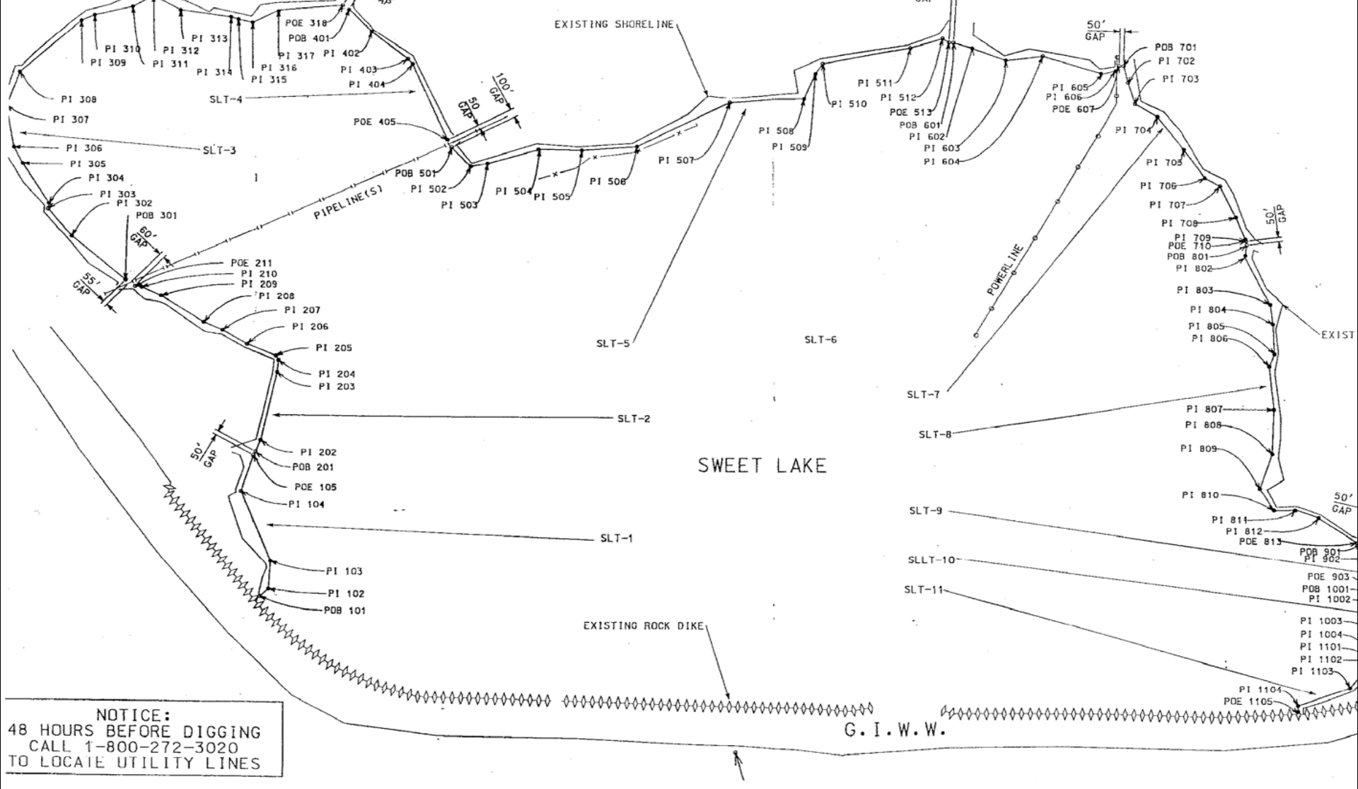
Figure 4. As-built location of earthen terraces within the Sweet Lake area of the Sweet/Willow Lake Hydrologic Restoration (CS-11b) project area.
