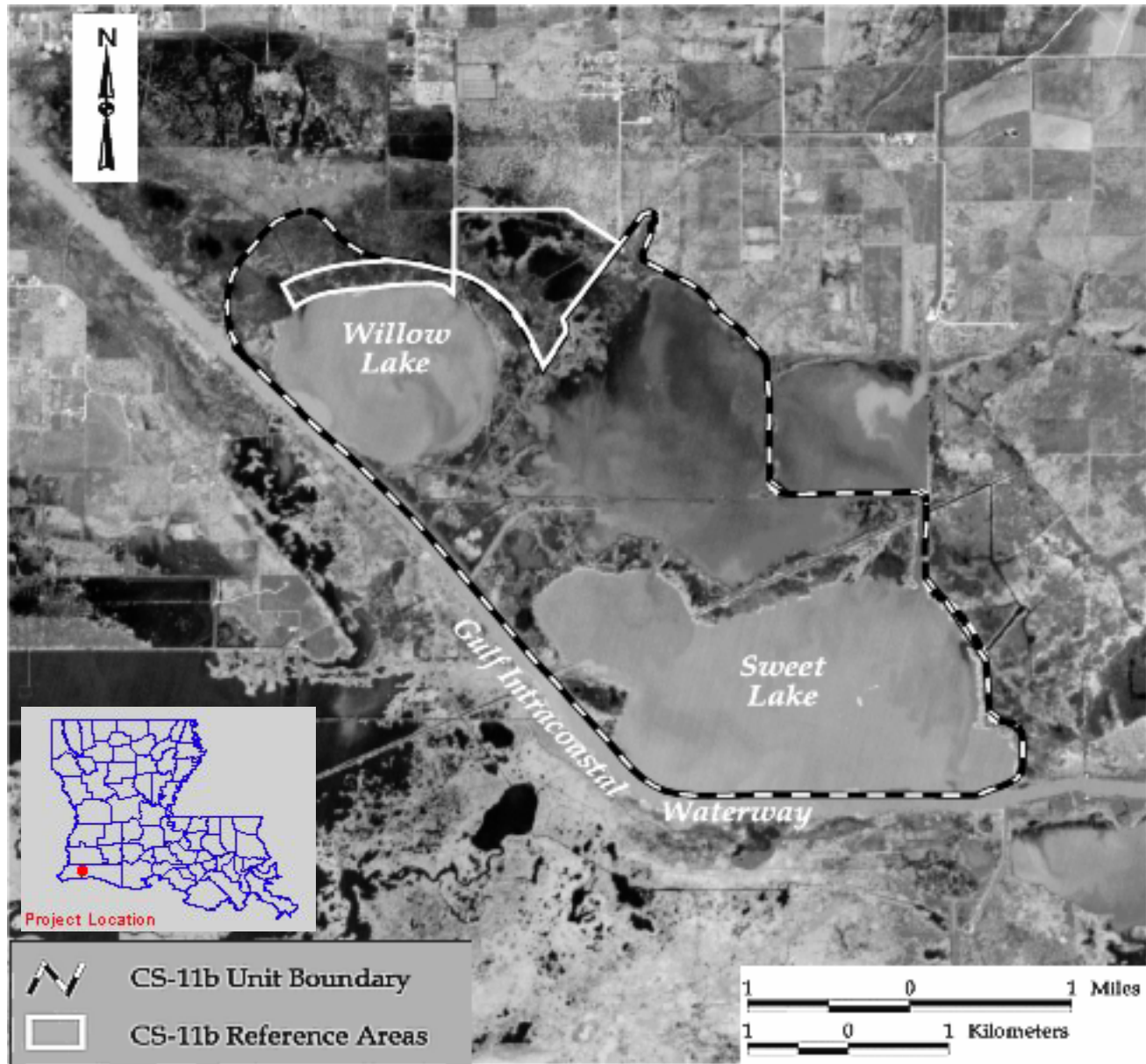
Figure 1. 1994 Sweet/Willow Lake Hydrologic Restoration (CS-11b) project and reference features.
