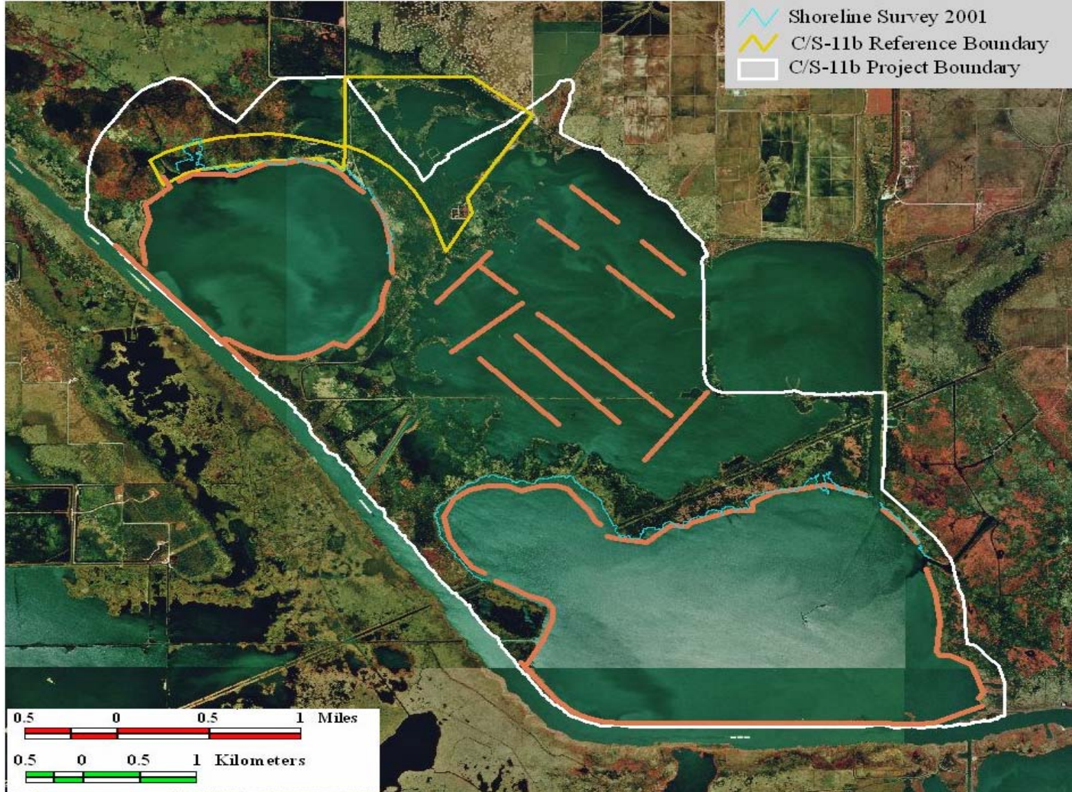
Figure 3. 2001 DGPS Shoreline survey of the Sweet/Willow Lake Hydrologic Restoration (CS-11b) project area and proposed location of the earthen terraces within the project area.
