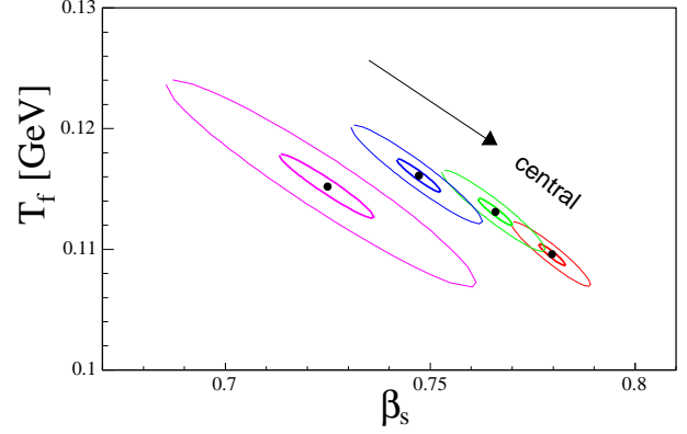
FIG. 8: Kinetic freeze-out temperatures T_f and transverse flow velocities \beta_s resulting from a simultaneous fit of \pi^\pm , K^\pm , p and \bar{p} spectra to Eq. 1 as a function of collision centrality. The curves correspond to increasing centrality as \beta_s increases. The points represent the best fit values of T_f and \beta_s while the contours indicate 1\sigma and 3\sigma levels. The systematic errors are \leq 5\% and are not included in the figure.
