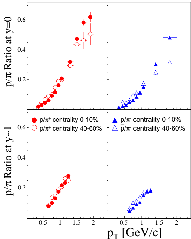
FIG. 11: p/\pi^+ (left) and \bar{p}/\pi^- (right) ratios as a function of p_T at y = 0 (top) and y \sim 1 (bottom). Closed and open symbols represent central (0–10%) and peripheral (40–60%) collisions, respectively. Only statistical error bars are shown.
