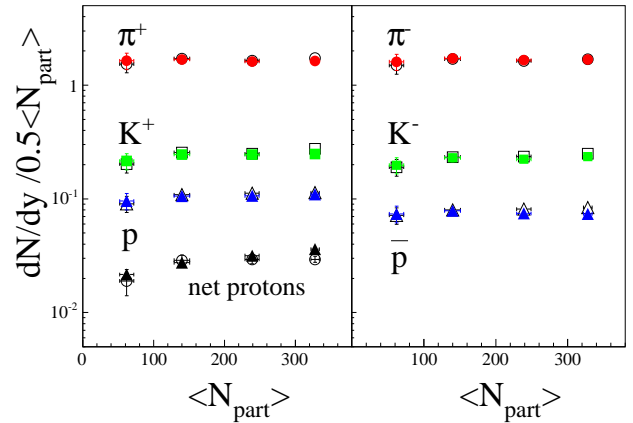
FIG. 9: Rapidity density ( dN/dy ) per participant pair ( N_{part}/2 ) as a function of N_{part} for \pi^+ , K^+ , p , net proton (left) and \pi^- , K^- , \bar{p} (right). Open symbols represent at y = 0 , and closed symbols are for y \sim 1 . The error bars represent the statistical errors only.
