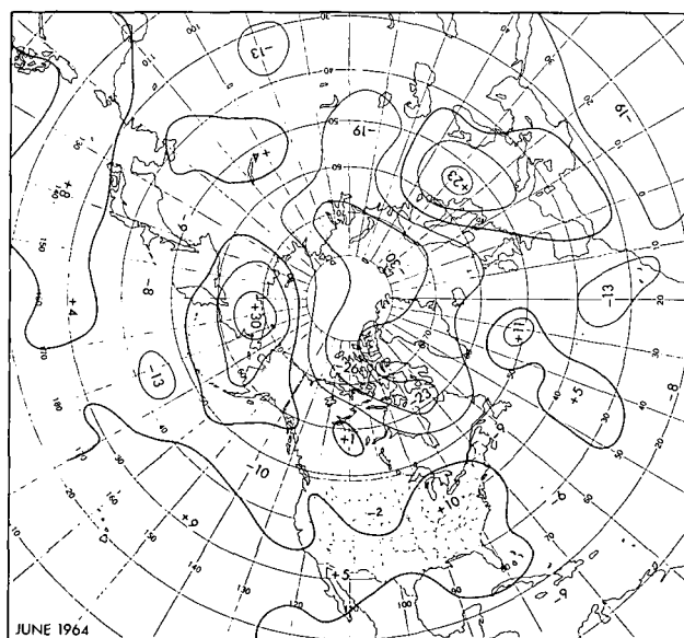
FIGURE 3.—Mean 700-mb. height departures from normal for June 1964 drawn at intervals of 100 ft. with centers in tens of feet and zero isopleth heavy.
