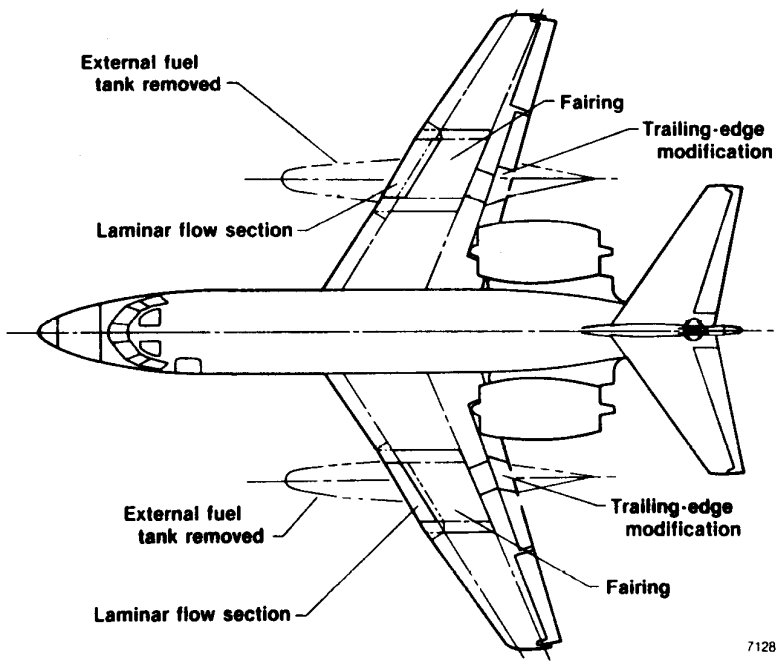
Fig. 2 JetStar airplane modifications.
