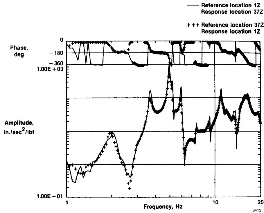
Fig. 7 Impulsive sine reciprocity comparison.
