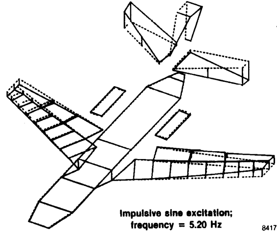
Fig. 9 Empennage roll and fuselage torsion mode shape.
