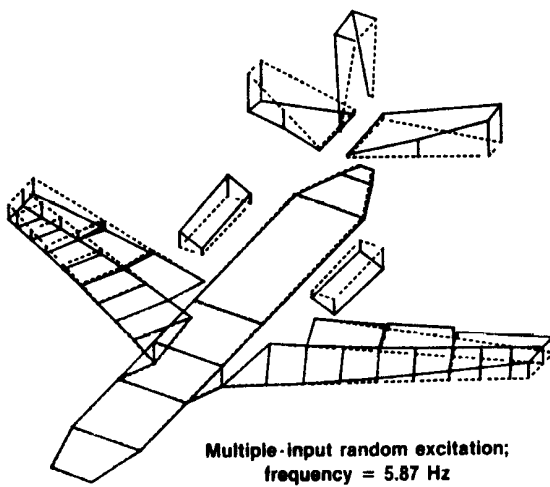
Fig. 10 Empennage roll, fuselage torsion, and engine pylon bending mode shape.
