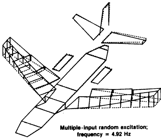
Fig. 8 Symmetric first wing bending mode shape.
