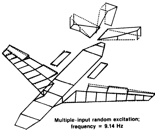
Fig. 12 Vertical fin bending mode shape.
