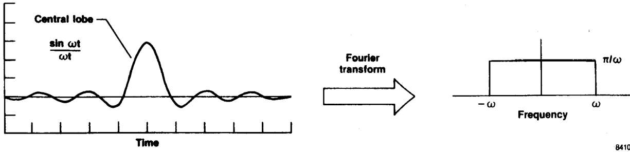
Fig. 1 The \sin \omega t / \omega t function and its Fourier transform.
