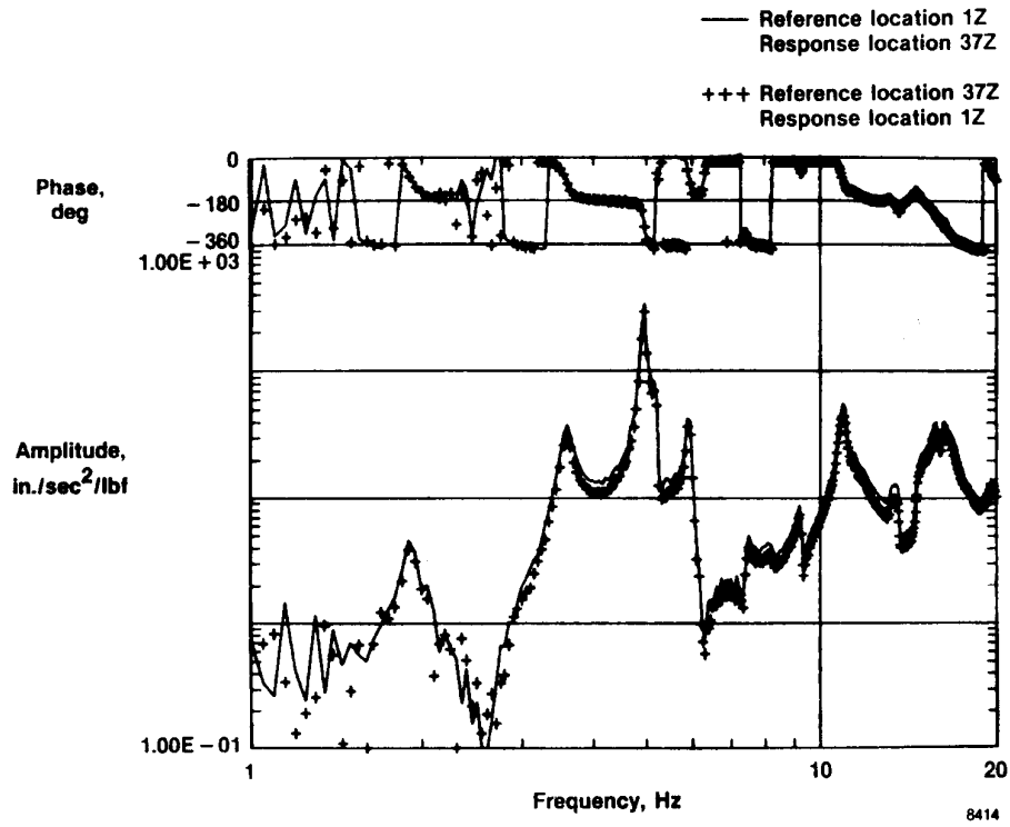
Fig. 6 Multiple-input random reciprocity comparison.
