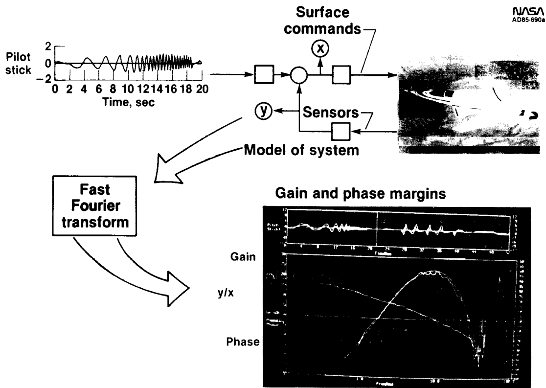
Figure 20. Flight-determined frequency response for unstable airframes.
