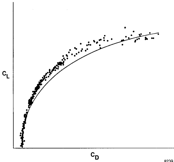
Figure 23. X-29 real-time drag polar.
