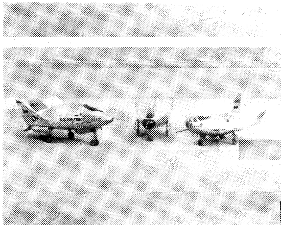
Figure 5. M-2, HL-10, and X-24A.
