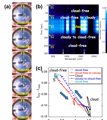
(a) Total sky images on 18 May 2007, and (b) plot of SWS normalized zenith radiances. In (b), arrows pointed at the time axis correspond to the times of the images shown in (a), while arrows pointed at the wavelength axis correspond to 870 and 1640 nm. (c) is the plot of radiance difference vs sum at 870 and 1640 nm. Letters S and E indicate the start and end of the time series. Two arrows show the flow of time evolution. A remarkable linear relationship is found in the transition zone.
