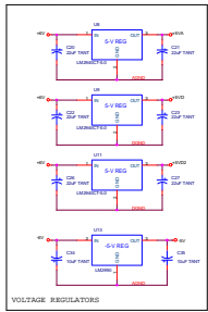
VOLTAGE REGULATORS
