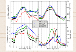
Figure 2. Diurnal cycle of surface variables simulated for the same 13 cases as in Fig. 1. LM: Lokalmmodell of the German Weather Service (DWD). Strong deviations from observations are found in all variables. Increasing model resolution and shutdown of convection parameterization results in an improvement of the simulation of precipitation.
