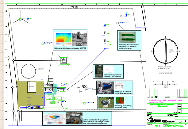
Figure 9. Result of site preparation and operation planning process, which was organized within a contract between Los Alamos National Laboratory and University of Hohenheim. It comprised the work of the local government and an engineering office and included site rental, building application, site ground work, logistics (power, internet, phone), fence, outreach, etc. The German COPS and GOP contributions are highlighted.
