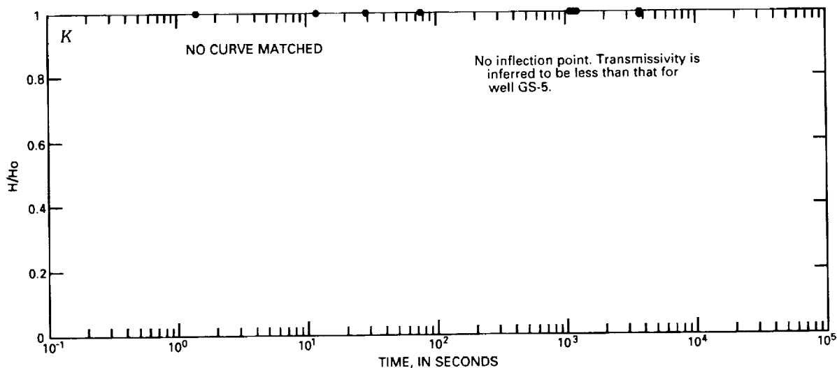
Figure 42K. Slug-test results for well GS-5.
