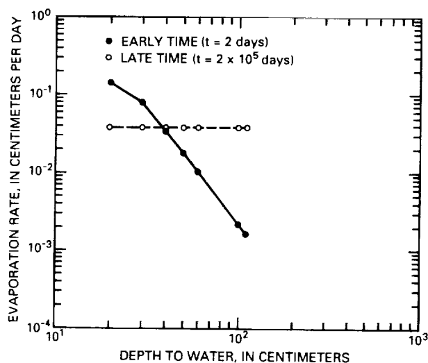
Figure 39.--Sensitivity analysis of the effect of varying model value of depth to the water table.
