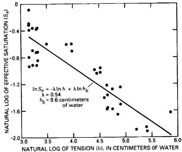
Figure 35.--Relation between the natural logarithm of effective-saturation data and the natural logarithm of soil-moisture tension.
