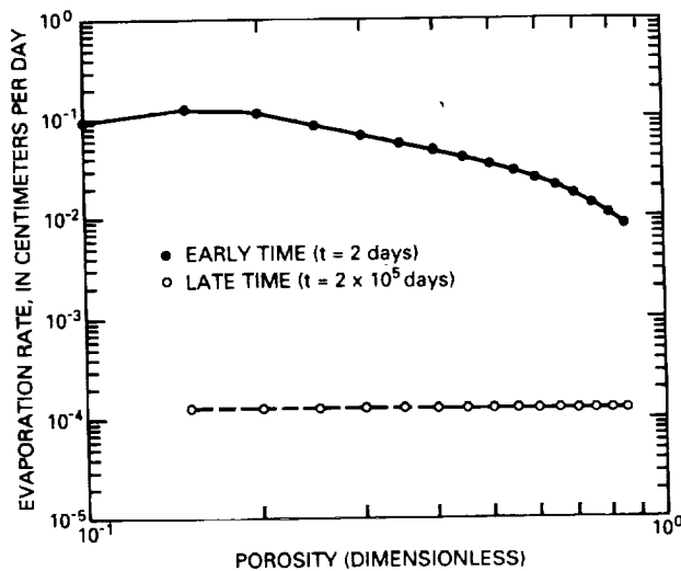
Figure 45.--Sensitivity analysis of the effect of varying model value of the porosity.
