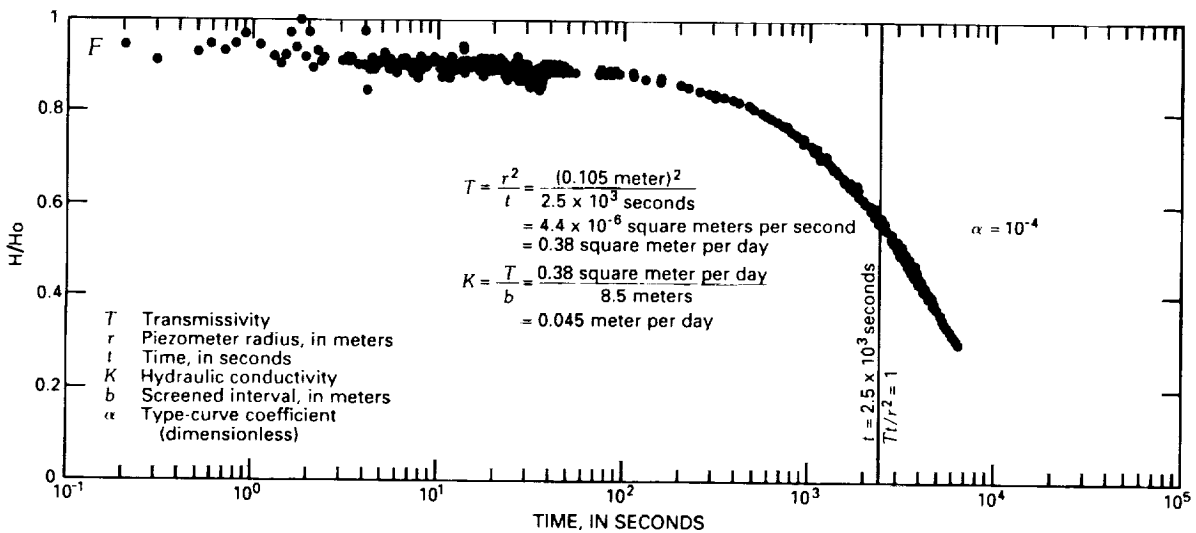
Figure 42F. Slug-test results for well 5.
