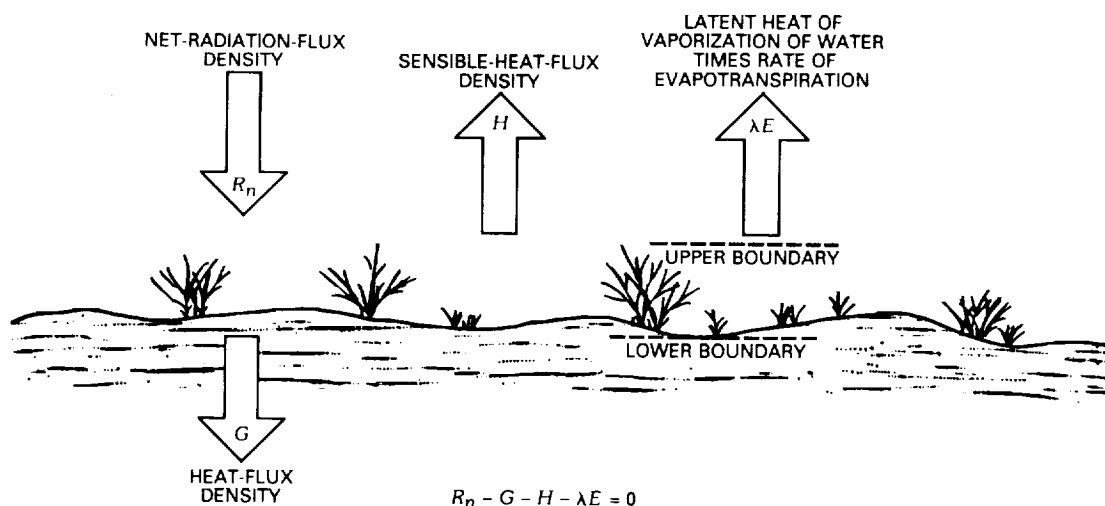
Figure 18.--The energy-balance method.
