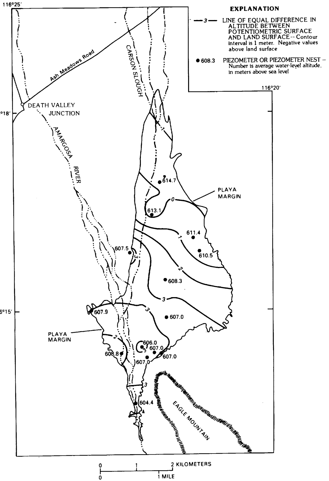
Figure 12. Difference in altitude between potentiometric surface and land surface.
