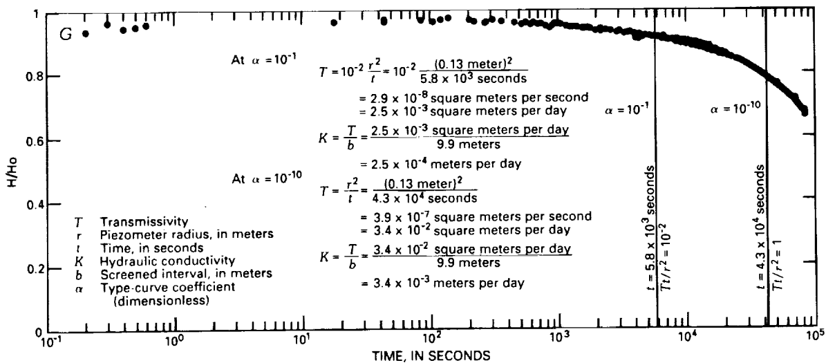
Figure 42G. Slug-test results for well 10.
