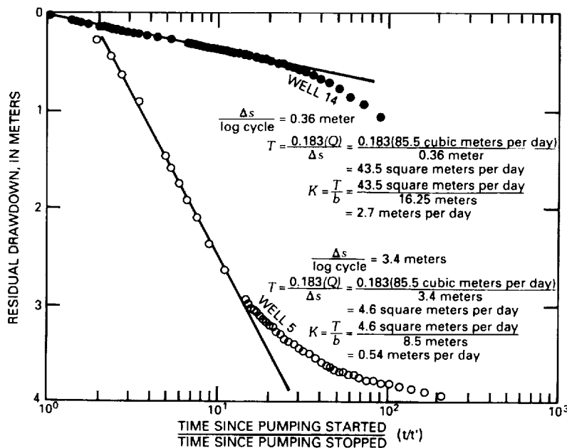
Figure 14. Recovery tests for wells 5 and 14.
