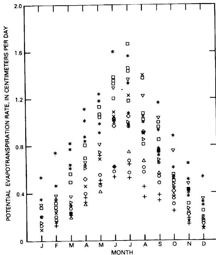
Figure 28.--Summary of potential evapotranspiration estimation results.
