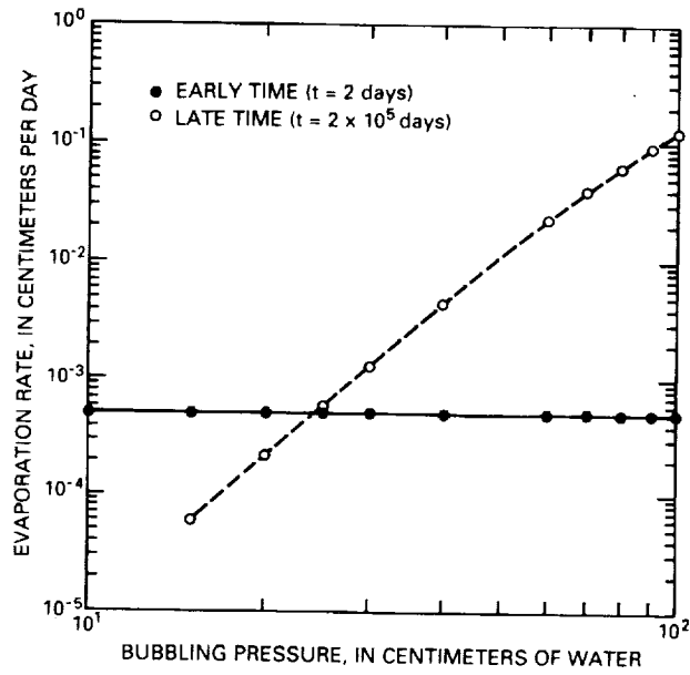
Figure 36.--Sensitivity analysis of the effect of varying model value of the bubbling-pressure head, h_b .
