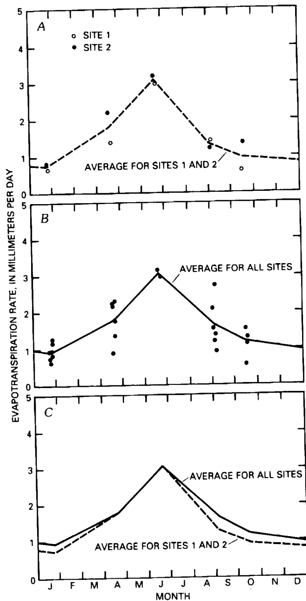
Figure 26.--Evapotranspiration rates for A, site 1, site 2, and the average; B, all sites and the average; and C, comparison of two methods of analysis.
