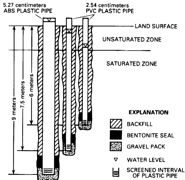
Figure 11. Typical piezometer nest construction.
