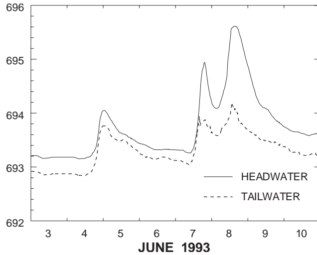
Figure 7. The headwater and tailwater continuous-stage data at Cenacle culvert (sites 5 and 7) on Spring Brook, a tributary to the West Branch Du Page River, in Illinois.
