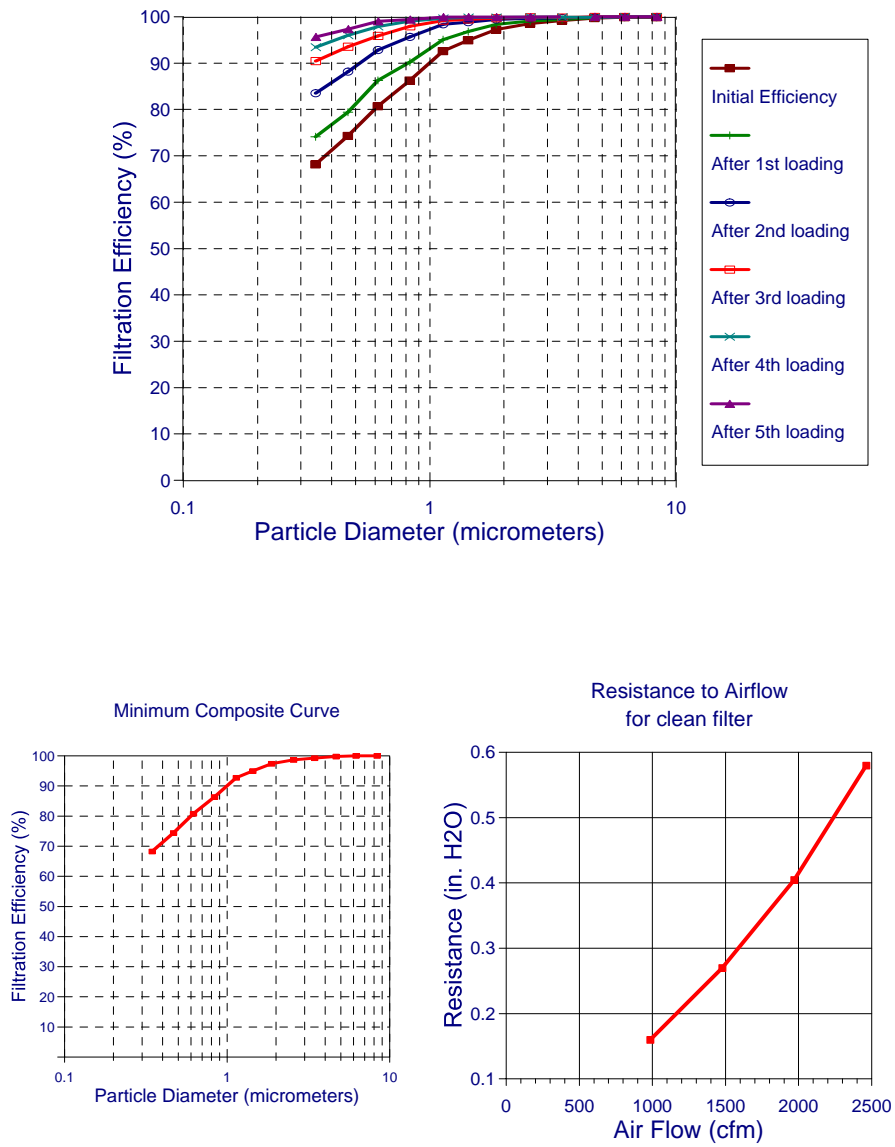
Figure A-1. Filtration Efficiency and Flow Resistance Curves for Aeolus Synthetic Minipleat V-cell SMV-M14-2424 Filter.
