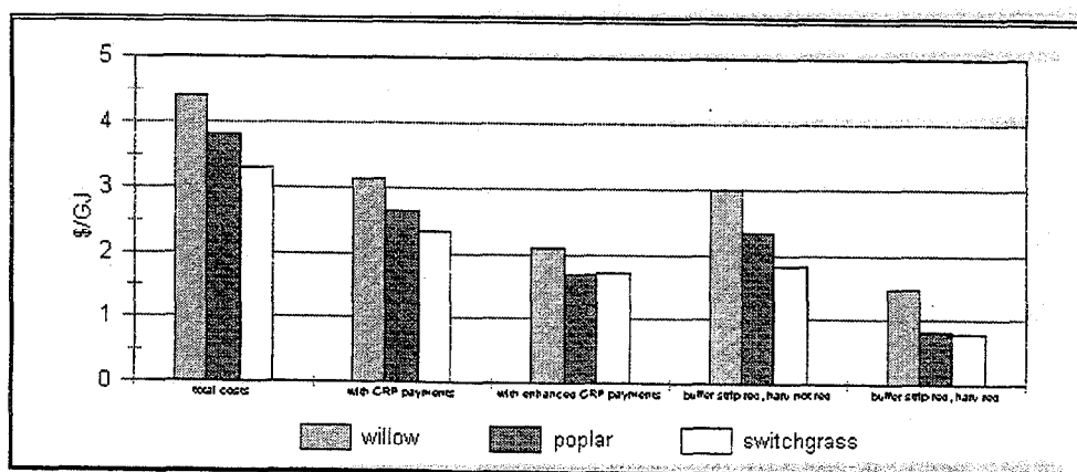
Fig. 12. Costs of willow, poplar, and switchgrass at 11.2 dry Mg/ha-year (5 dry tons/ac-year).
