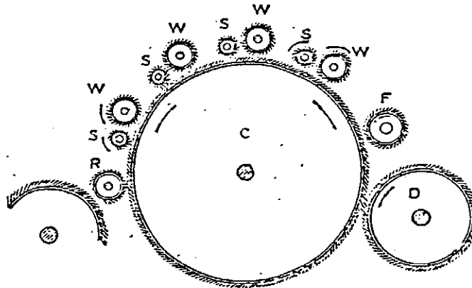
Figure 1: Diagram Showing Parts of Card.
