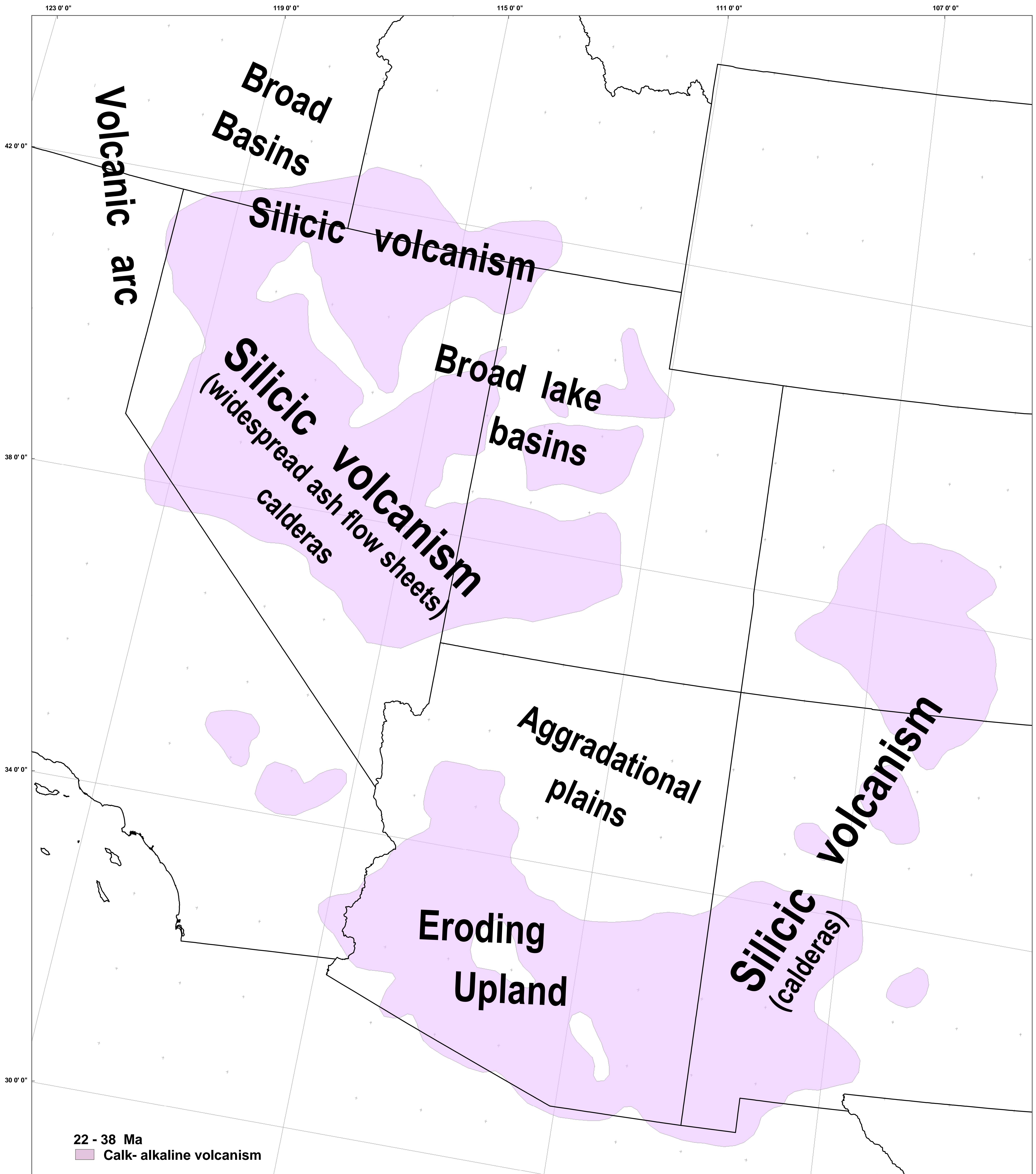
Sheet 18. Interpretive paleotectonic map of SW United States for the early part of Paleogene time (22-38 Ma). Regions with large volumes of calc-alkaline volcanic rock are shaded pink.
