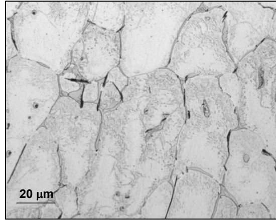
Figure 9. Grain boundary eutectic phase and Fe, Si precipitates in as-deposited Al 2219.
