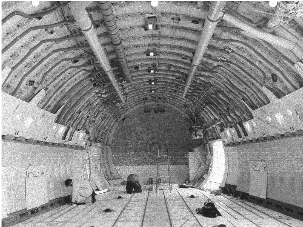
Figure 17. 747-400 Main Deck Cargo Compartment
