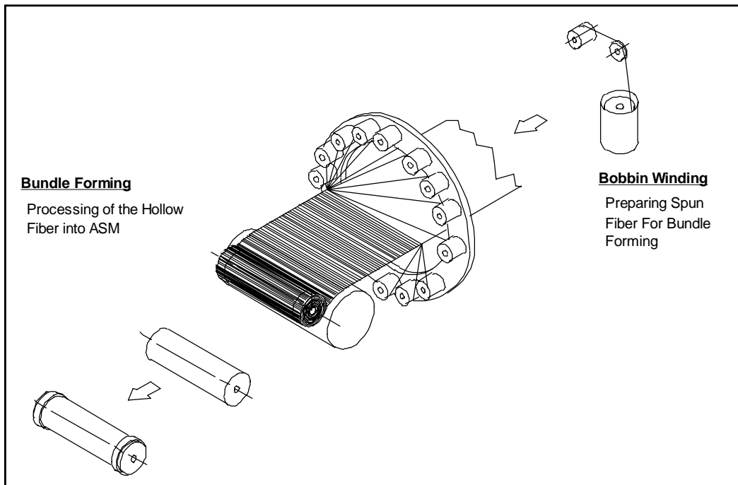
Figure 5. Complete ASM Manufacturing Capabilities
