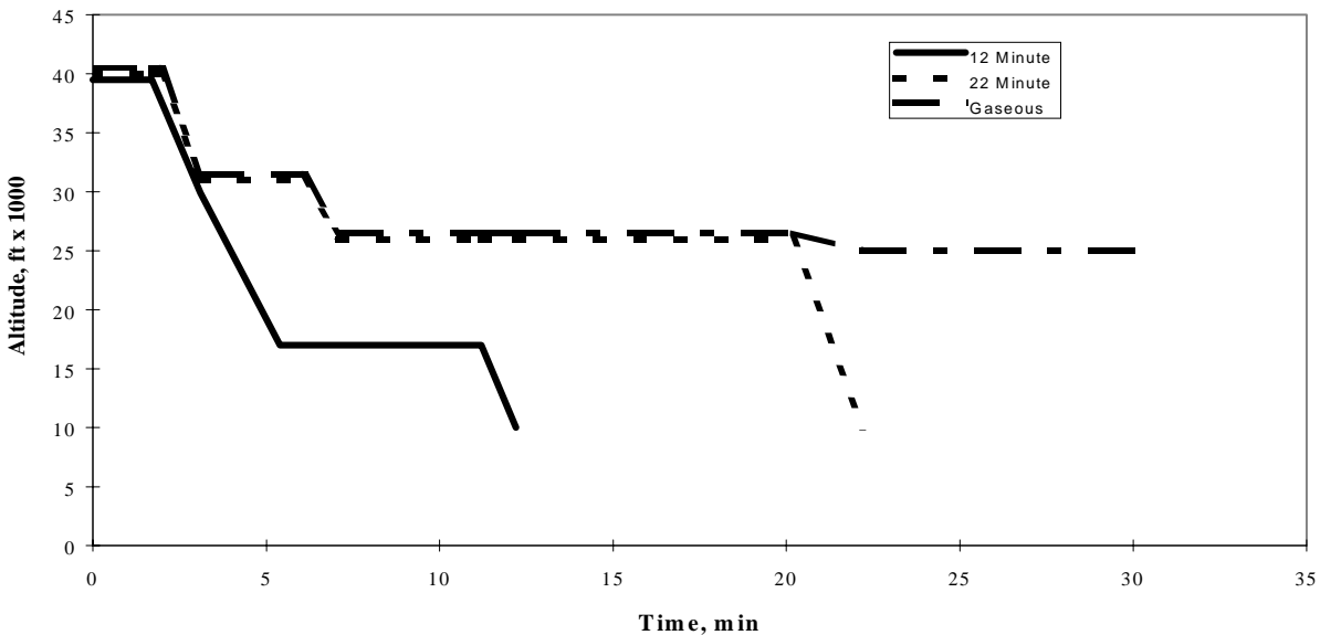
Figure 18. Aircraft Descent Profiles
