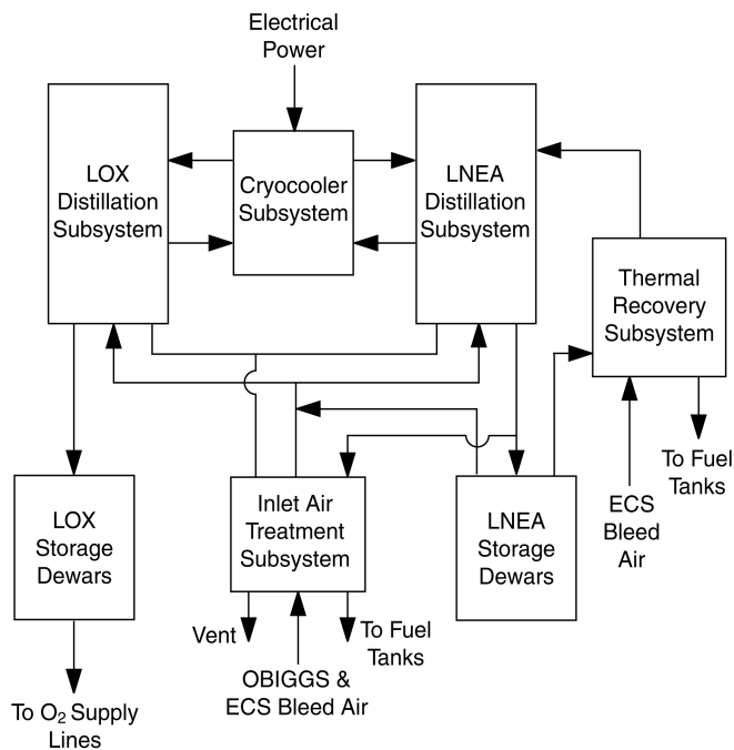
Figure 30. TALON System Description
