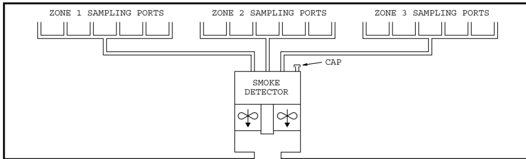
LOWER CARGO COMPARTMENT (TYPICAL)
