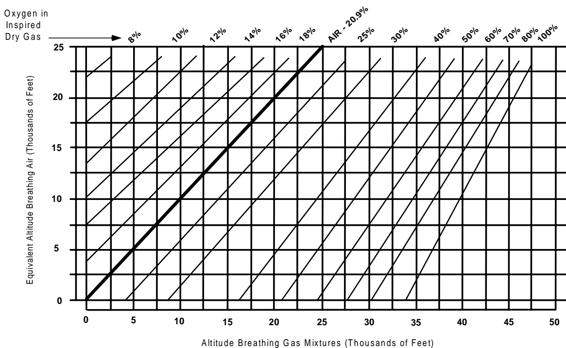
Figure 21. Equivalent Altitude
