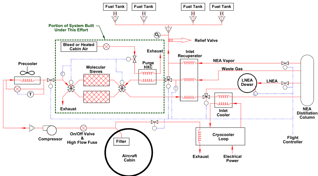
Figure 26. Precooling/Recuperation Subsystem
