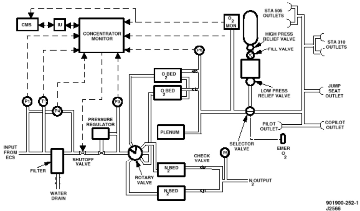
Figure 2. V-22 OBOGS/OBOGS Detailed Schematic
