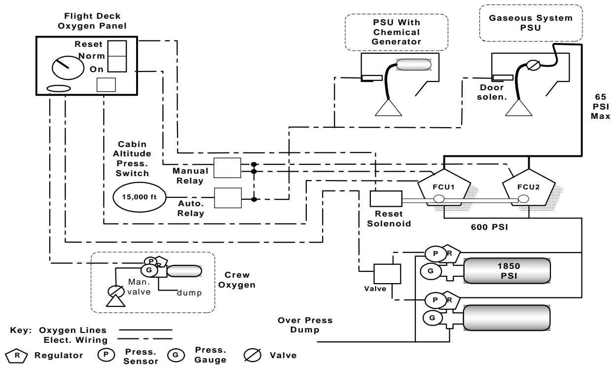
Figure 19. Gaseous Oxygen System
