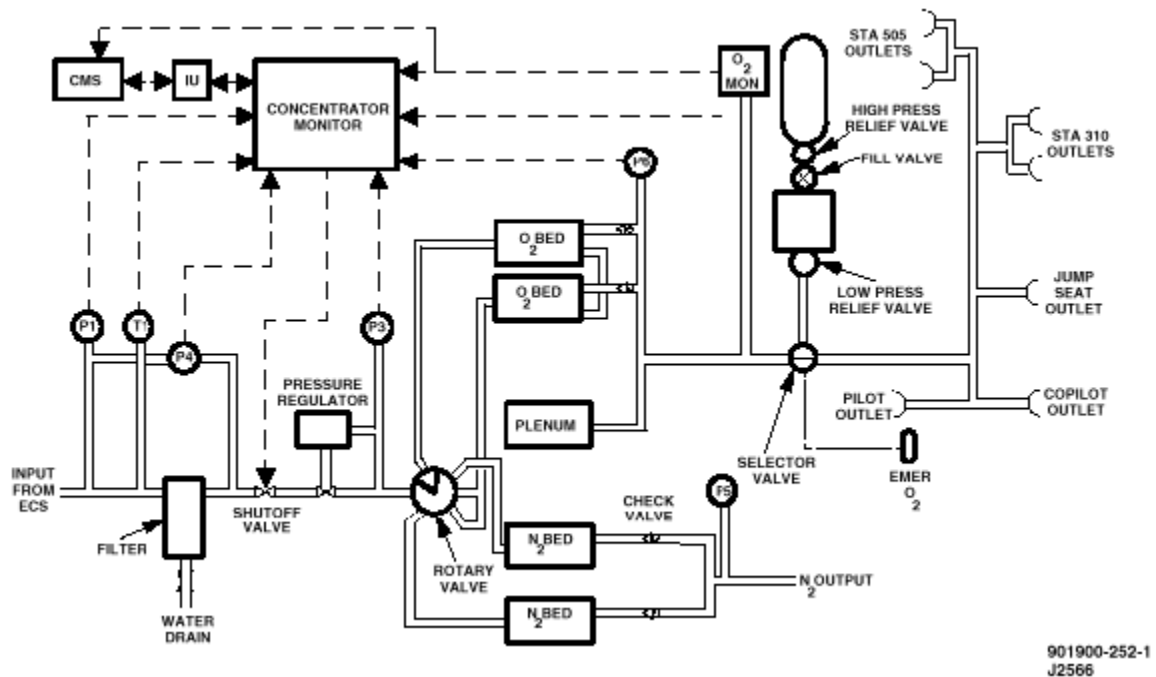
Figure 34. V-22 OBIGGS/OBOGS Schematic
