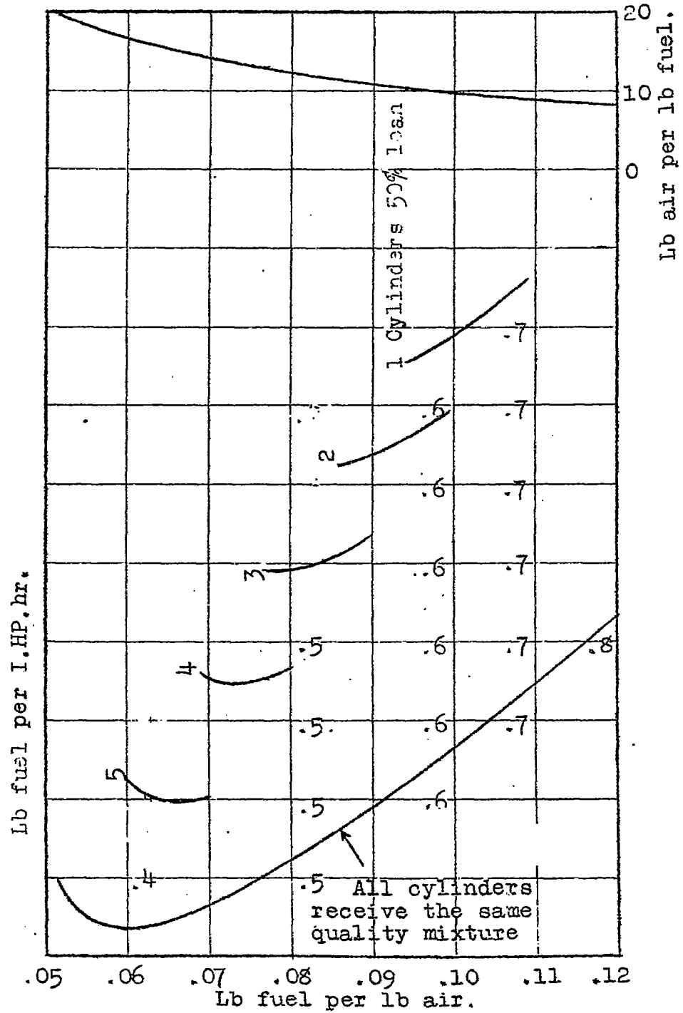
Fig.7. Effect of changes in distribution - 6 cylinder engine.
