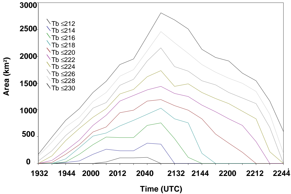
Figure 10. Time history of GOES-8 IR4 brightness temperatures ( T_b ) for the 16 July, 2002 case study. the contours represent the area (km 2 ) of a given T_b threshold at 2 °K intervals in an isolated region associated with cell 2.
