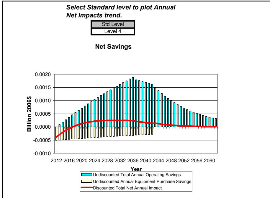
Figure G.7.5 National Annual Costs and Savings for Non-Standard Size PTHP, TSL 6
