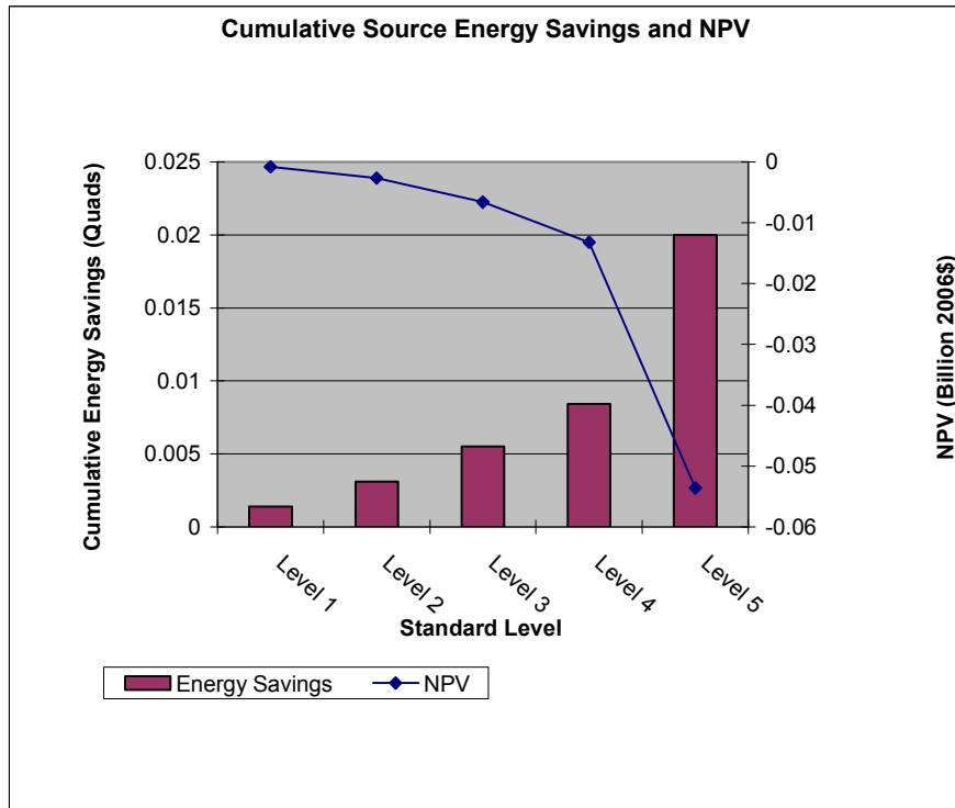
Figure G.3.1 Cumulative NPV Results for Standard Size PTAC, Cooling Capacity > 10,000 Btu/h, 7-Percent Discount Rate (Billion 2006$)
