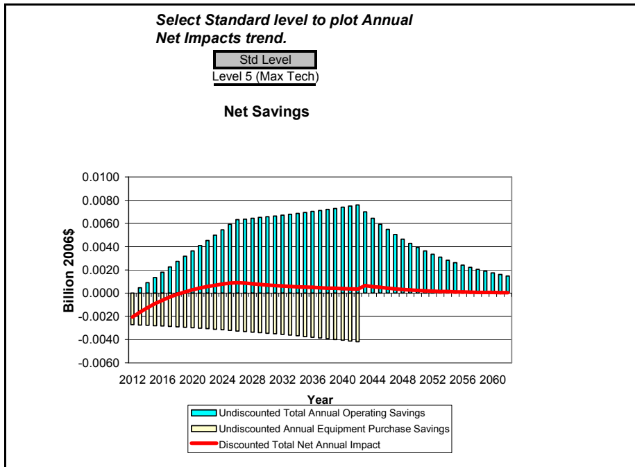
Figure G.4.6 National Annual Costs and Savings for Standard Size PTHP, Cooling Capacity \leq 10,000 Btu/h, TSL 7
