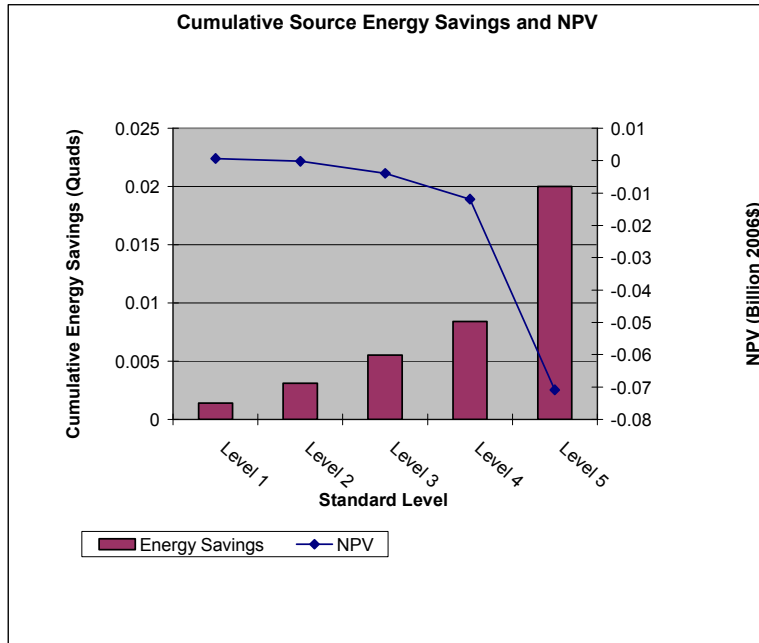
Figure G.3.7 Cumulative NPV Results for Standard Size PTAC, Cooling Capacity > 10,000 Btu/h, 3-Percent Discount Rate (Billion 2006$)
