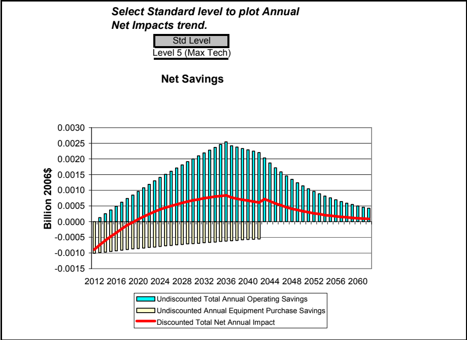
Figure G.2.12 National Annual Costs and Savings for Standard Size PTAC, Cooling Capacity ≤ 10,000 Btu/h, TSL 7
