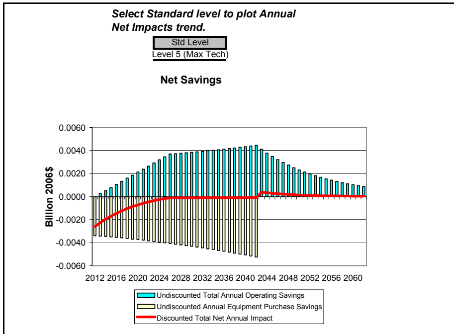
Figure G.2.6 National Annual Costs and Savings for Standard Size PTAC, Cooling Capacity of \leq 10,000 Btu/h, TSL 7
