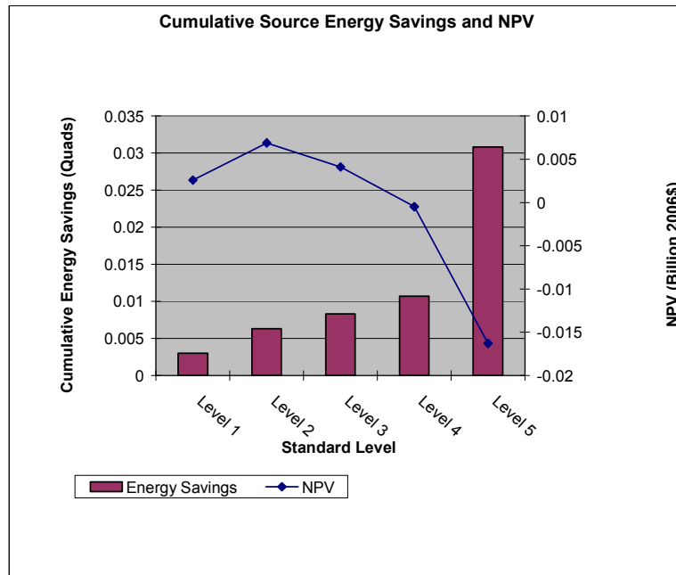
Figure G.5.1 Cumulative NPV Results for Standard Size PTHP, Cooling Capacity > 10,000 Btu/h, 7-Percent Discount Rate (Billion 2006$)
