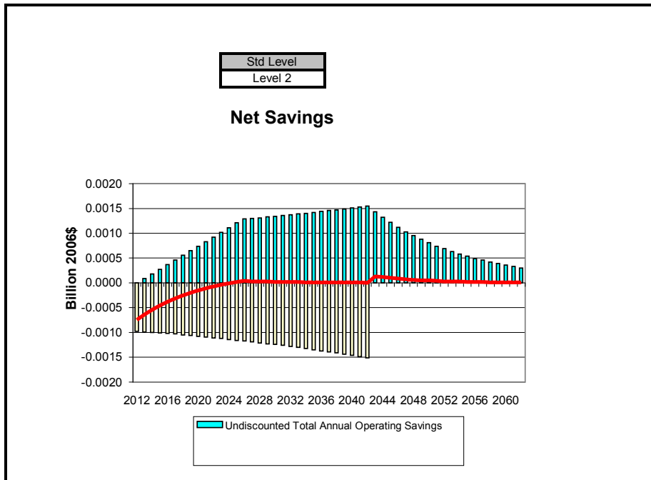
Figure G.3.3 National Annual Costs and Savings for Standard Size PTAC, Cooling Capacity > 10,000 Btu/h, TSL 3
