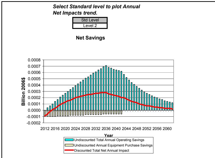
Figure G.7.9 National Annual Costs and Savings for Non-Standard Size PTHP, TSL 2 and TSL 3
