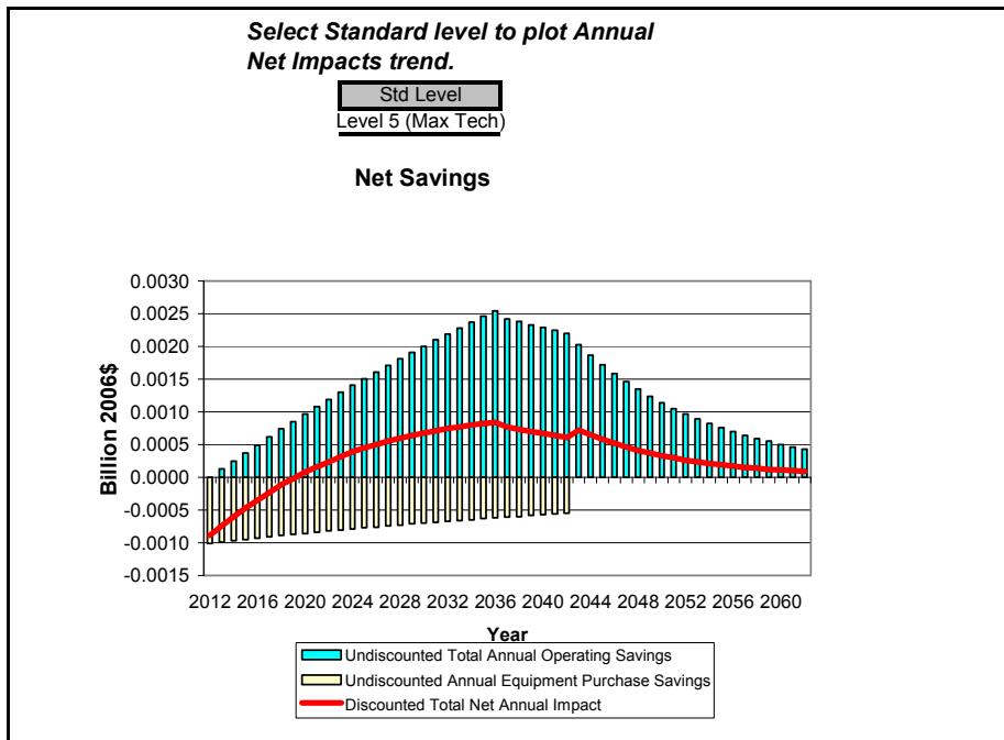
Figure G.7.12 National Annual Costs and Savings for Non-Standard Size PTHP, TSL 7
