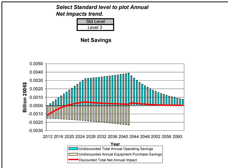
Figure G.5.4 National Annual Costs and Savings for Standard Size PTHP, Cooling Capacity > 10,000 Btu/h, TSL 4 and TSL 5
