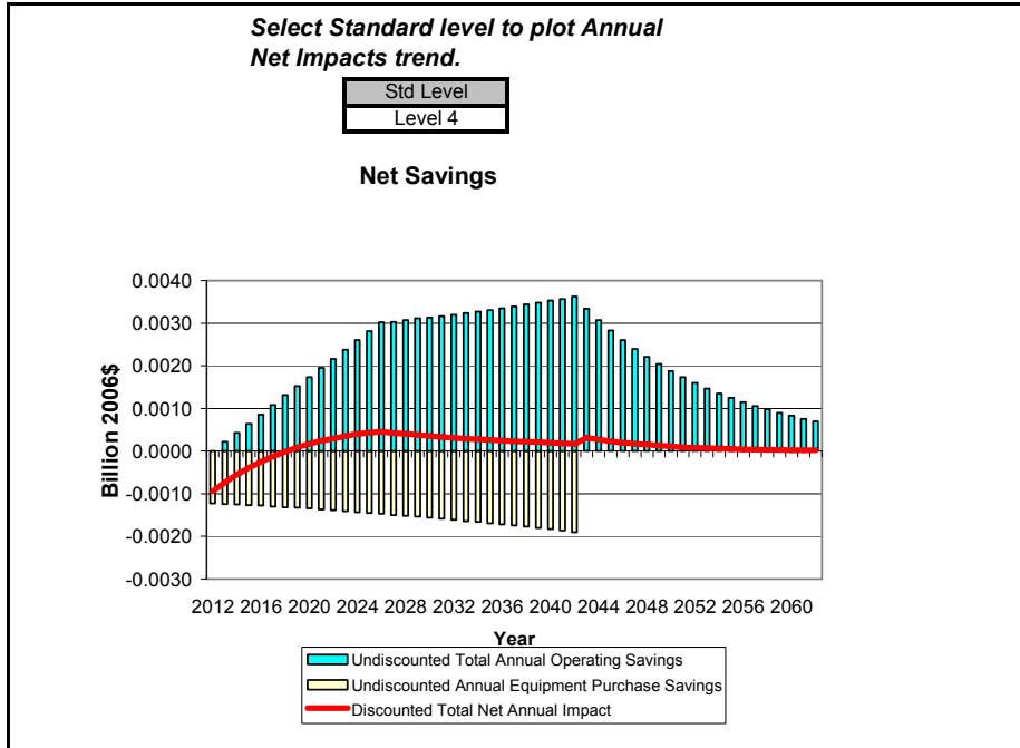
Figure G.4.5 National Annual Costs and Savings for Standard Size PTHP, Cooling Capacity \leq 10,000 Btu/h, TSL 6
