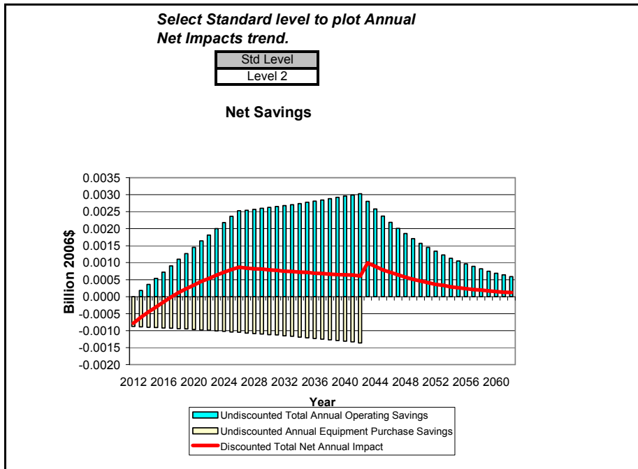
Figure G.5.9 National Annual Costs and Savings for Standard Size PTHP, Cooling Capacity > 10,000 Btu/h, TSL 2 and TSL 3
