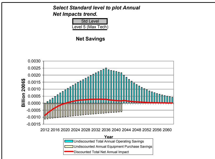
Figure G.6.6 National Annual Costs and Savings for Non-Standard Size PTAC, TSL 7
