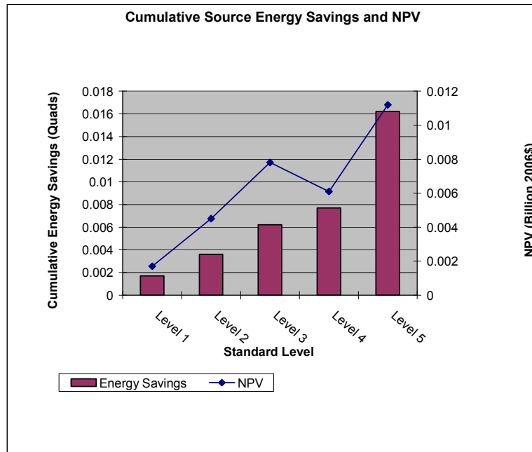
Figure G.4.1 Cumulative NPV Results for Standard Size PTHP, Cooling Capacity \leq 10,000 Btu/h, 7-Percent Discount Rate (Billion 2006$)
