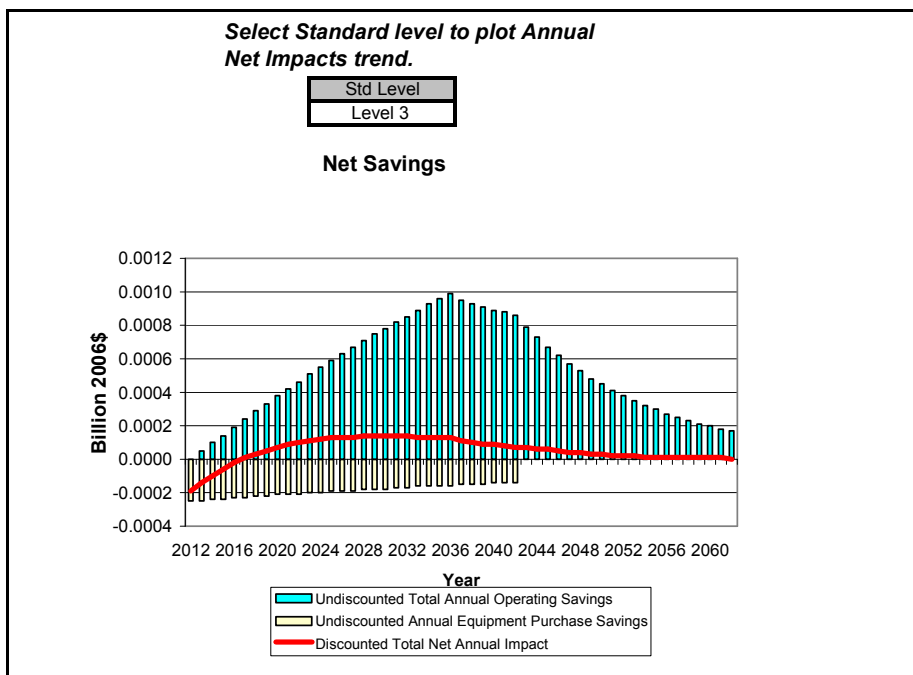
Figure G.6.4 National Annual Costs and Savings for Non-Standard Size PTAC, TSL 5
