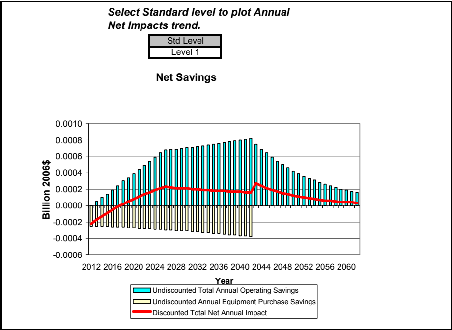
Figure G.4.8 National Annual Costs and Savings for Standard Size PTHP, Cooling Capacity \leq 10,000 Btu/h, TSL 1
