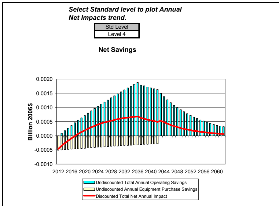
Figure G.2.11 National Annual Costs and Savings for Standard Size PTAC, Cooling Capacity \leq 10,000 Btu/h, TSL 6
