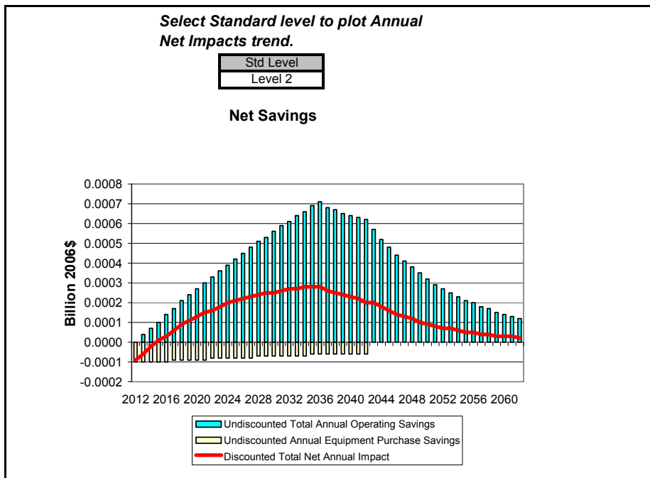
Figure G.2.9 National Annual Costs and Savings for Standard Size PTAC, Cooling Capacity \leq 10,000 Btu/h, TSL 3
