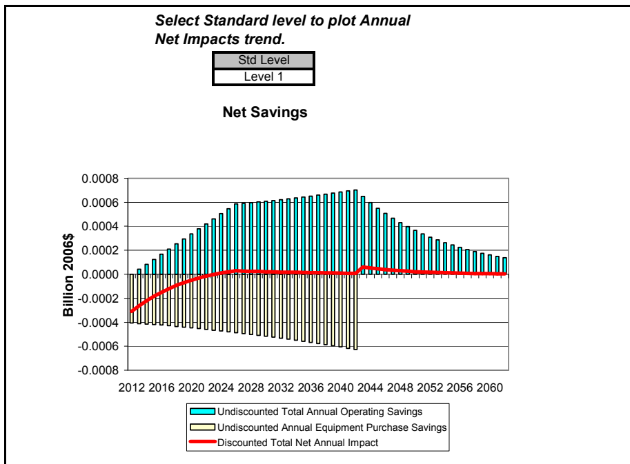
Figure G.3.2 National Annual Costs and Savings for Standard Size PTAC, Cooling Capacity > 10,000 Btu/h, TSL 1, TSL 2 and TSL 4
