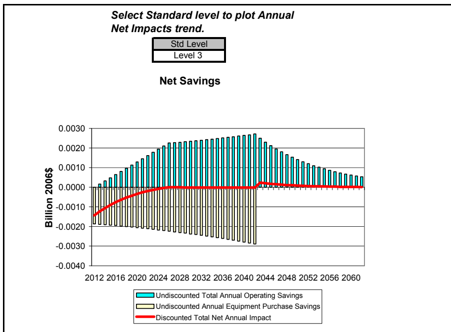
Figure G.3.4 National Annual Costs and Savings for Standard Size PTAC, Cooling Capacity > 10,000 Btu/h, TSL 5
