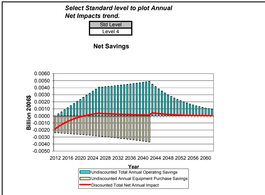
Figure G.5.5 National Annual Costs and Savings for Standard Size PTHP, Cooling Capacity > 10,000 Btu/h, TSL 6
