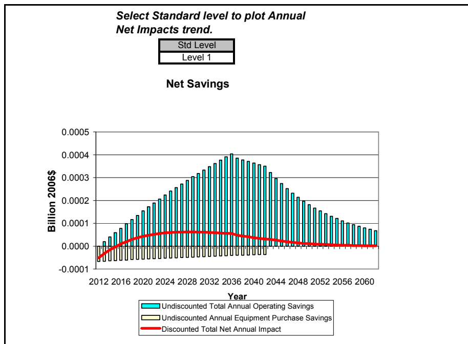
Figure G.6.2 National Annual Costs and Savings for Non-Standard Size PTAC, TSL 1, TSL 2 and TSL 4
