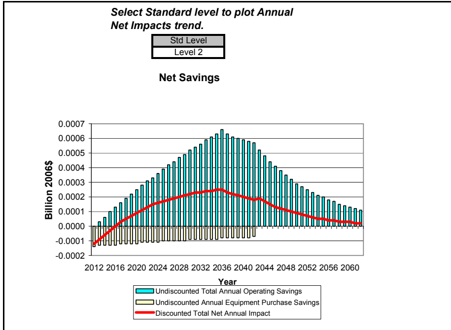
Figure G.6.9 National Annual Costs and Savings for Non-Standard Size PTAC, TSL 3
