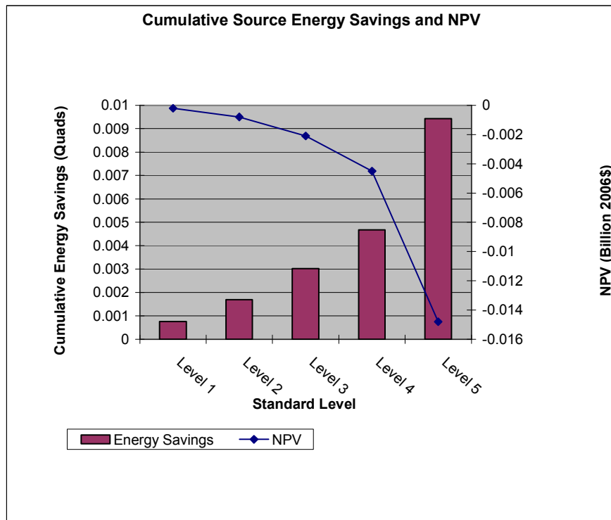
Figure G.2.1 Cumulative NPV Results for Standard Size PTAC, Cooling Capacity \leq 10,000 Btu/h, 7-Percent Discount Rate (Billion 2006$)
