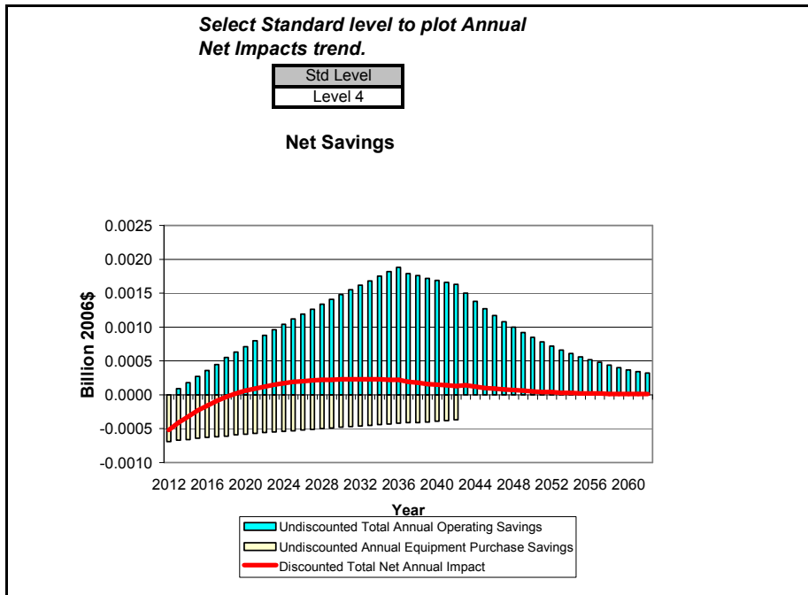
Figure G.6.5 National Annual Costs and Savings for Non-Standard Size PTAC, TSL 6
