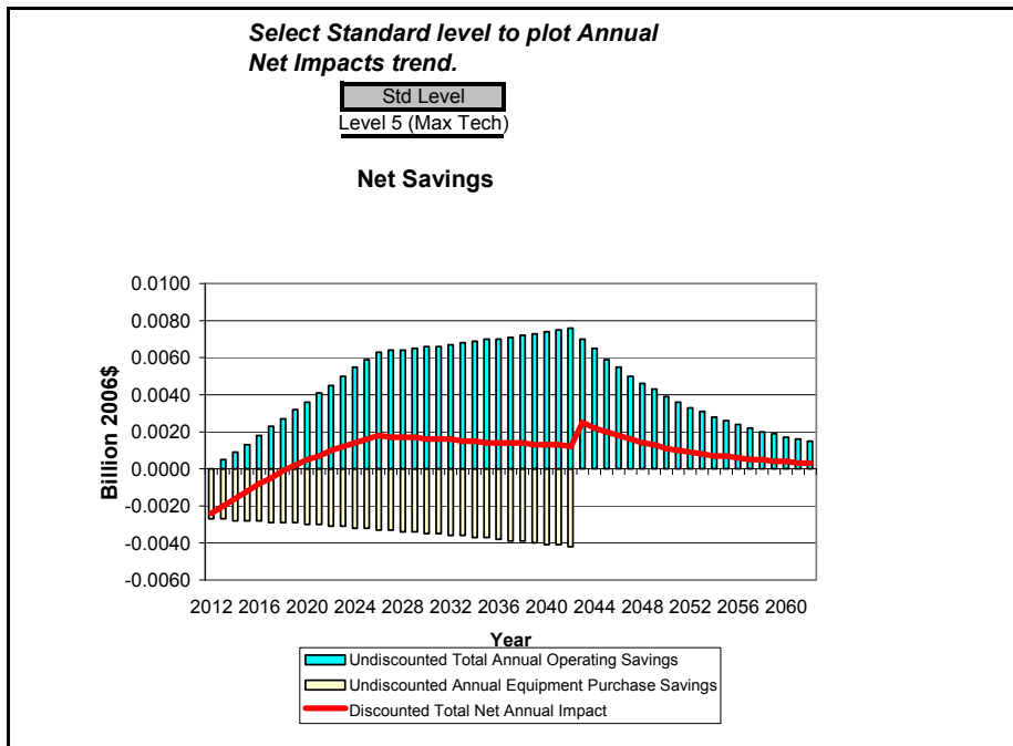
Figure G.4.12 National Annual Costs and Savings for Standard Size PTHP, Cooling Capacity \leq 10,000 Btu/h, TSL 7
