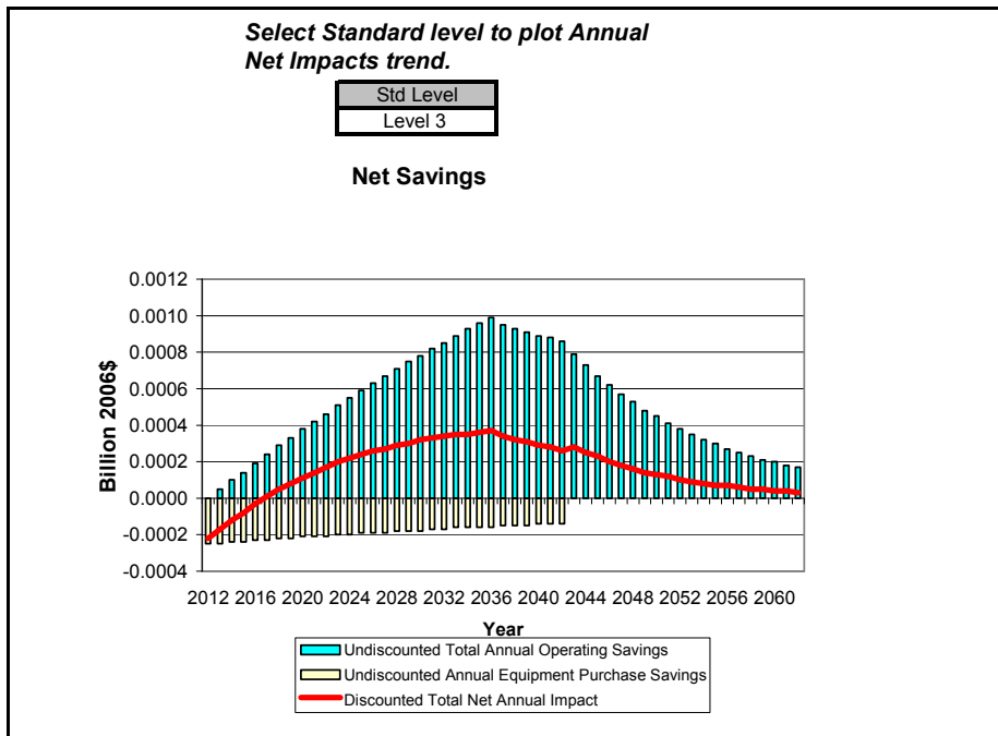
Figure G.6.10 National Annual Costs and Savings for Non-Standard Size PTAC, TSL 5
