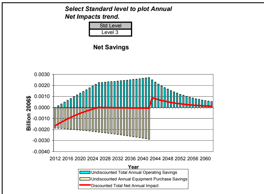
Figure G.3.10 National Annual Costs and Savings for Standard Size PTAC, Cooling Capacity > 10,000 Btu/h, TSL 5
