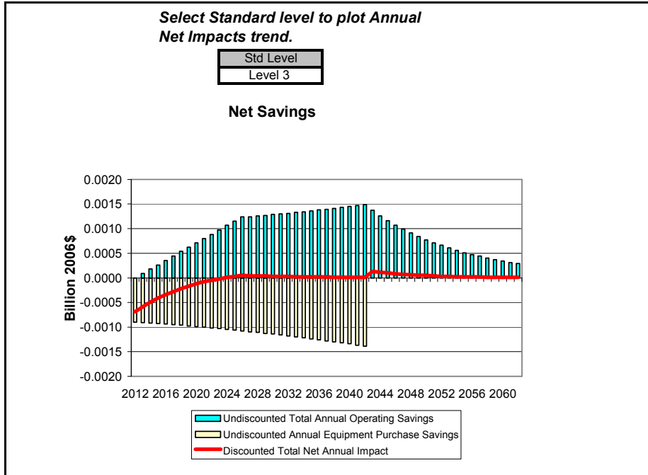
Figure G.2.4 National Annual Costs and Savings for Standard Size PTAC, Cooling Capacity \leq 10,000 Btu/h , TSL 5
