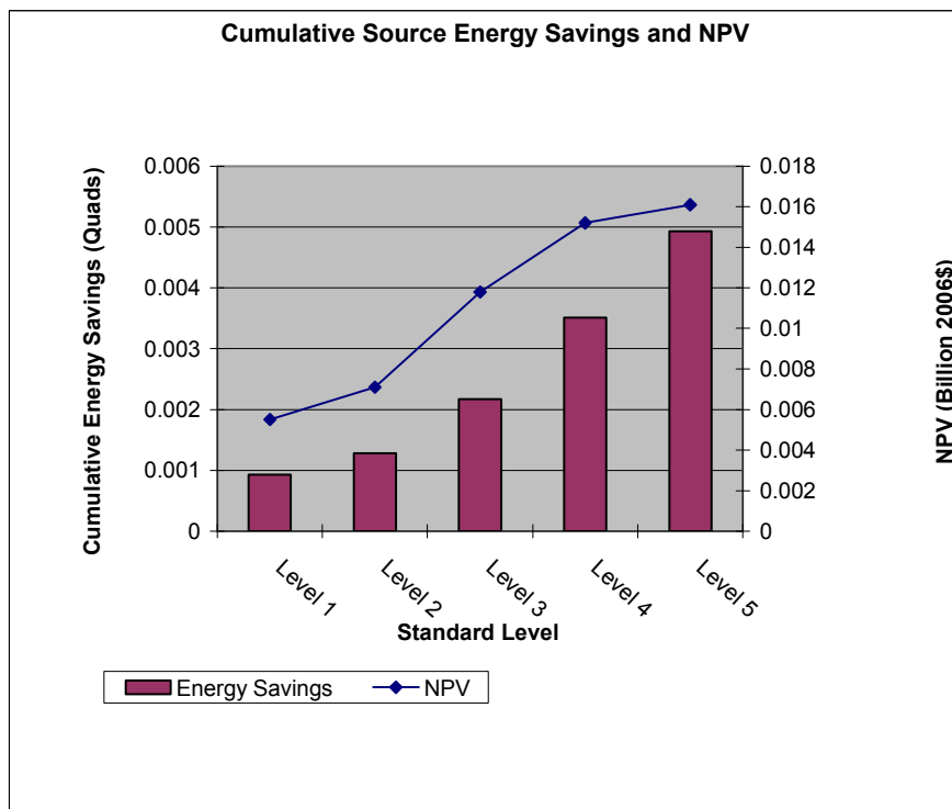
Figure G.2.7 Cumulative NPV Results for Standard Size PTAC, Cooling Capacity \leq 10,000 Btu/h, 3-Percent Discount Rate (Billion 2006$)
