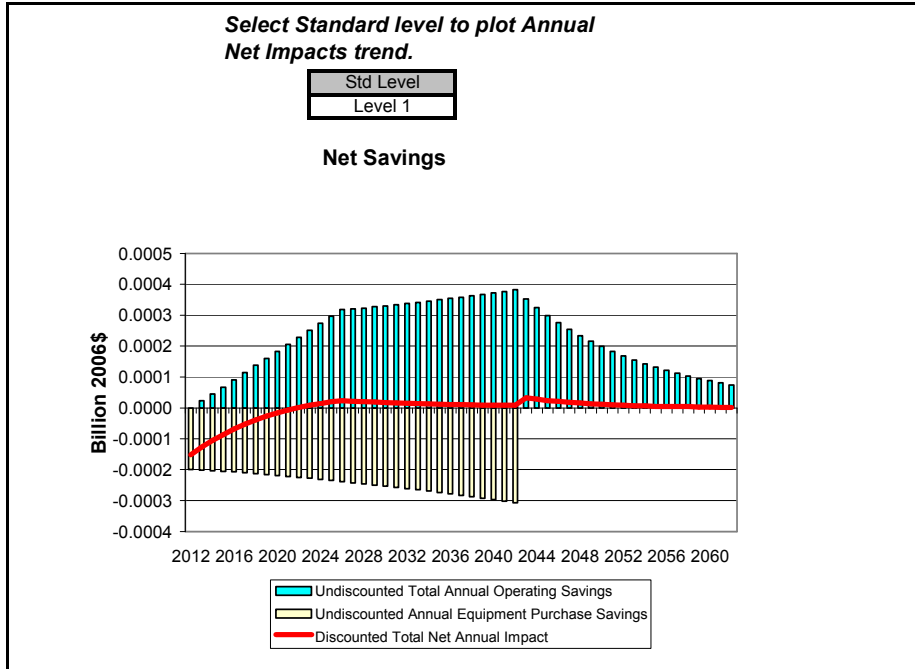
Figure G.2.2 National Annual Costs and Savings for Standard Size PTAC, Cooling Capacity \leq 10,000 Btu/h, TSL 1, TSL 2 and TSL 4
