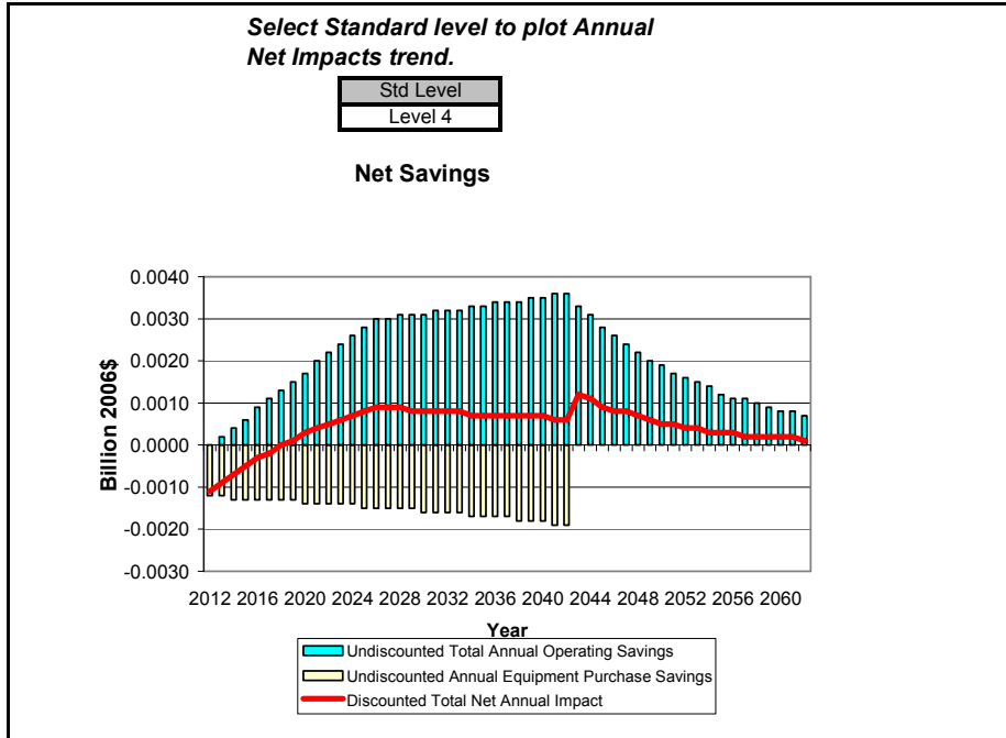
Figure G.4.11 National Annual Costs and Savings for Standard Size PTHP, Cooling Capacity \leq 10,000 Btu/h, TSL 6
