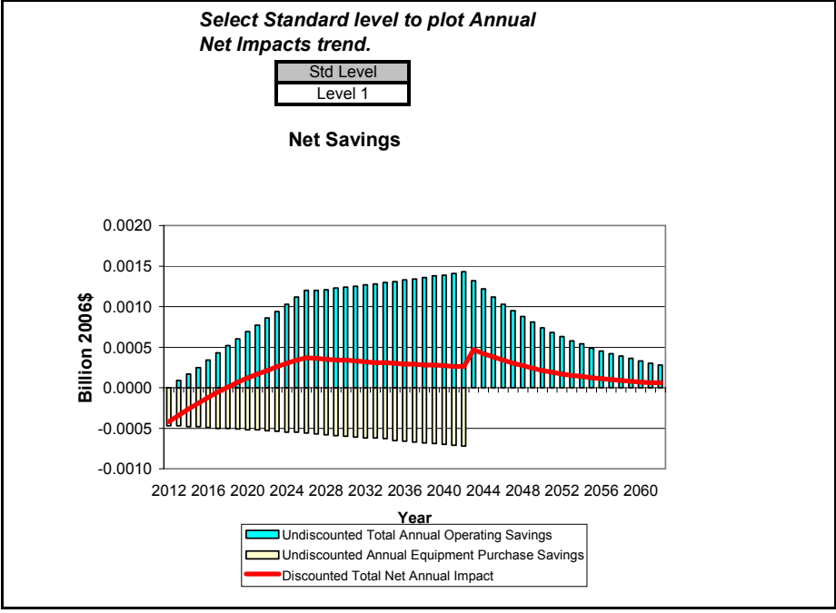
Figure G.5.8 National Annual Costs and Savings for Standard Size PTHP, Cooling Capacity > 10,000 Btu/h, TSL 1
