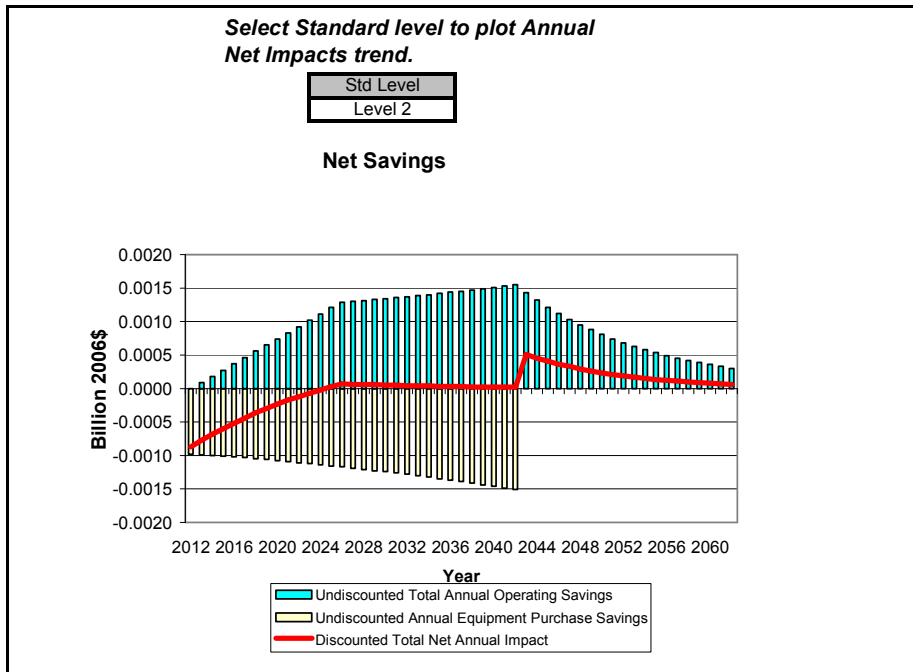
Figure G.3.9 National Annual Costs and Savings for Standard Size PTAC, Cooling Capacity > 10,000 Btu/h, TSL 3
