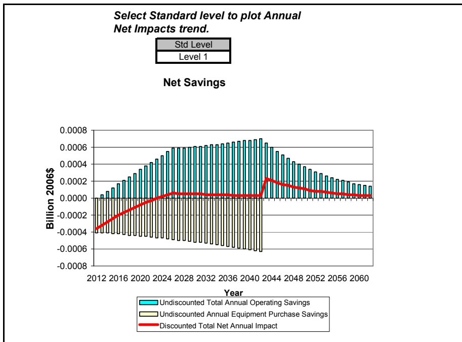
Figure G.3.8 National Annual Costs and Savings for Standard Size PTAC, Cooling Capacity > 10,000 Btu/h, TSL 1, TSL 2 and TSL 4
