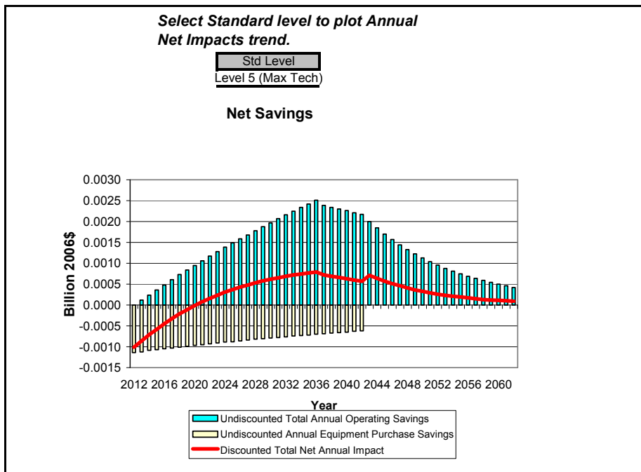
Figure G.6.12 National Annual Costs and Savings for Non-Standard Size PTAC, TSL 7
