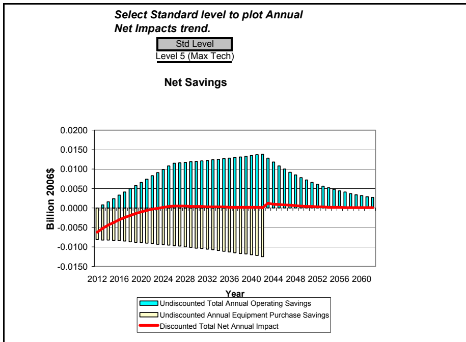
Figure G.5.6 National Annual Costs and Savings for Standard Size PTHP, Cooling Capacity > 10,000 Btu/h, TSL 7
