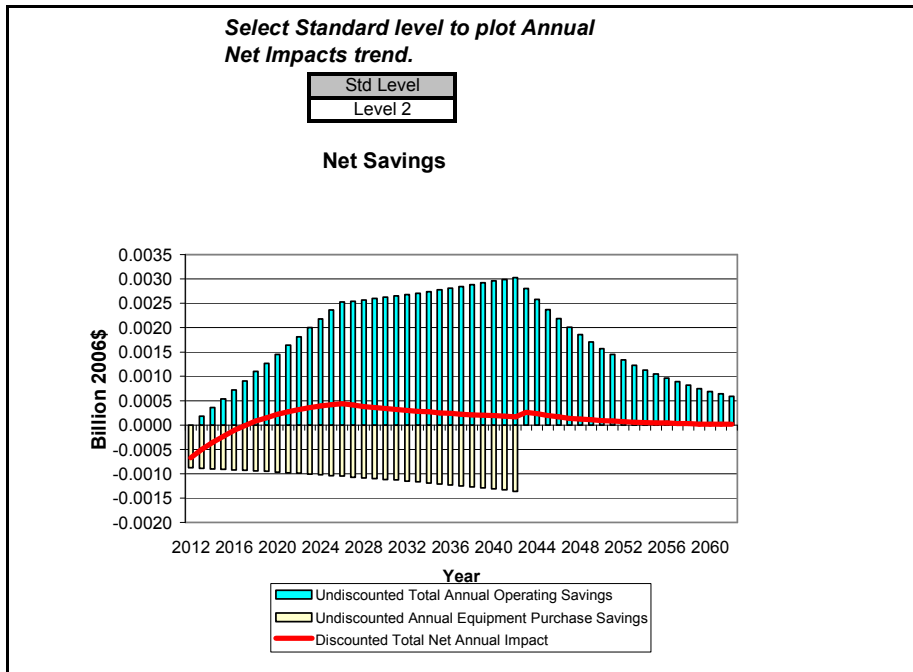
Figure G.5.3 National Annual Costs and Savings for Standard Size PTHP, Cooling Capacity > 10,000 Btu/h, TSL 2 and TSL 3
