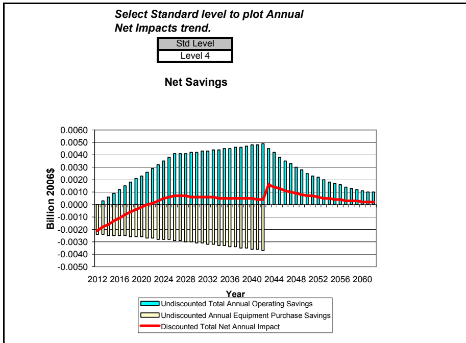
Figure G.5.11 National Annual Costs and Savings for Standard Size PTHP, Cooling Capacity > 10,000 Btu/h, TSL 6
