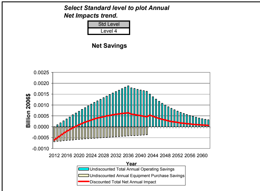
Figure G.6.11 National Annual Costs and Savings for Non-Standard Size PTAC, TSL 6
