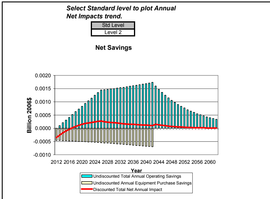
Figure G.4.3 National Annual Costs and Savings for Standard Size PTHP, Cooling Capacity \leq 10,000 Btu/h, TSL 2 and TSL 3
