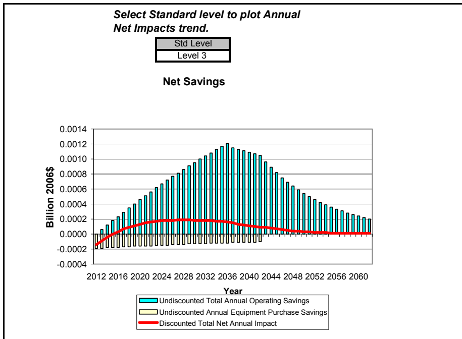
Figure G.7.4 National Annual Costs and Savings for Non-Standard Size PTHP, TSL 4 and TSL 5
