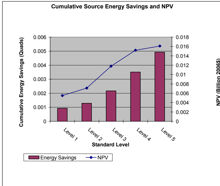
Figure G.7.7 Cumulative NPV Results for Non-Standard Size PTHP, 3-Percent Discount Rate (Billion 2006$)
