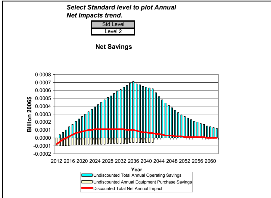
Figure G.7.3 National Annual Costs and Savings for Non-Standard Size PTHP, TSL 2 and TSL 3
