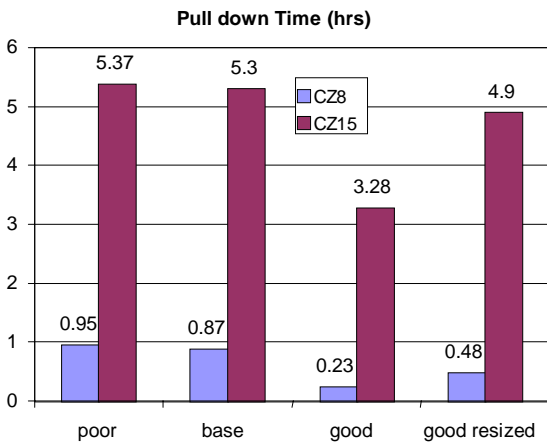
Figure 5. Climate and system dependence of the time required to cool a house (pull-down time)
