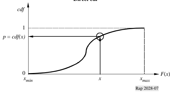
FIGURE 7 Direct cdf
