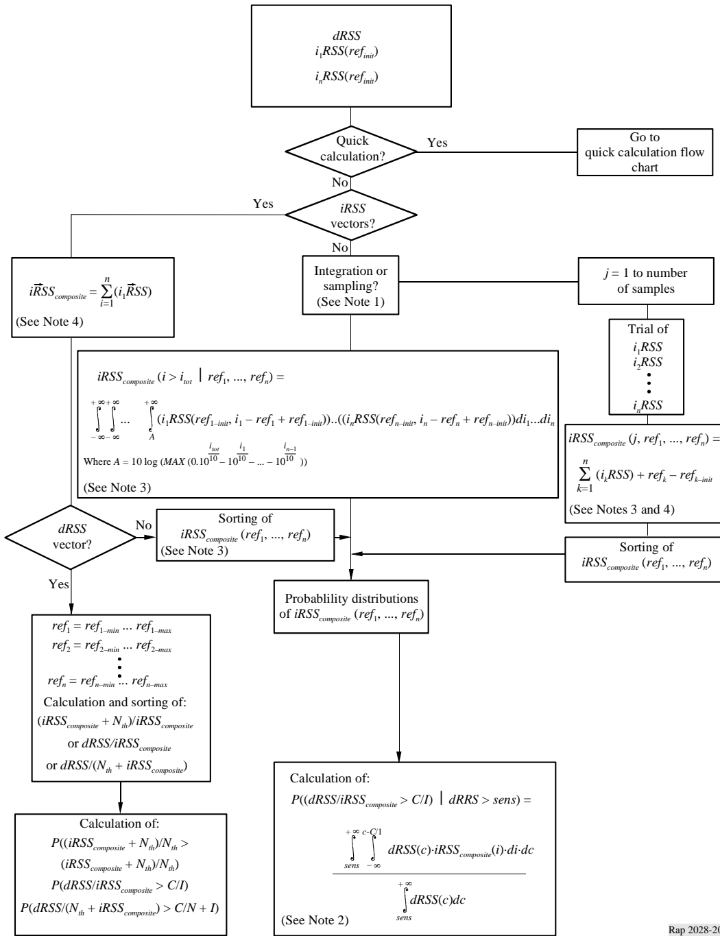
FIGURE 20 ICE flow chart
