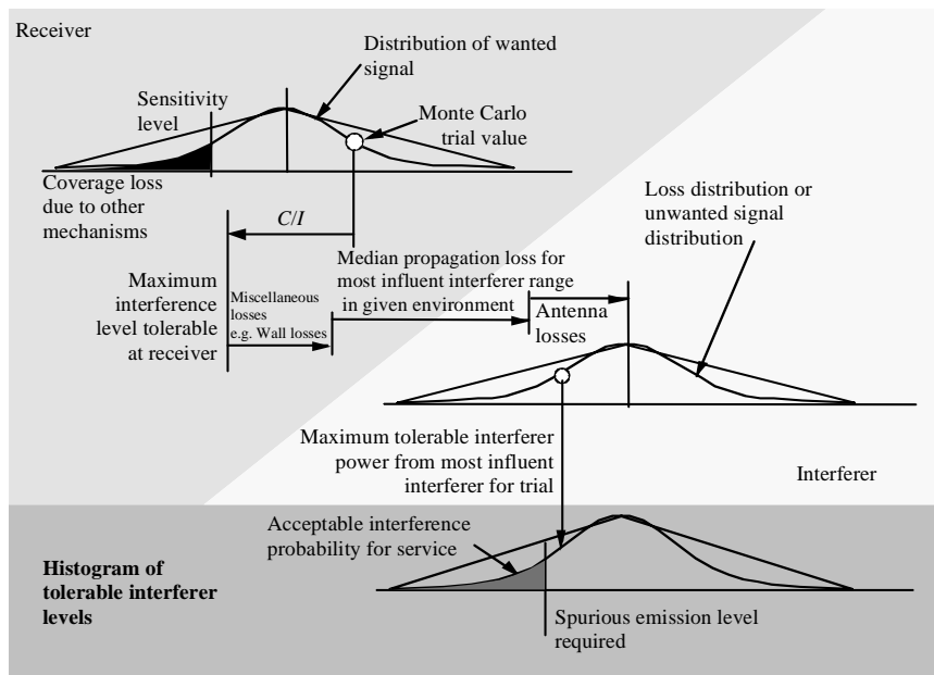
FIGURE 2 An example formulation of the Monte Carlo evaluation process
