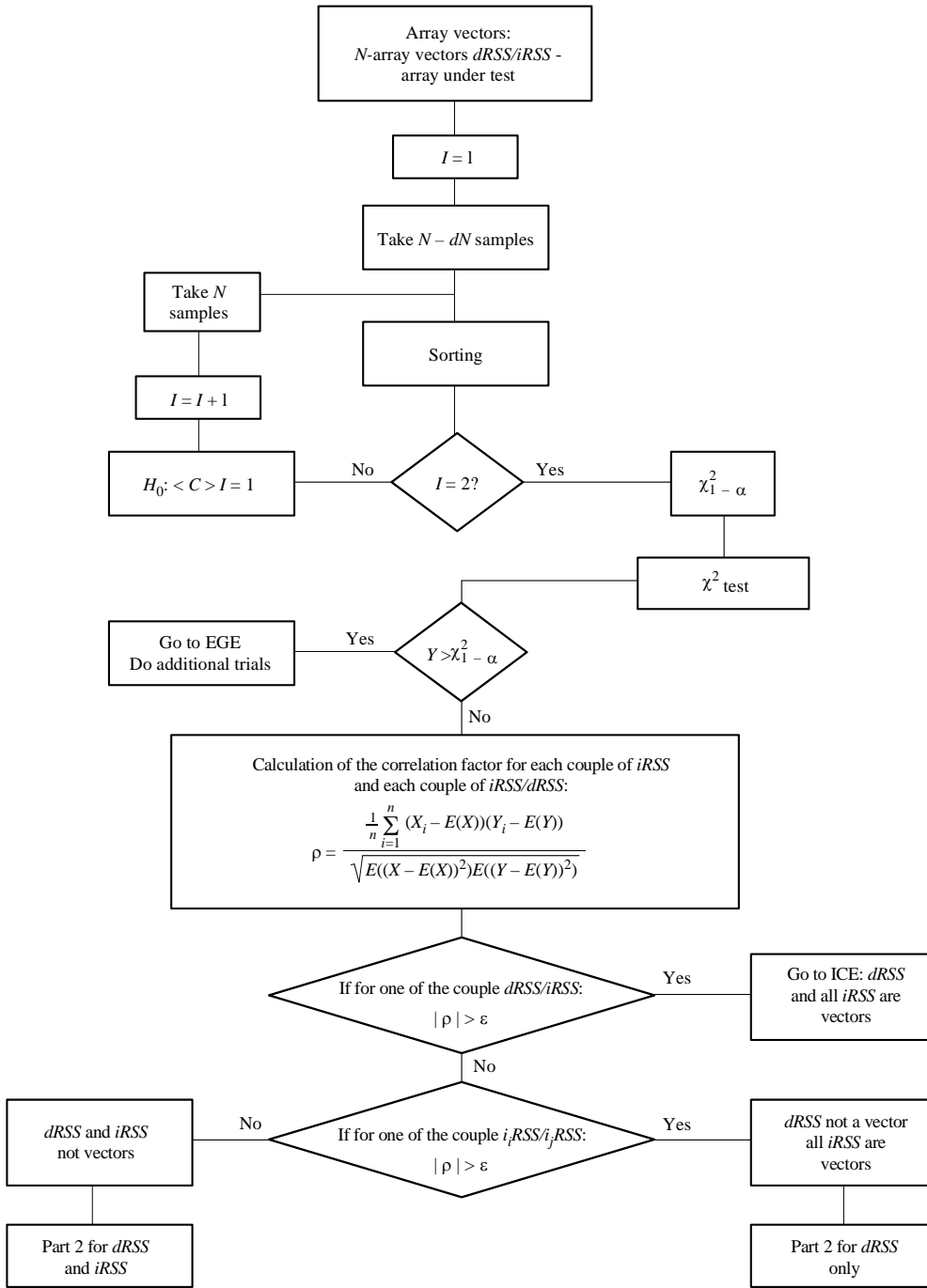
FIGURE 17 DEE flow chart
