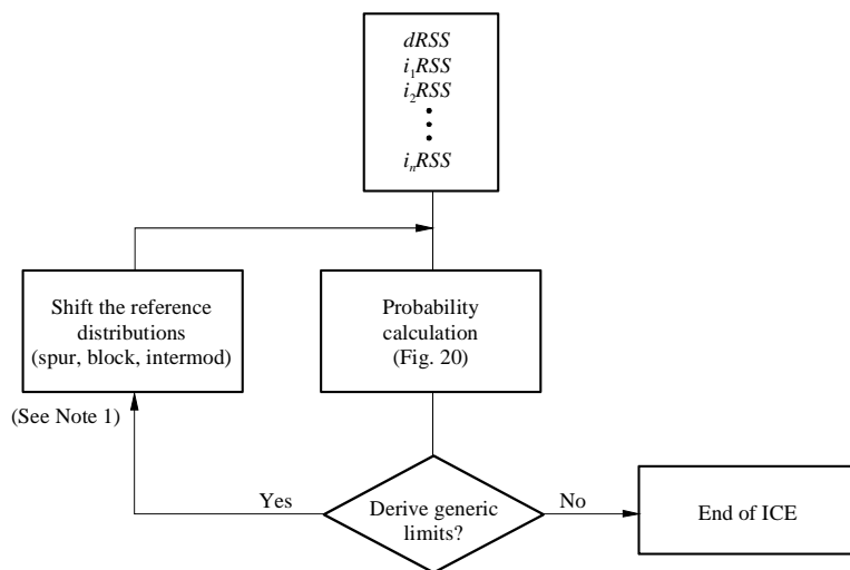
FIGURE 19 General ICE flow chart
