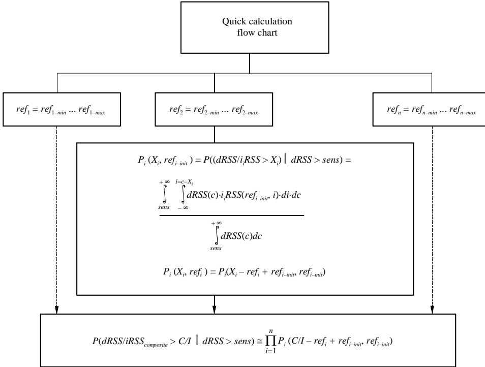
FIGURE 21 ICE quick calculation flow chart
