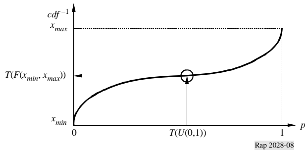
FIGURE 8 Inverse cdf
