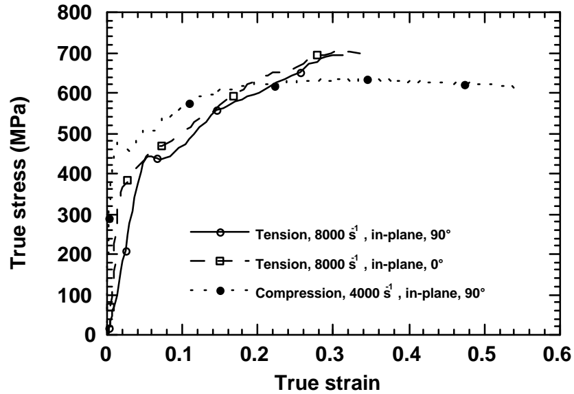
FIGURE 14. COMPARISON OF THE HIGH-STRAIN RATE, STRESS-STRAIN RESPONSE OF 2024-T3 ALLOY IN TENSION AND COMPRESSION
