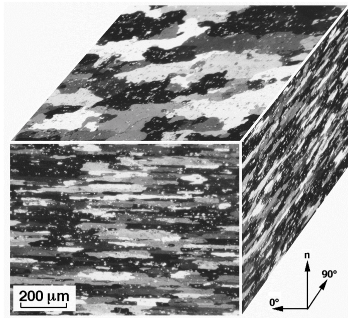
FIGURE 2. MICROSTRUCTURE OF 2024-T3 ALLOY
