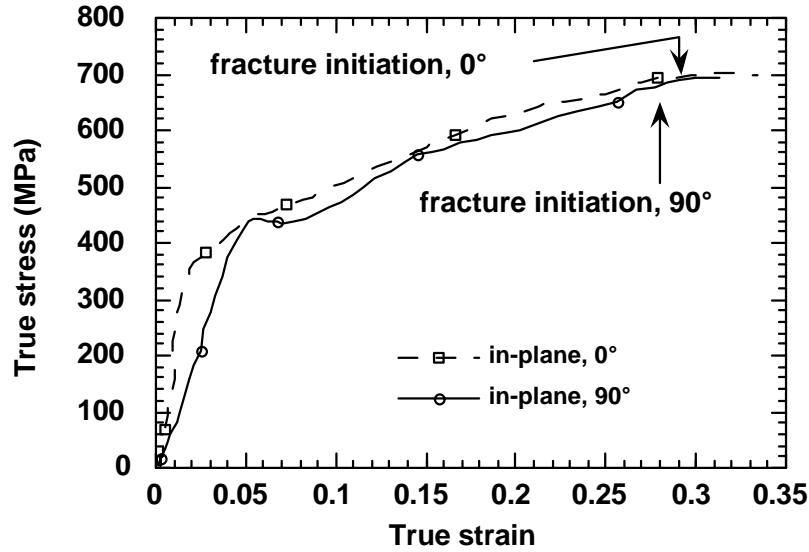
FIGURE 13. STRESS-STRAIN RESPONSE FOR 2024-T3 ALLOY TESTED IN TENSION AT A STRAIN RATE OF 8000 \text{ S}^{-1}
