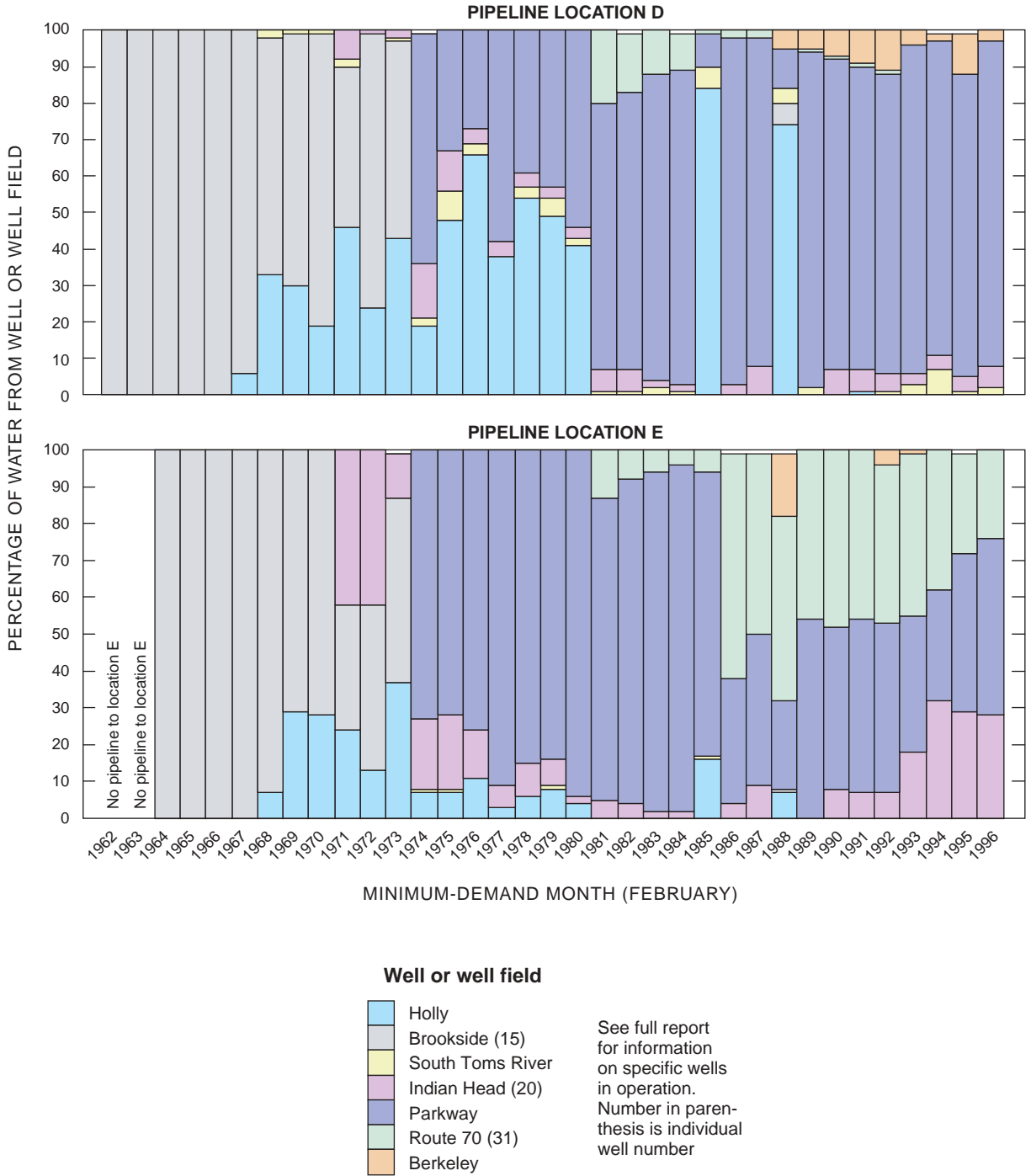
Figure 7. Annual variation of simulated proportionate contribution of water from wells and well fields to selected locations in the Dover Township area, New Jersey, minimum-demand months, 1962–96.
