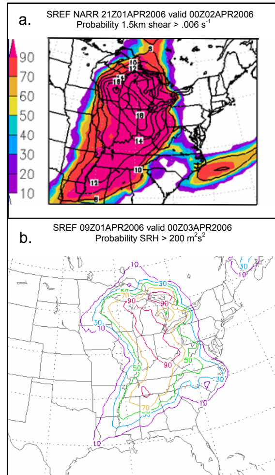
Figure 5. As in Figure 4 except showing a) Probability of 1.5 km mean shear > .006 s -1 (shaded) and mean shear magnitude > .006 s -1 and b) Probability of SRH > 200 m 2 s -2 .
