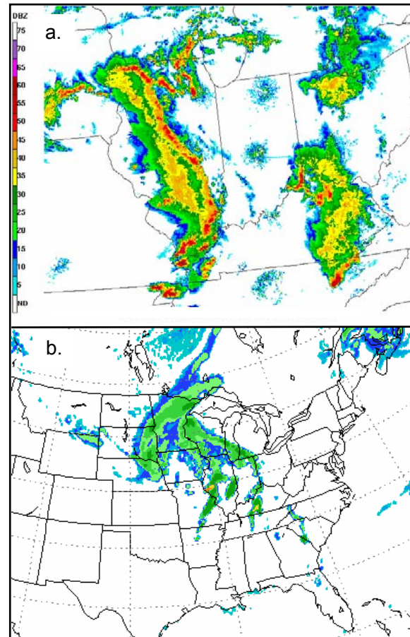
Figure 9. a) Real-time WSR-88D 0.5° Base Reflectivity and b) lowest model level Simulated Radar Reflectivity (dBZ) from the operational NAM-WRF, valid 0000 UTC 3 April 2006.
