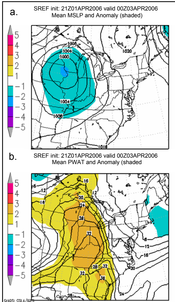
Figure 2. SREF forecasts initialized at 2100 UTC 1 April 2006 showing the 21-member ensemble mean of a) sea-level Pressure (hPa) and standardized climate anomaly (shaded, SD) and b) precipitable water (mm) and anomaly (shaded). MSLP and PWAT contours every 4 hPa and 4 mm respectively.
