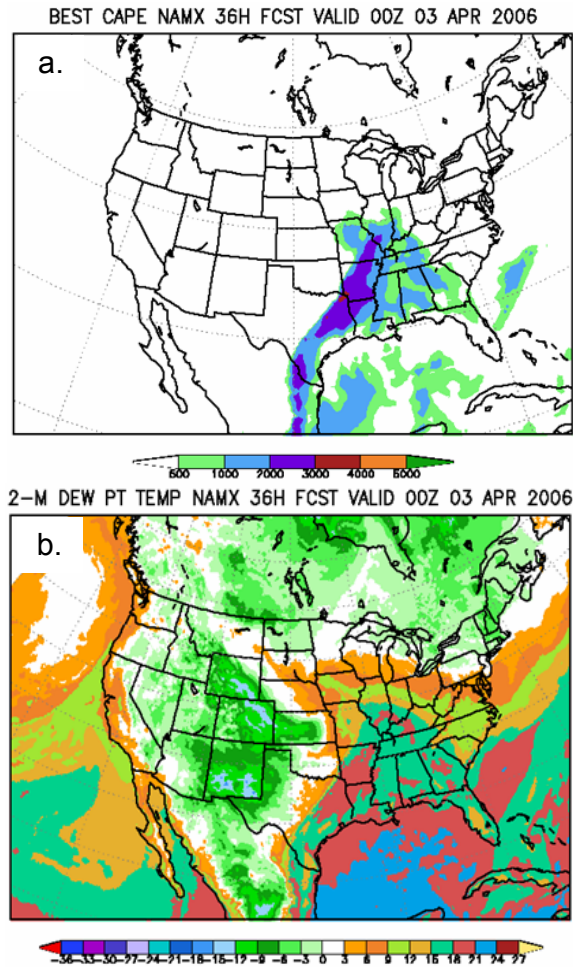
Figure 8. NAM-WRF 36 hr forecast of a) Best CAPE and b) 2 meter Dew Point temperatures, valid 0403/0000 UTC.
