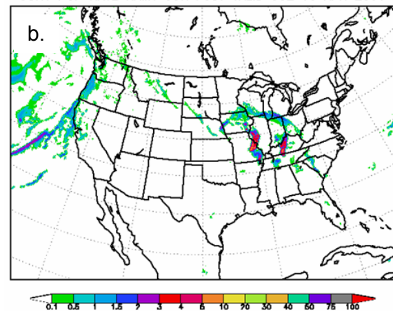
Figure 7. NAM-WRF 36 hr forecast of a) Instant PrecipitationRate and b) Convective precipitation rate, valid 0403/0000 UTC.
