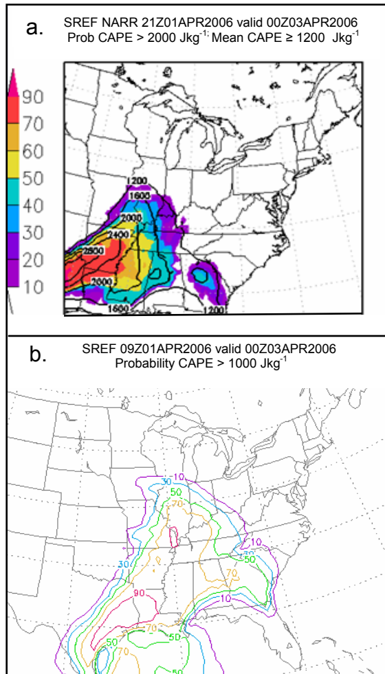
Figure 4. SREF forecasts initialized at (a) 2100 UTC and (b) 0900 UTC 1 April 2006 valid 0000 UTC 3 April 2006 showing the SREF of a) Probability of CAPE > 2000 Jkg -1 (shaded) and mean CAPE ≥ 1200 Jkg -1 and b) Probability of CAPE > 1000 Jkg -1 .
