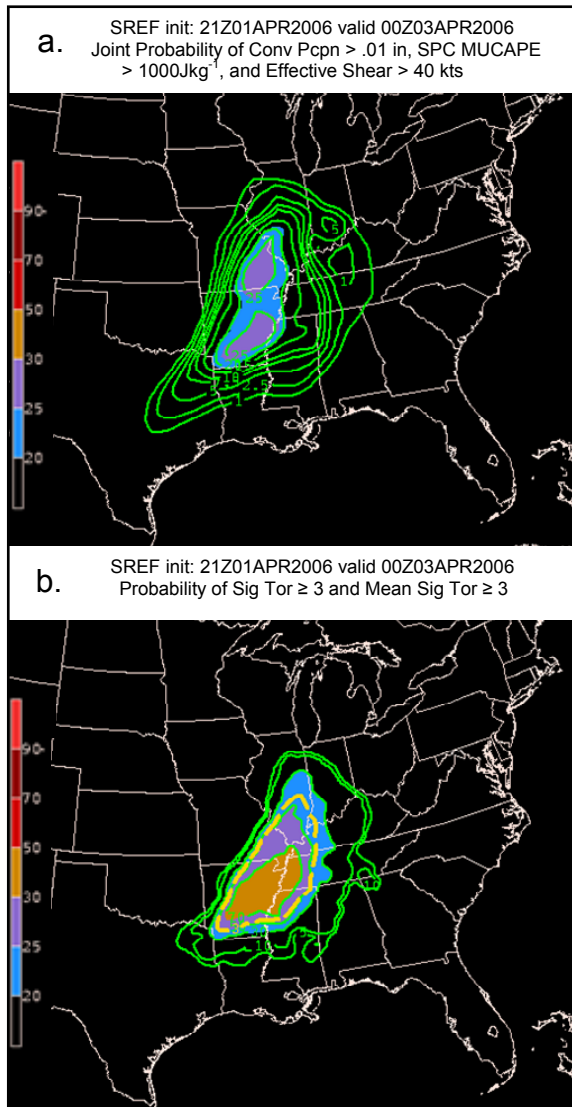
Figure 6. SREF forecasts initialized at 2100 UTC 1 April 2006 showing a) Joint Probability of 3 hr. Convective Precipitation > .01 in, SPC MUCAPE > 1000Jkg -1 , and Effective Shear > 40 kts and b) probability of Significant Tornado Parameter ≥ 3 (shaded) and Mean Significant Tornado Parameter ≥ 3 (yellow dash)
