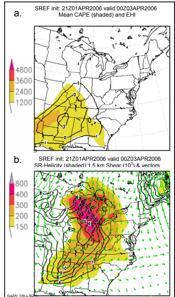
Figure 3. As in Figure 2 except showing a) mean CAPE (shaded, \text{Jkg}^{-1} ) and EHI and b) mean SR-Helicity (shaded, \text{m}^2\text{s}^{-2} ), 1.5km Shear magnitude ( \text{s}^{-1} \times 10^3 ), and 1.5 km Shear vectors.
