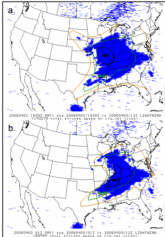
Figure 10. a) SPC Day 1 Convective Outlook valid a) 0402/1630 UTC and b) 0403/0100 UTC. Total lightning strikes a) 0402/1630 UTC – 0403/1200 and b) 0403/0100 UTC – 0403/1200 UTC.
