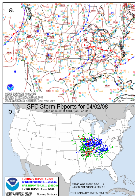
Figure 1. a) HPC surface analysis valid 0000 UTC 3 April 2006 and b) SPC Storm Reports for 2 April 2006
