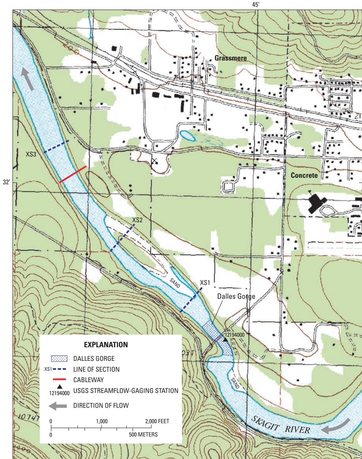
Figure 1. Location of cross sections, discharge measurement cableway, Dalles Gorge, and streamflow-gaging station Skagit River near Concrete, Washington.
