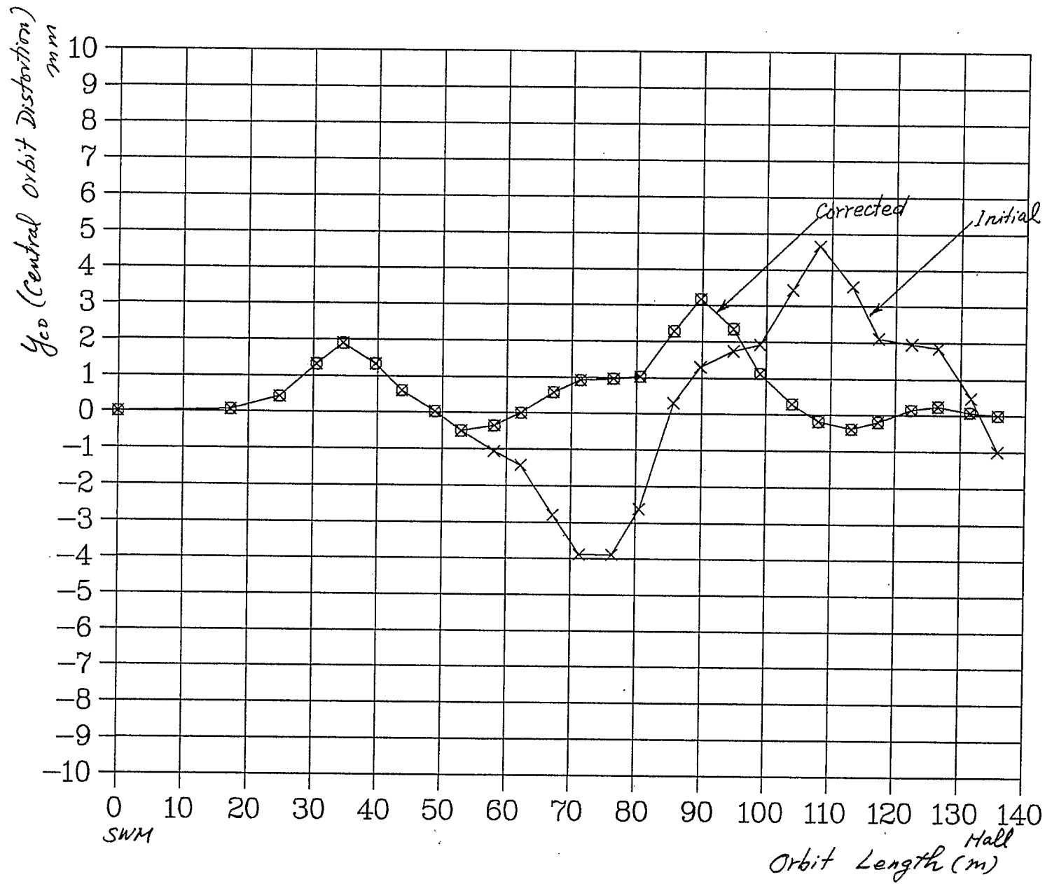
Figure 10. Initial and Corrected Orbit Distortion 30.10.60
