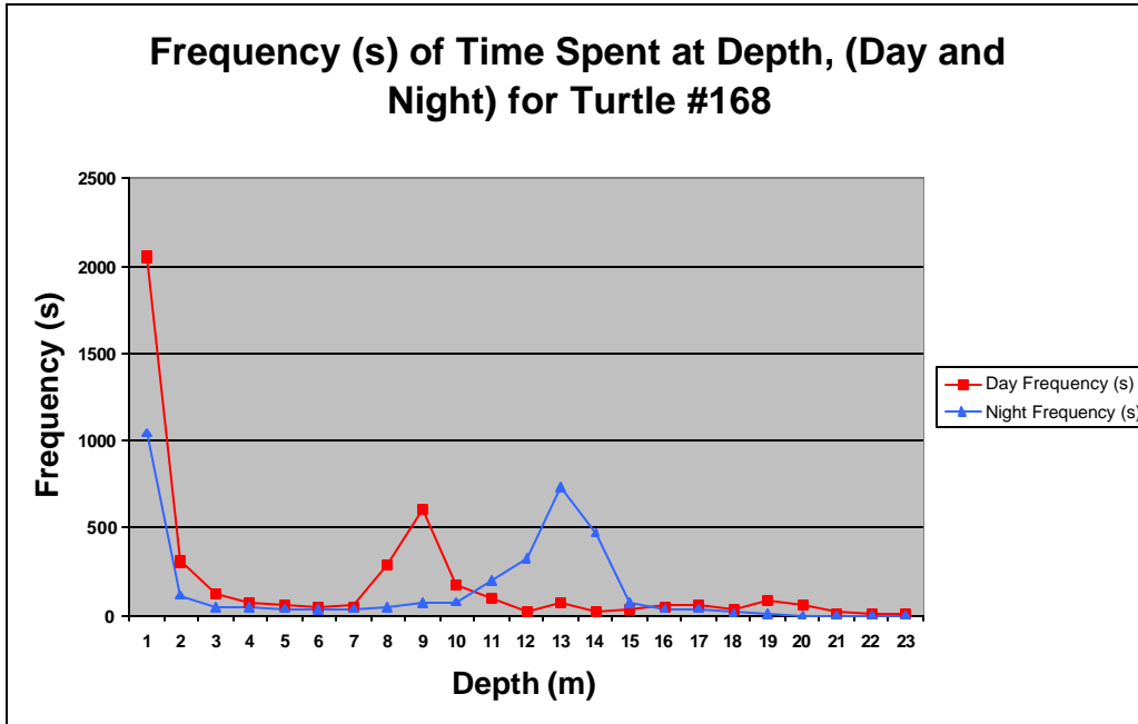
Figure 27. Frequency of time spent at different depths for turtle # 168, Day vs. Night.
