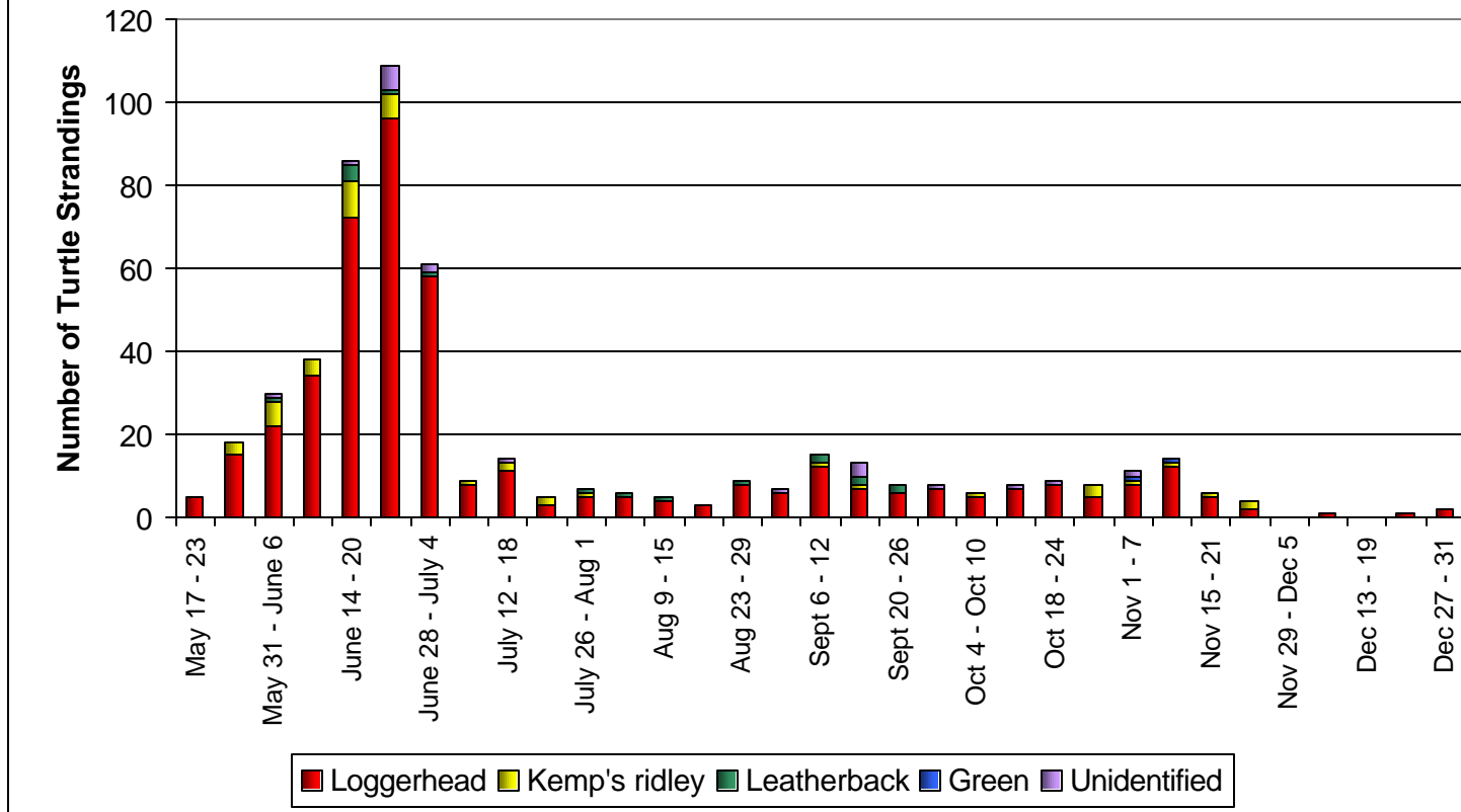
Figure 1. 2003 sea turtle strandings by week and species, May 17 through December 31 (n=526). Note: there were three strandings recorded in March that are not represented on this graph.
