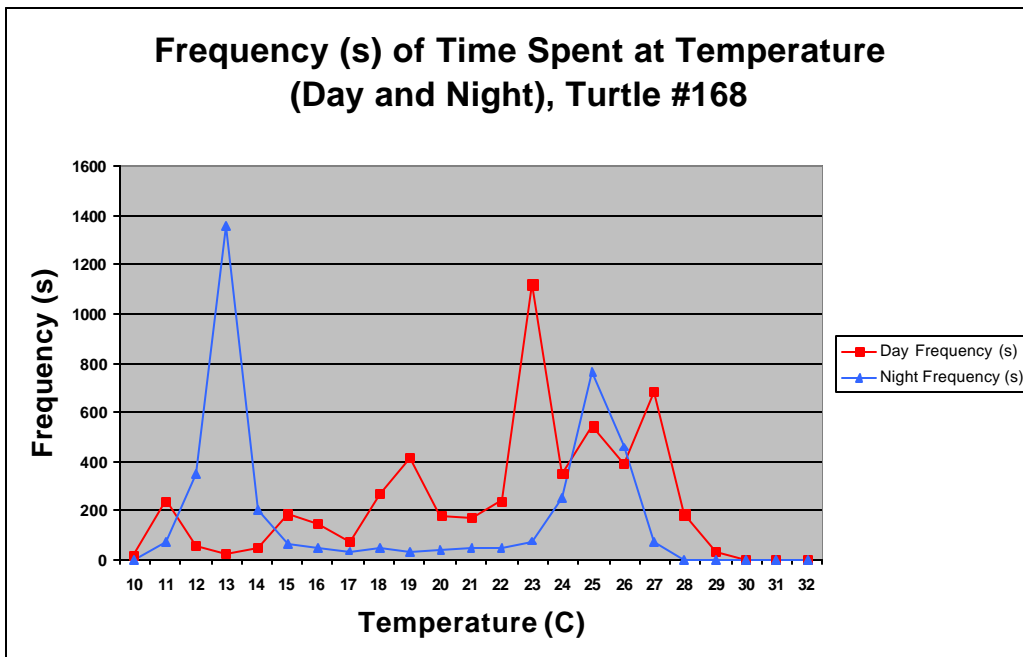
Figure 28. Frequency of time spent at different temperatures for turtle # 168, Day vs. Night.
