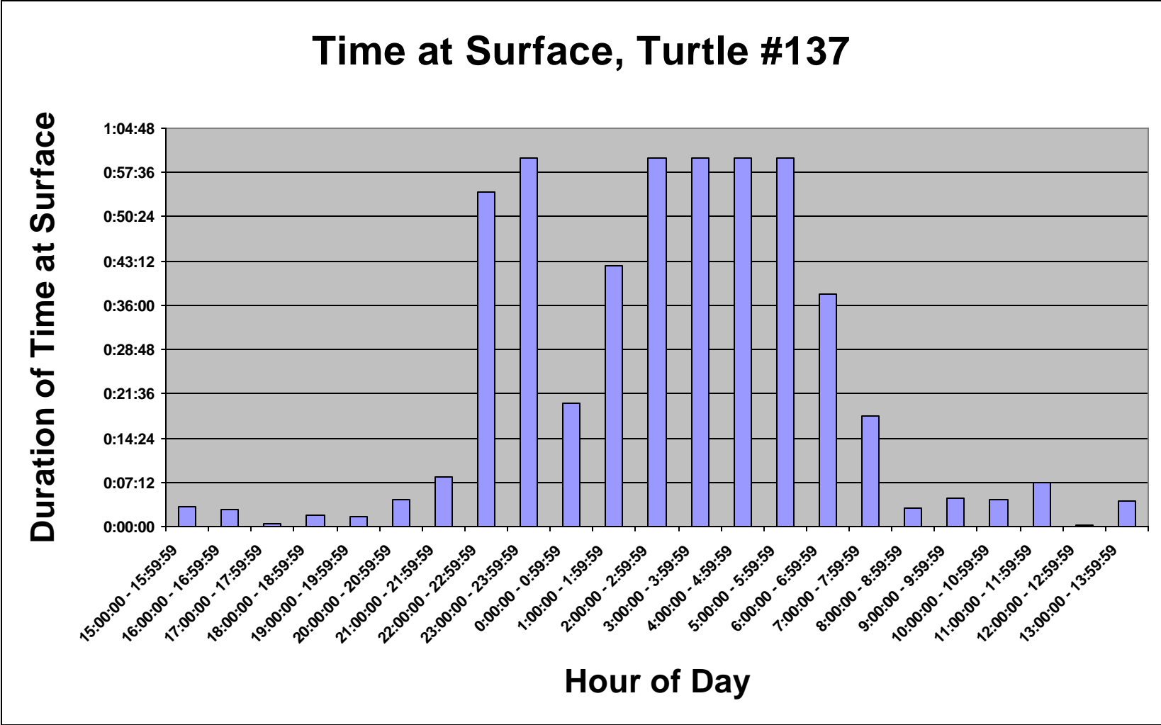
Figure 6. Turtle #137 Surfacing Times, July 15-16, 2003
