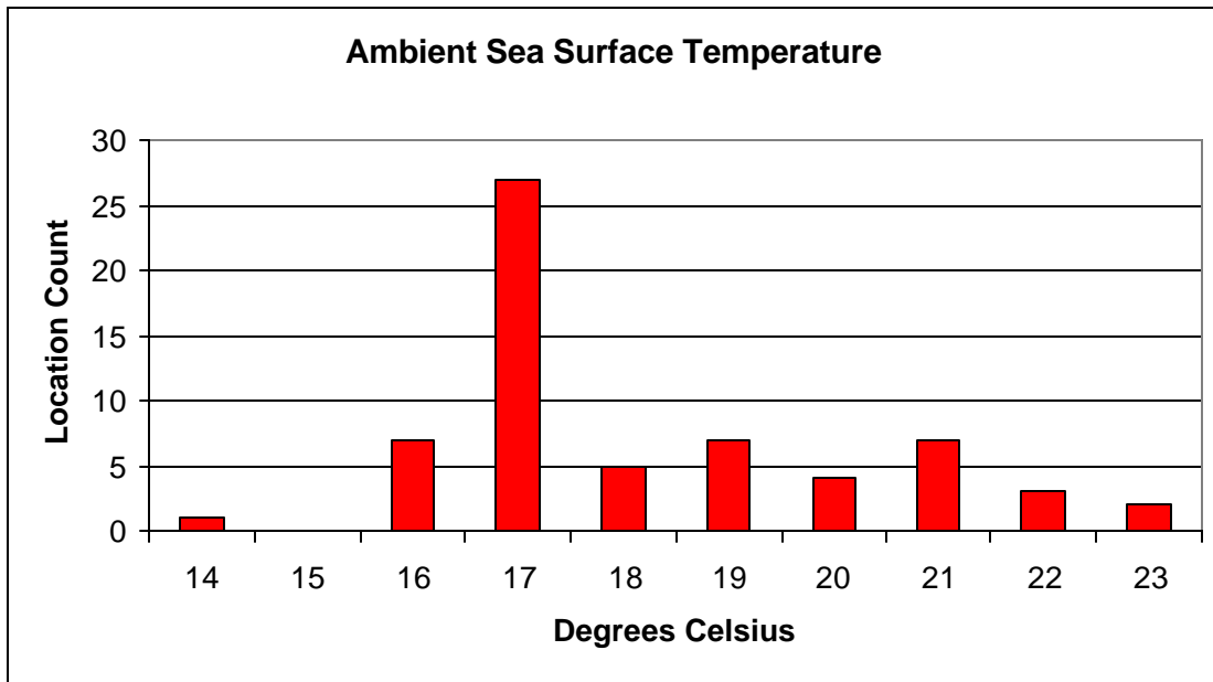
Figure 11. Counts of satellite telemetry locations for turtle # 137 overlaid on NOAA GOES SST datasets from the NOAA NESDIS archives. Data generated by Maptool (seaturtle.org, 2002)
