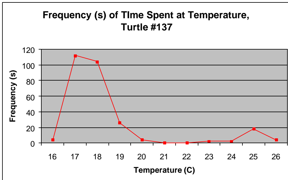
Figure 8. Frequency if time spent at different temperatures for turtle # 137 (total track).
