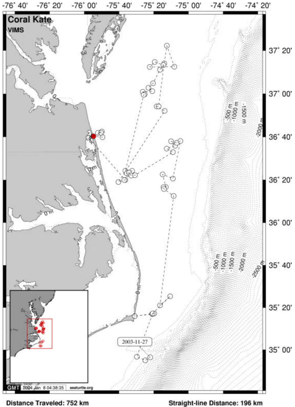
Figure 35. Satellite tracks of turtle #41136, from October 22 to November 27, 2003. Map generated by Maptool (seaturtle.org, 2002).
