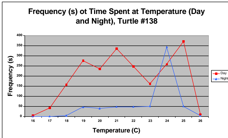
Figure 21 Frequency if time spent at different temperatures for turtle # 138, Day vs. Night.
