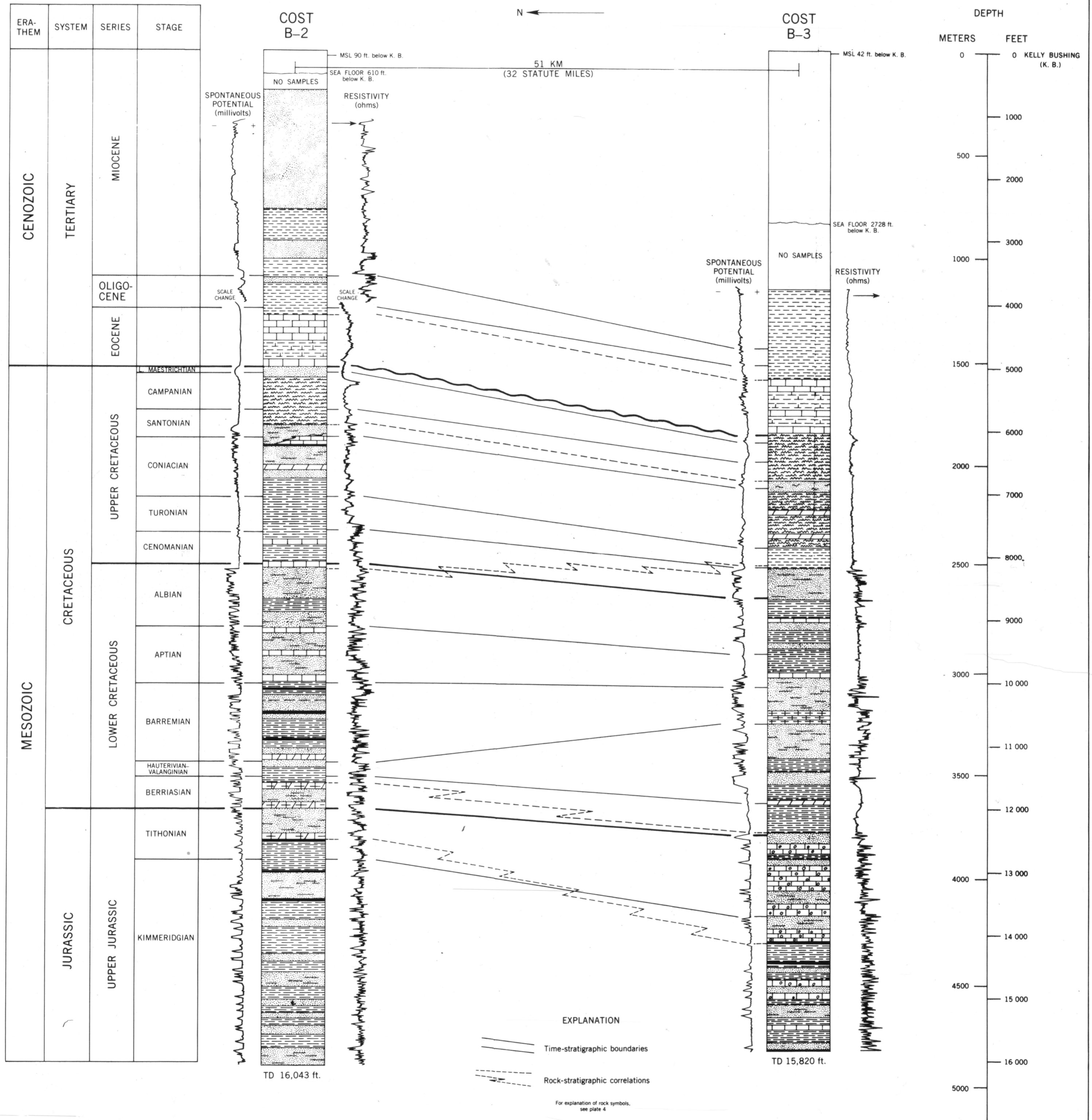
Plate 2. STRATIGRAPHIC CORRELATION OF COST WELLS B-2 AND B-3, U.S. MID-ATLANTIC CONTINENTAL MARGIN
