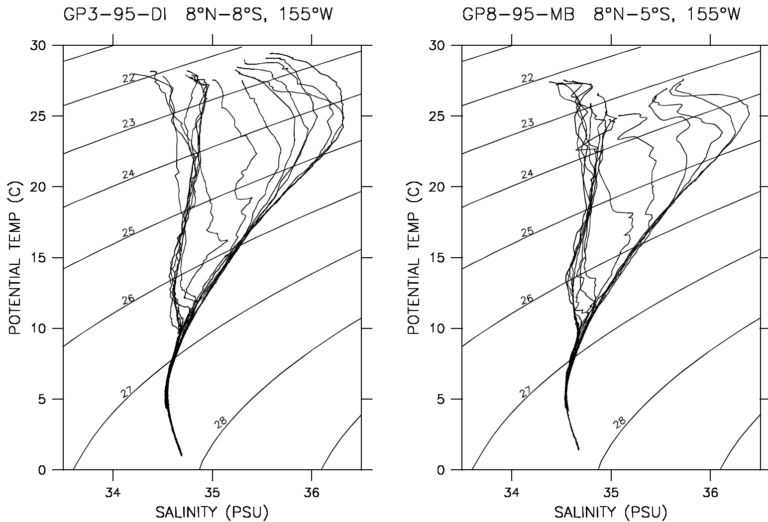
Fig. 56. GP3-95-DI spring and GP8-95-MB winter composite TS diagrams along 155°W.
