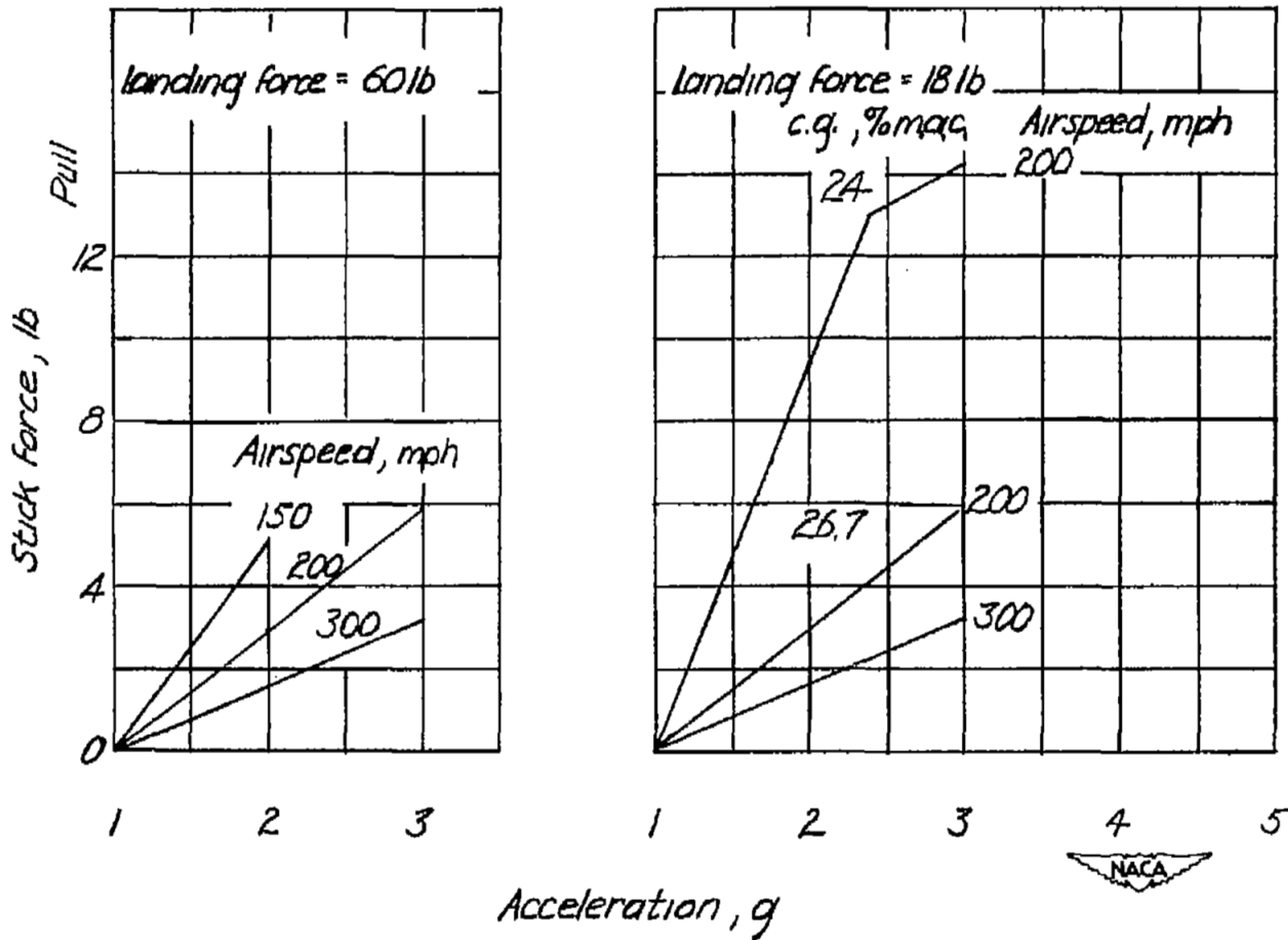
(a) Centering spring. Center of gravity, 26.7 percent mean aerodynamic chord.
