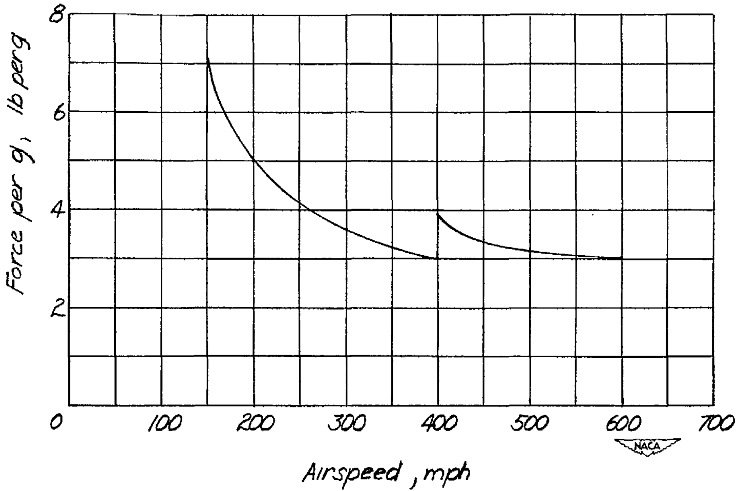
Figure 10.- Variation of stick force per g with airspeed for the centering-spring type of feel system with a variable spring constant and a 2-pound bobweight.
