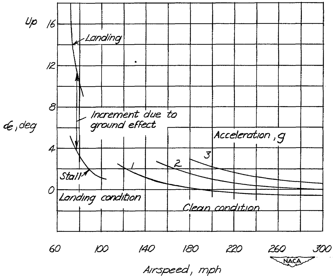
Figure 6.- Variation of elevator angle with airspeed and acceleration in the clean and landing conditions for the F4U-4B airplane. Center of gravity, 26.7 percent mean aerodynamic chord.
