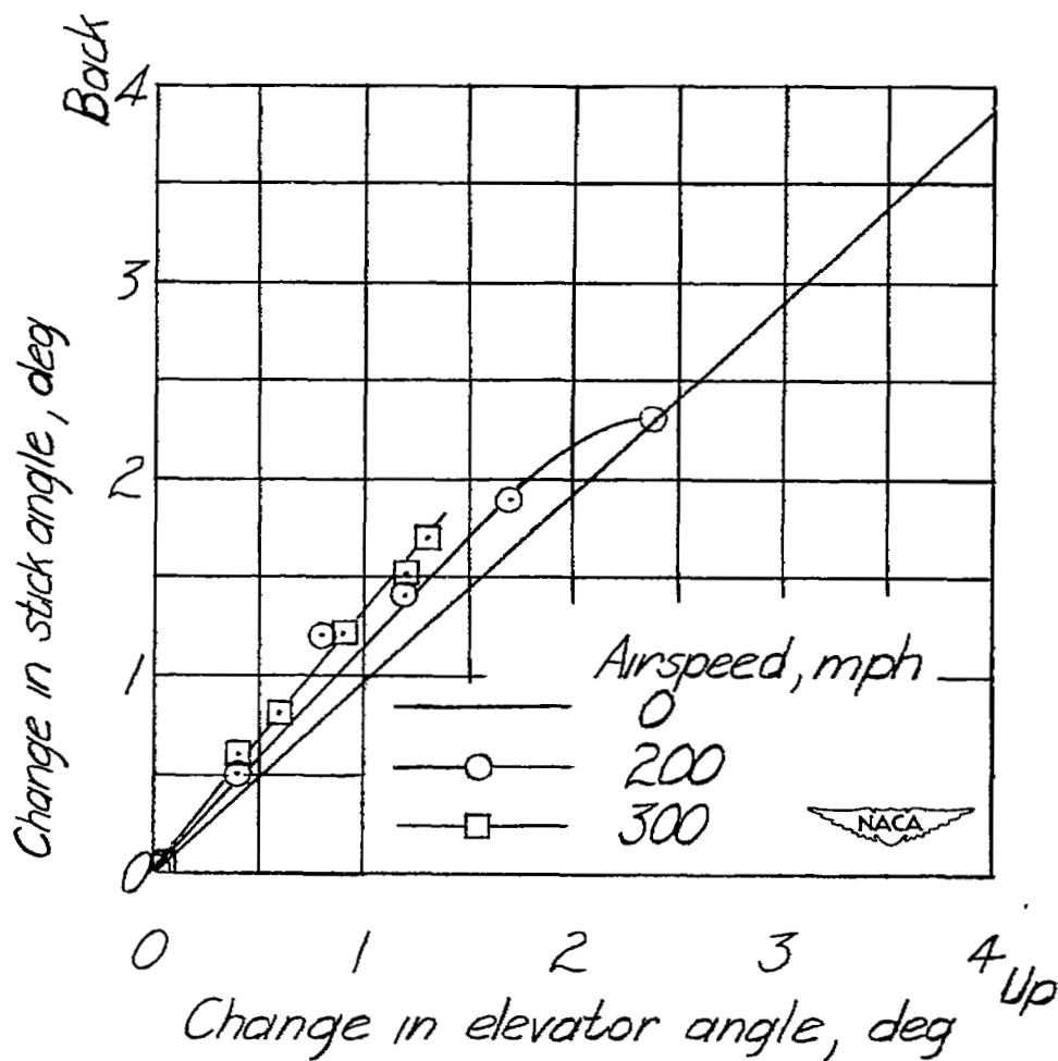
Figure 9.- Variation of elevator angle with stick angle at various airspeeds in the F4U-4B airplane.
