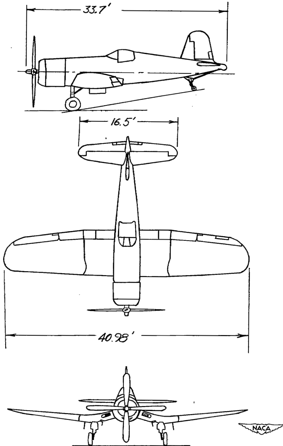
Figure 3.- Drawing of the F4U-4B airplane.
