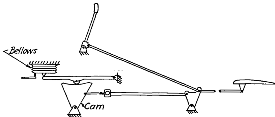
(a) Original feel system.
