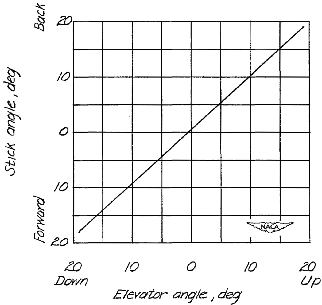
Figure 5.- Variation of stick angle with elevator angle for the F4U-4B airplane.
