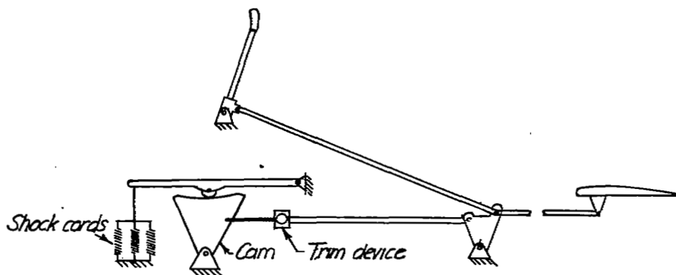
(b) Simple centering-spring feel system.
