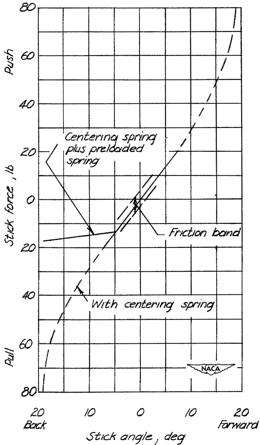
Figure 4.- Variation of the stick force with stick deflection for the various feel system arrangements.
