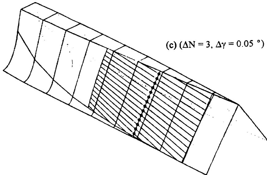
Fig. 1.9.3 Face gear tooth: localized bearing contact
