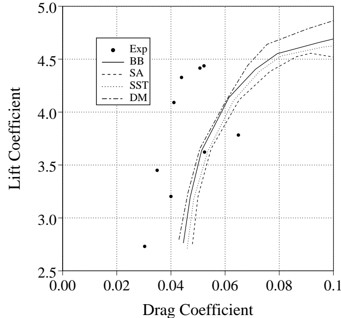
Fig. 13 Drag polar for geometry B and Re=9 million
