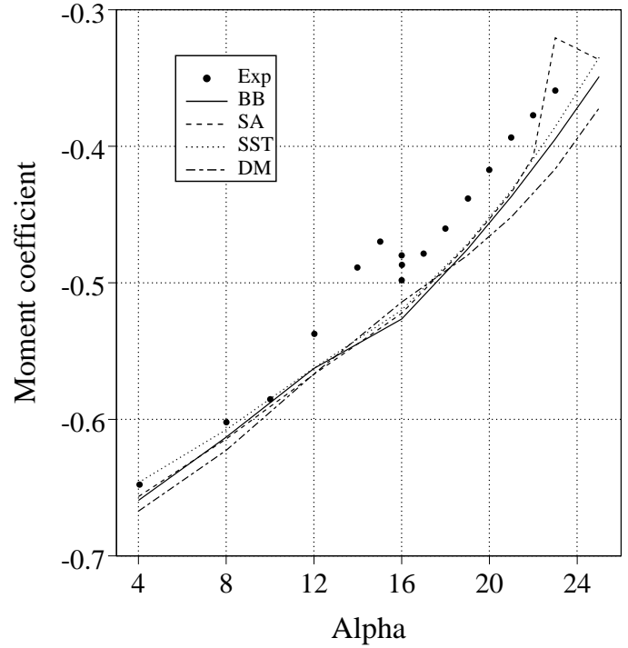
Fig. 12 C_m versus angle of attack for geometry B and Re=9 million
