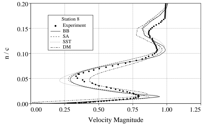
Fig. 8 Velocity profiles for Alpha=16 degrees, Geometry A, Re=9 million
