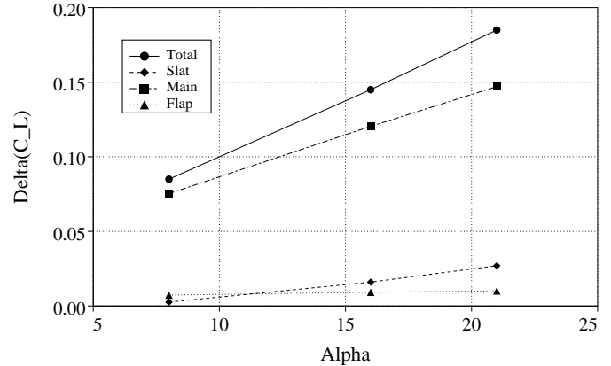
Fig. 3 Difference in C_l between wind-tunnel wall boundaries and a free-air outer boundary for geometry A and Re=9 million.
