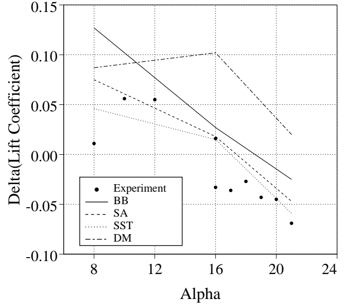
Fig. 16 Flap gap change: C_l (A) - C_l (B)
