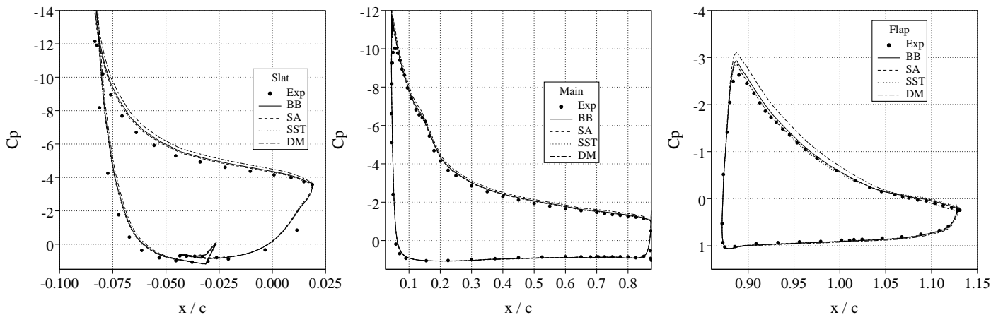
Fig. 6c Alpha=21 degrees
