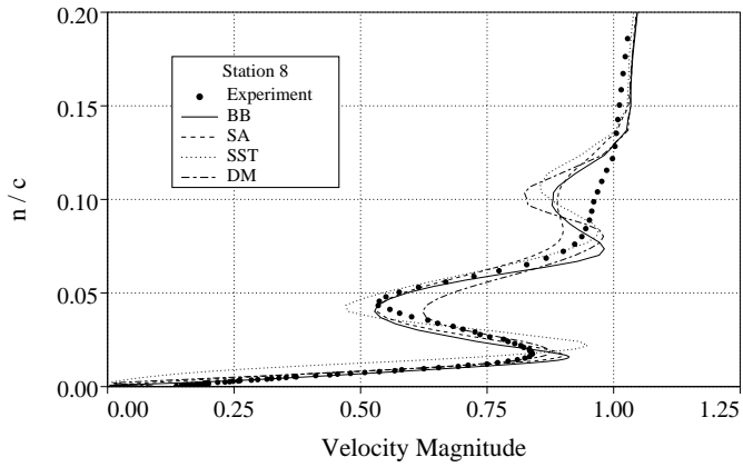
Fig. 7 Velocity profiles for Alpha=8 degrees, Geometry A, Re=9 million
