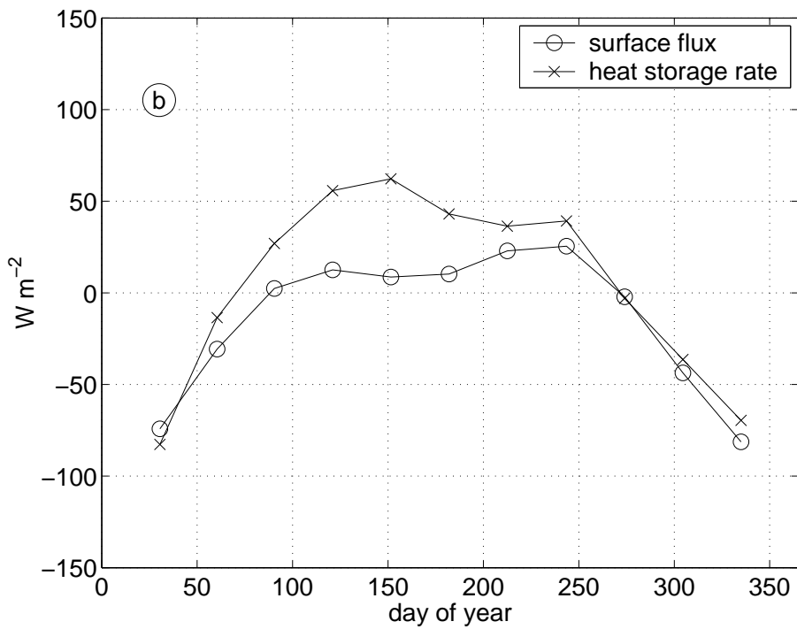
FIG. 10: The mean annual cycle of the surface flux and the heat storage rate based on observations collected in the tropical North Atlantic (5-25°N, 60-30°W) in the years 2000-2003. a) from non-float profiles. b) from all profiles.
