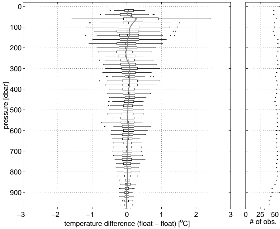
FIG. 4: Box and whisker plots (as in Fig. 1) of the temperature difference for adjacent float profiles in the tropical Atlantic ( 30^{\circ}\text{S} to 30^{\circ}\text{N} ), after exclusion of outliers. All considered profiles are within a 0.2^{\circ} by 0.5^{\circ} box (latitude by longitude) and were obtained within 5 days of each other.
