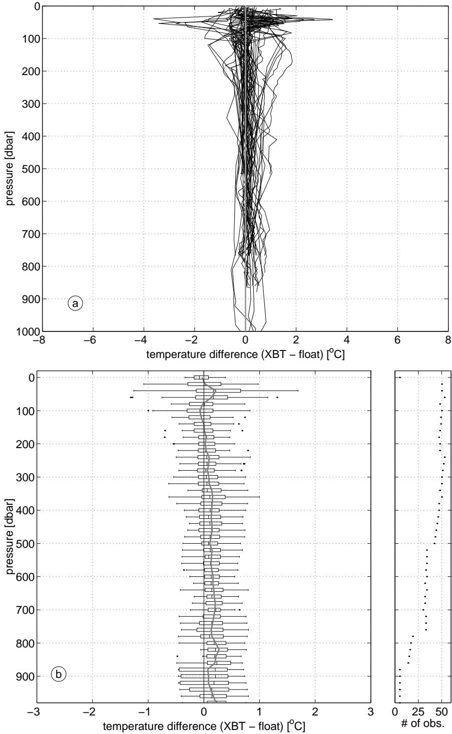
FIG. 5: Temperature difference in the North Atlantic (30°N to 55°N) between adjacent XBT and float profiles obtained within 5 days of each other. All considered profiles are within a 0.2° by 0.5° box (latitude by longitude). (a) all profiles. (b) box and whisker plot after exclusion of outliers (as in Fig. 1).
