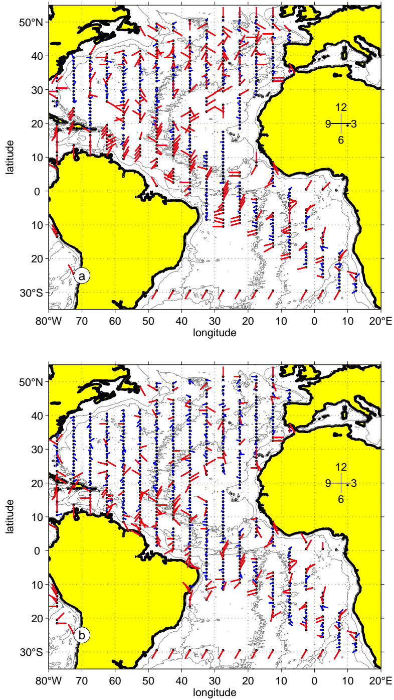
FIG. 8: Seasonal bias for the profiles obtained in the year 2002. The direction of the lines gives the phase (months 1-12) and the length gives the amplitude (0-1) of the bias. The inset cross-hair represents an amplitude of 1 for four different months. If the amplitude is less (more) than 0.5 the lines are blue (red). a) for non-float profiles, based on 6346 profiles in 567 boxes. b) for all profiles, based on 11886 profiles in 667 boxes.
