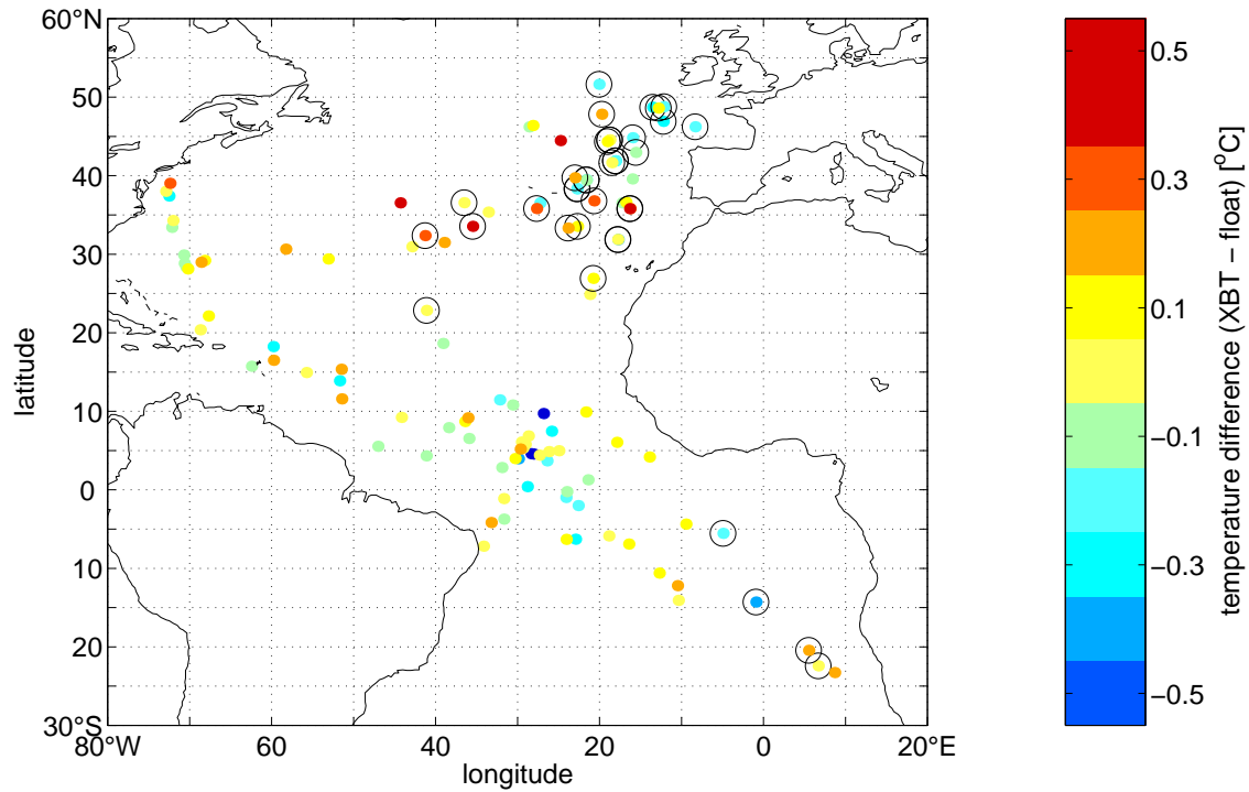
FIG. 6: Map showing mean temperature differences between adjacent XBT and float profiles obtained within 5 days of each other. The means were obtained for the layer below 250 dbar. All considered profiles are within a 0.2^\circ by 0.5^\circ box (latitude by longitude). Highlighted by circles are temperature differences associated with profiles from PROVOR floats, because they have the highest data density in the eastern North Atlantic.
