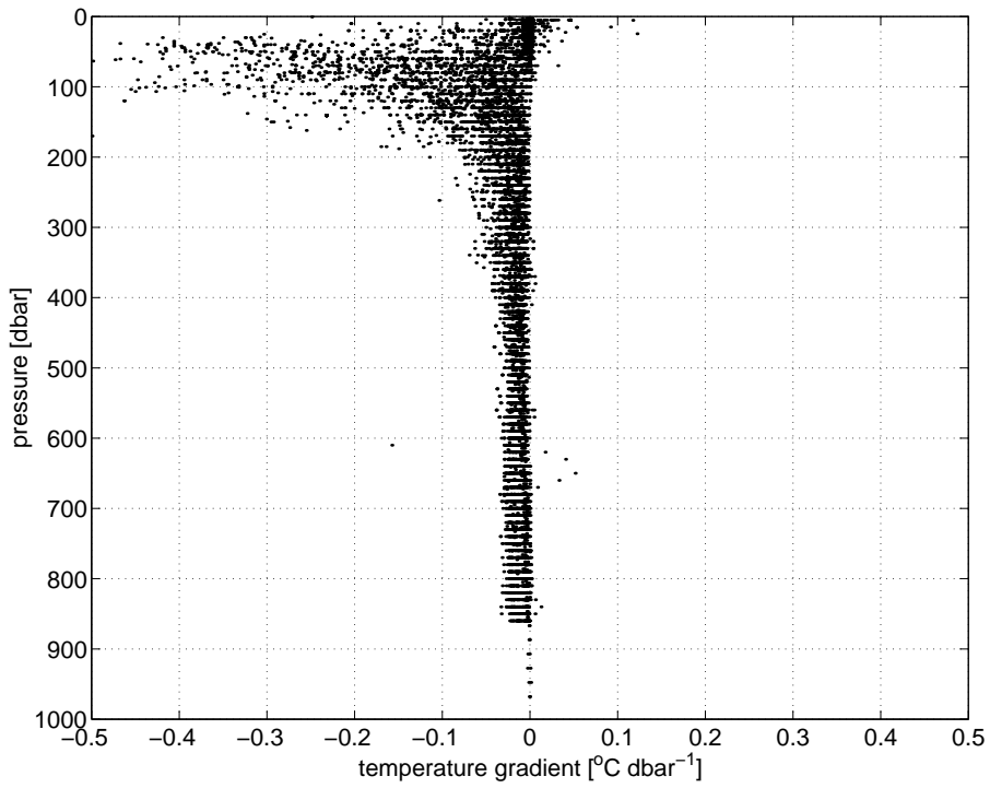
FIG. 3: The vertical temperature gradient (\delta T / \delta p)^{-1} , with T = temperature and p = pressure) in the tropical Atlantic from profiling floats.
