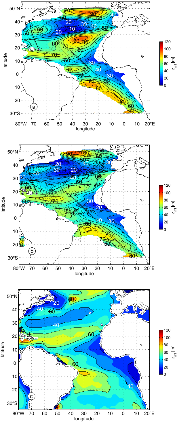
FIG. 9: a) Annual mean of the mixed layer thickness in the year 2002 for non-float profiles, based on 6346 profiles in 567 boxes. b) Annual mean of the mixed layer thickness in the year 2002 for all profiles, based on 11886 profiles in 667 boxes. c) Climatology of the mixed layer thickness from World Ocean Atlas 2001 (Conkright et al., 2002).
