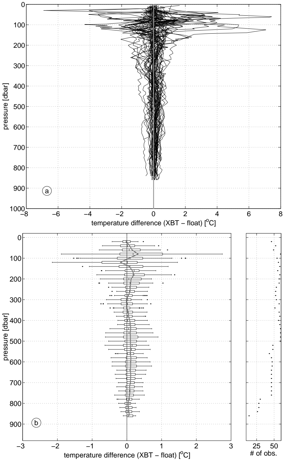
FIG. 1: Temperature difference in the tropical Atlantic ( 30^{\circ}\text{S} to 30^{\circ}\text{N} ) between XBT and float profiles located within a 0.2^{\circ} by 0.5^{\circ} box (latitude by longitude) that were obtained within 5 days of each other. (a) all profiles. (b) box and whisker plot after exclusion of large outliers (see section 2). The box has lines at the lower quartile, median, and upper quartile values. The whiskers are lines extending from each end of the box to show the extent of the data that are not considered outliers. The remaining outliers are marked with dots. The grey line follows the means. The panel to the right is part of (b) and shows the number of data points available for the statistical estimates at each level.
