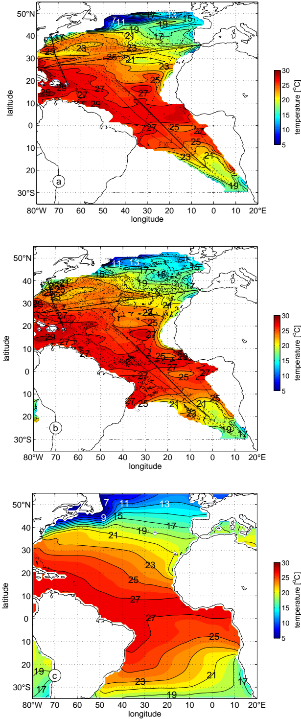
FIG. 7: a) Annual mean of the mixed layer temperature in the year 2002 for non-float profiles, based on 6346 profiles in 567 boxes. b) Annual mean of the mixed layer temperature in the year 2002 for all profiles, based on 11886 profiles in 667 boxes. c) Climatology of the surface temperature from World Ocean Atlas 2001 (Conkright et al., 2002).
