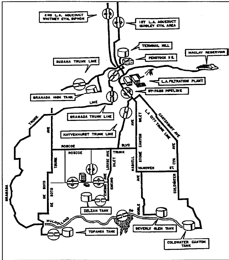
Figure 2-4. Water System Damage, Northridge Earthquake (Courtesy of LAFD)
