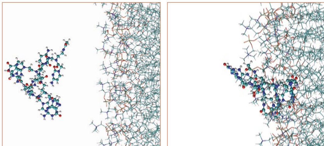
Results from a computer simulation showing an information molecule “sticking” to the protocell’s container.
