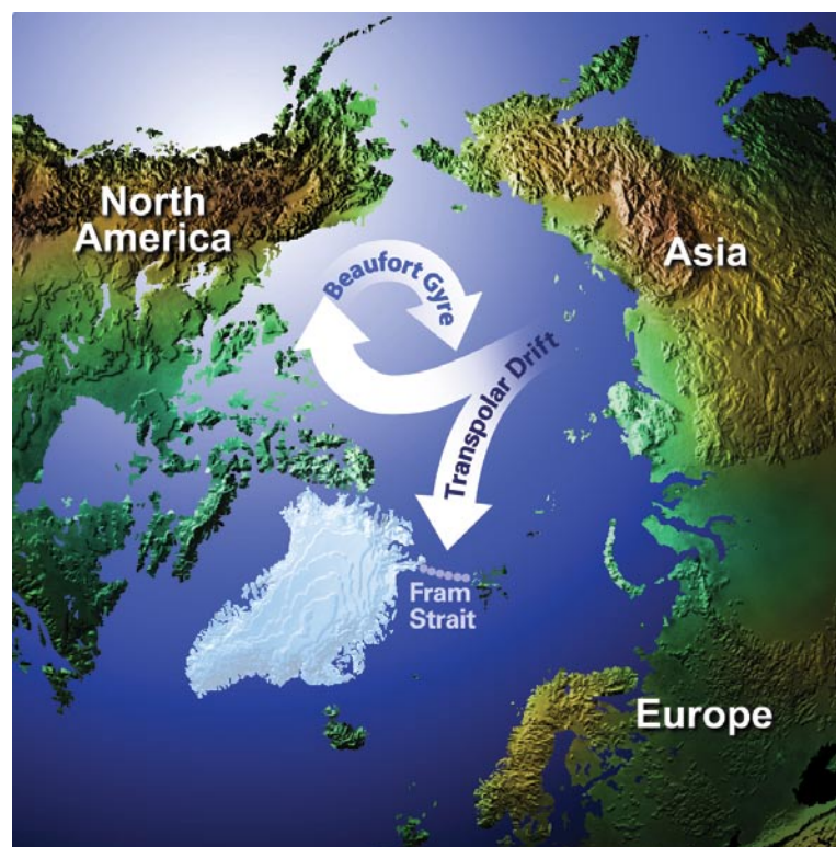
Top: Bill Lipscomb’s height relative to an Arctic sea ice ridge. Right: The two main sea ice drift systems in the Arctic Ocean, the Beaufort Gyre and the Transpolar Drift.
