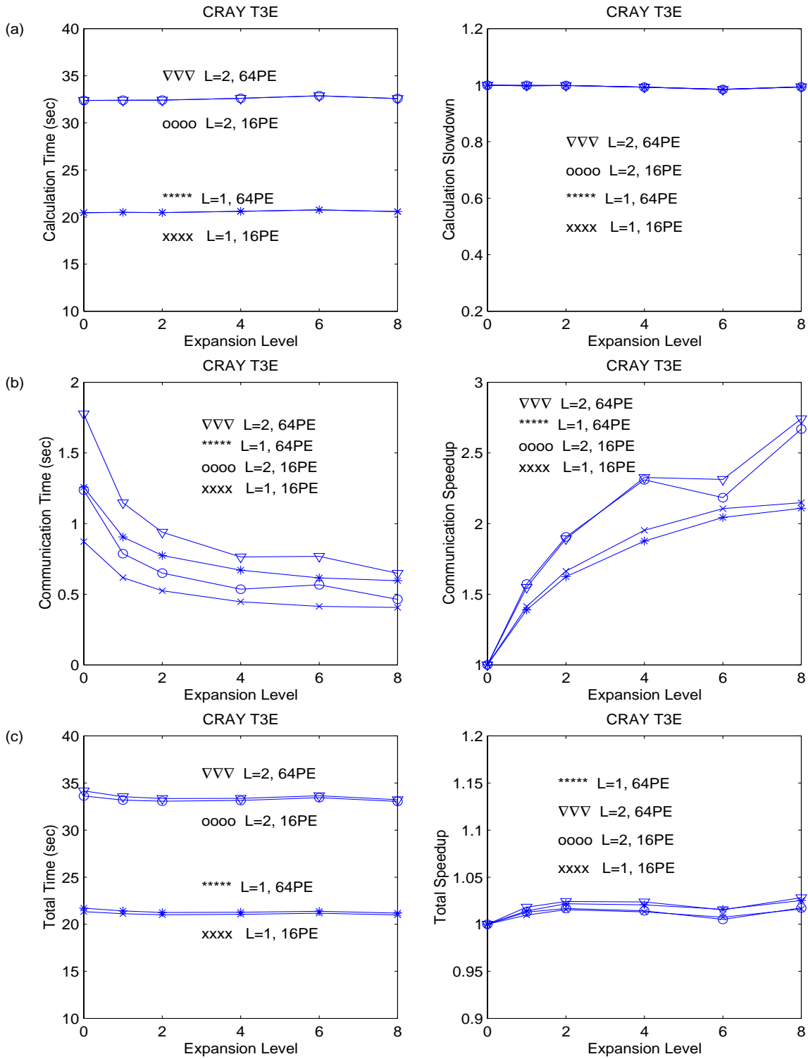
Figure 5: (a) calculation time and slowdown, (b) communication time and speedup, (c) total time and speedup for these four tests on Cray T3E.
