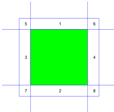
Figure 2: Illustration of ghost cells in 2D. Shaded area is active region (subdomain). 4 ghost cells blocks (1,2,3,4) are from immediate neighbors ( horizontal and vertical neighbors). Another 4 corner ghost cell blocks (5,6,7,8) are from 2nd nearest neighbors (diagonal processors). In 3D, there will be 6 ghost cell blocks from immediate neighbors, 12 planar corner blocks from 2nd nearest neighbors, and 8 cubic corner blocks from 3rd nearest neighbors.
