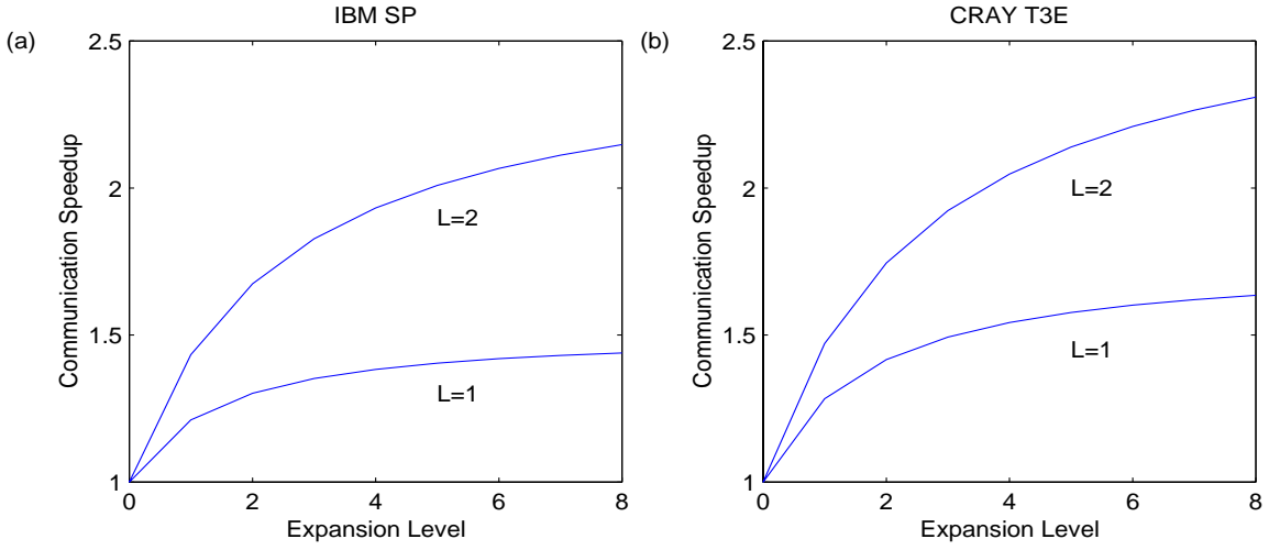
Figure 3: Communication speedup as the function of the ghost cells layers required level L and expansion level e for a 2D domain decomposition. Here n_x = n_y = 800 .
