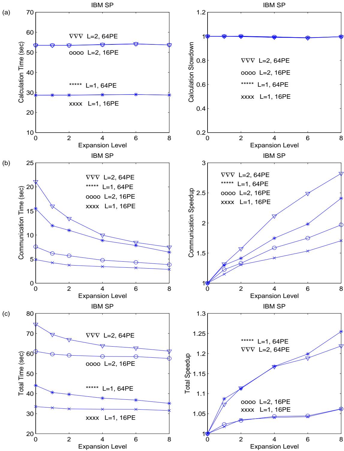
Figure 4: (a) calculation time and slowdown, (b) communication time and speedup, (c) total time and speedup for these four tests on IBM SP.
