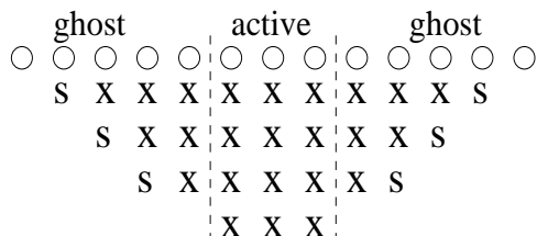
Figure 1: An illustration of field update for L = 2, e = 3 for a 1D domain decomposition. 2D and 3D decompositions are similar. Note that active cell region are far larger than ghost cell regions in real applications. Also, even though we only need to updating fields in active cells, some fields in ghost cells are updated in order to maintain the correct timeliness.
