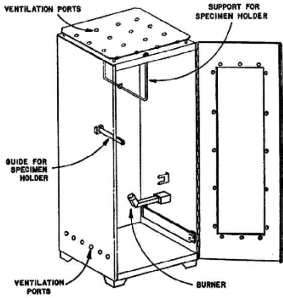
VERTICAL TEST CABINET
