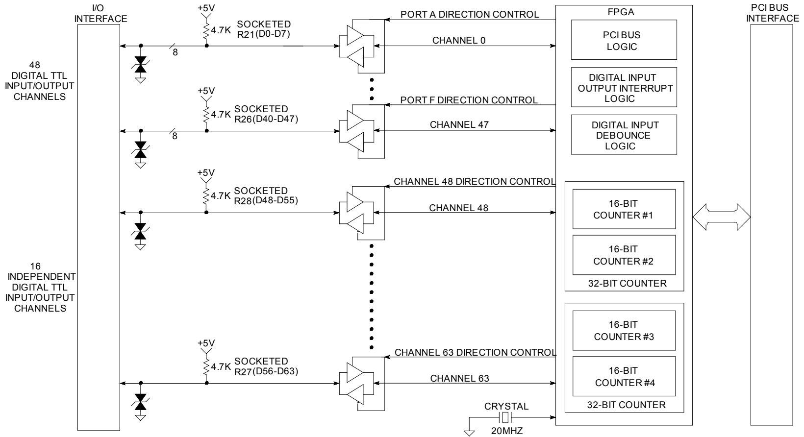
PMC, APC, AcPC464 BLOCK DIAGRAM
