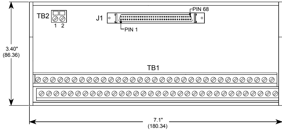
TOP VIEW
