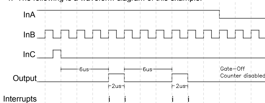
Figure 3.3: PWM waveform
