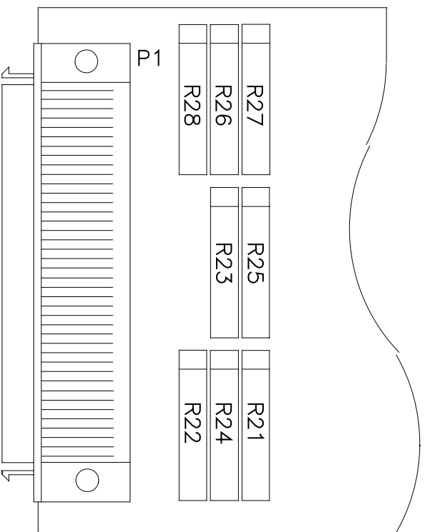
PMC, APC, AcPC464 RESISTOR LOCATIONS
