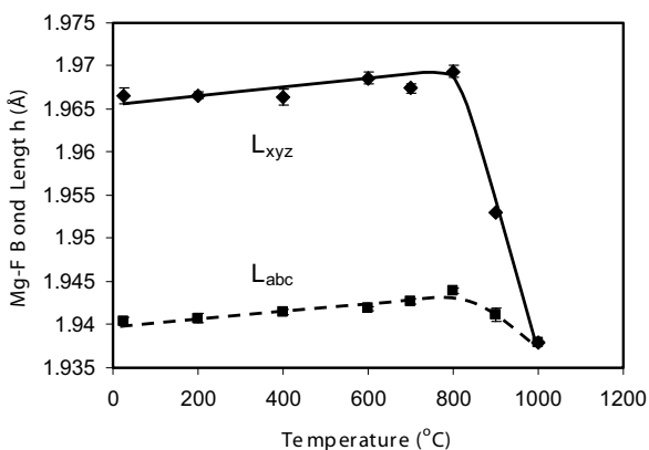
FIGURE 5. Mean (Mg-F) bond length of NaMgF 3 at 4 GPa derived from atomic coordinates ( L_{xyz} ) and from the lattice parameters ( L_{abc} ). Bars attached to the symbols represent the experimental errors.
