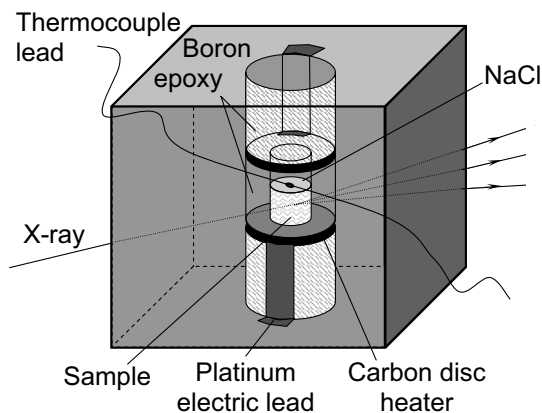
FIGURE 1. Cubic high pressure cell assembly for monochromatic X-ray diffraction experiments.
