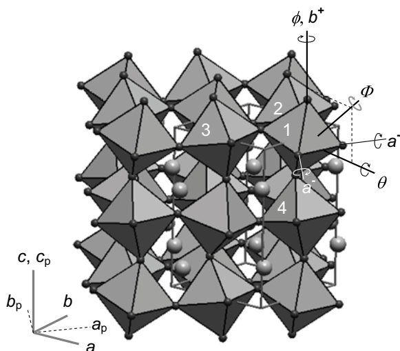
FIGURE 4. Crystal structure of NaMgF 3 at 700 °C and 4 GPa. Dark and grey spheres represent F and Na, respectively. Octahedra represent the MgF 6 sites. The unit cell ( Pbnm ) and a , b , c distances are shown in the structure. a p , b p , c p represent the dimensions of the pseudo-cubic cell ( a p = a /√2, b p = b /√2, c p = c /2, Z = 1). ( a p , b p , c p ) axes: any consecutive two octahedra (e.g., 1 and 3) about (100) p axis tilt in opposite direction; any consecutive two octahedra (e.g., 1 and 2) about (010) p axis also tilt in the opposite direction, and the magnitude of tilting about (100) p and (010) p are the same; and any two consecutive octahedra (e.g., 1 and 4) about (001) p axis tilt in the same direction. \phi and \theta indicate the two independent tilting angles about (001) p and (110) p , which define a compound angle \Phi about the “threefold axes” (111) p .
