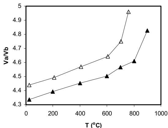
FIGURE 8. The V_A/V_B ratio of the NaMgF 3 structure at 4 GPa (solid symbols) and ambient pressure (open symbols, after Zhao et al. 1993a).
