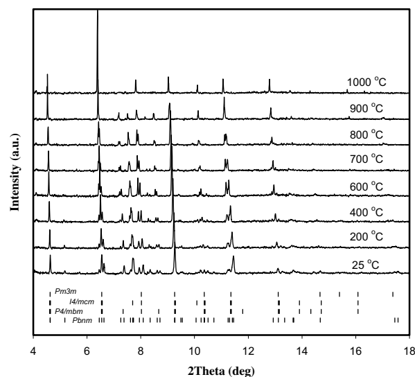
FIGURE 2. X-ray diffraction patterns of NaMgF 3 collected using imaging plate and a monochromatic beam ( E = 40.61 keV) at 4 GPa.
