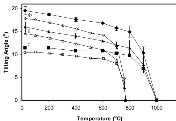
FIGURE 7. The octahedral tilting angle \Phi , \theta , and \phi of the NaMgF 3 structure at 4 GPa (solid symbols) and ambient pressure (open symbols, after Zhao et al. 1993a). The bars attached to the symbols represent the experimental errors (some are smaller than the symbols).
