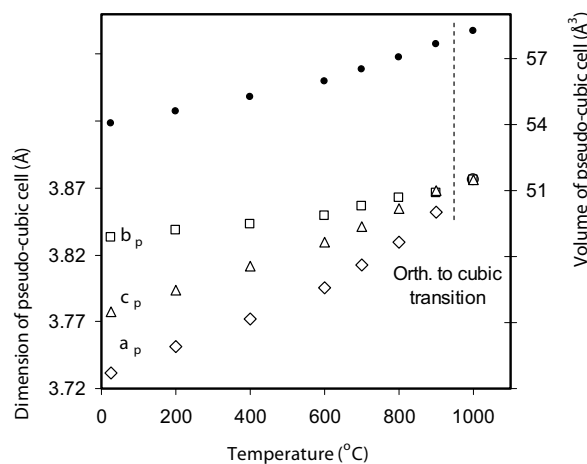
FIGURE 3. Temperature dependence of the pseudo-cubic cell ( a_p = a/\sqrt{2}, b_p = b/\sqrt{2}, c_p = c/2, V_p = V/4, Z = 1 ) of NaMgF 3 at 4 GPa. Experimental uncertainties of the data are less than the size of the symbols.
