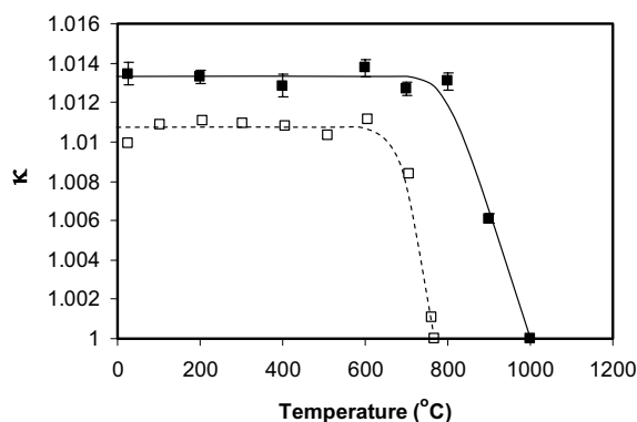
FIGURE 6. Ratio of the bond length ( L_{xyz} ) derived from atomic coordinates ( x, y, z ) to that ( L_{abc} ) derived from the lattice parameters ( a, b, c ) of NaMgF 3 at 4 GPa (solid symbols) and ambient pressure (open symbols, after Zhao et al. 1993a). Bars attached to the symbols represent the experimental errors.
