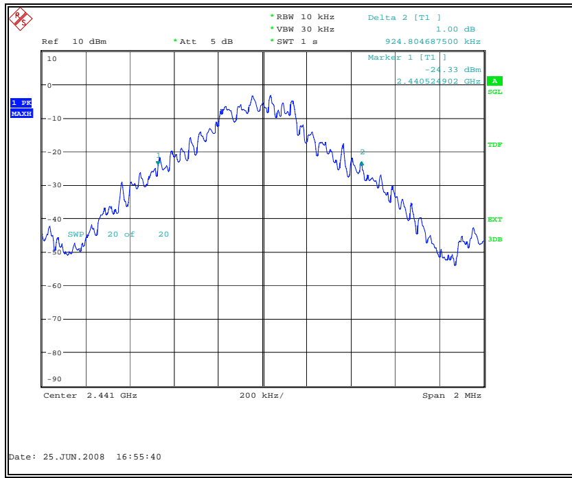
Fig. 27 20dB Bandwidth: Channel 39
