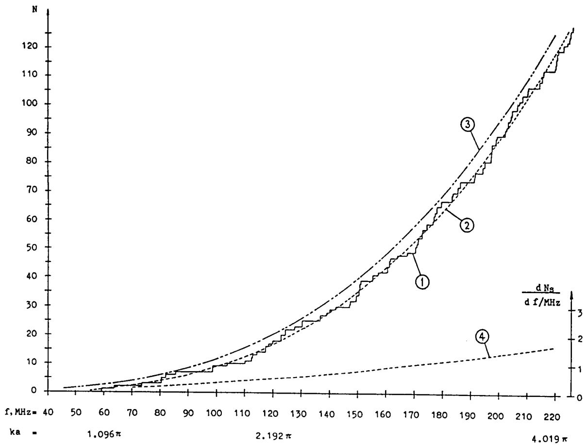
Figure 4. Mode number (curve 1), smooth approximation to the mode number (curve 2), Weyl approximation to the mode number (curve 3), and smooth mode density (curve 4) for the NIST reverberation (2.74 m \times 3.05 m \times 4.57 m).
