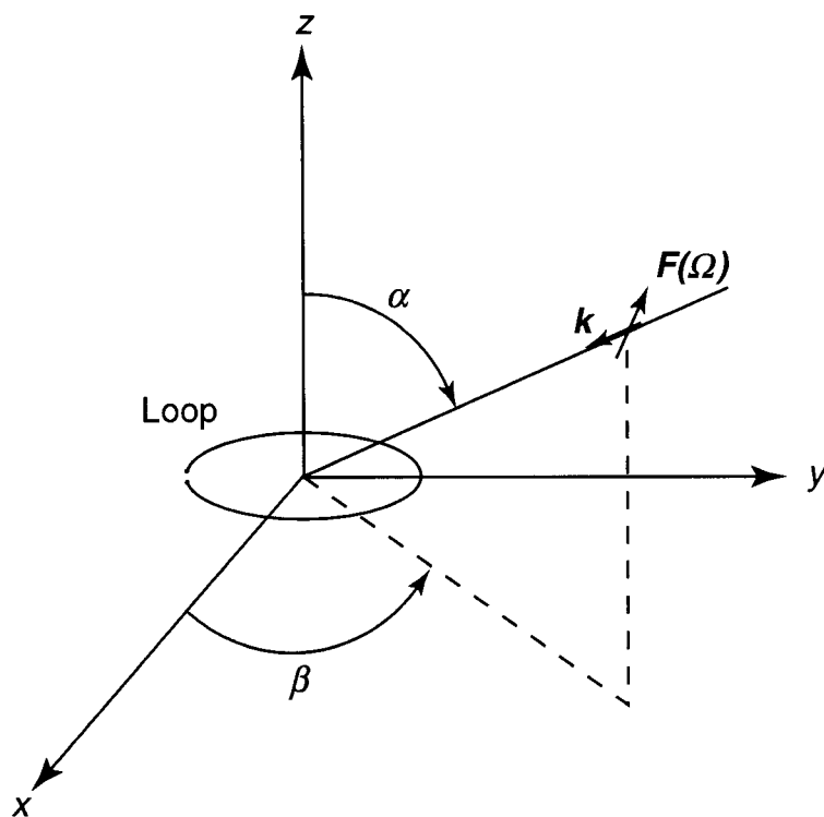
Figure 22. Loop antenna illuminated by a plane-wave component of the electric field.
