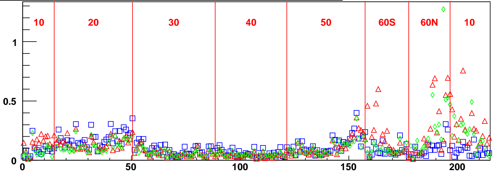
BG/S of A 2.5 MHz Component for all BPMs, Shot 1
