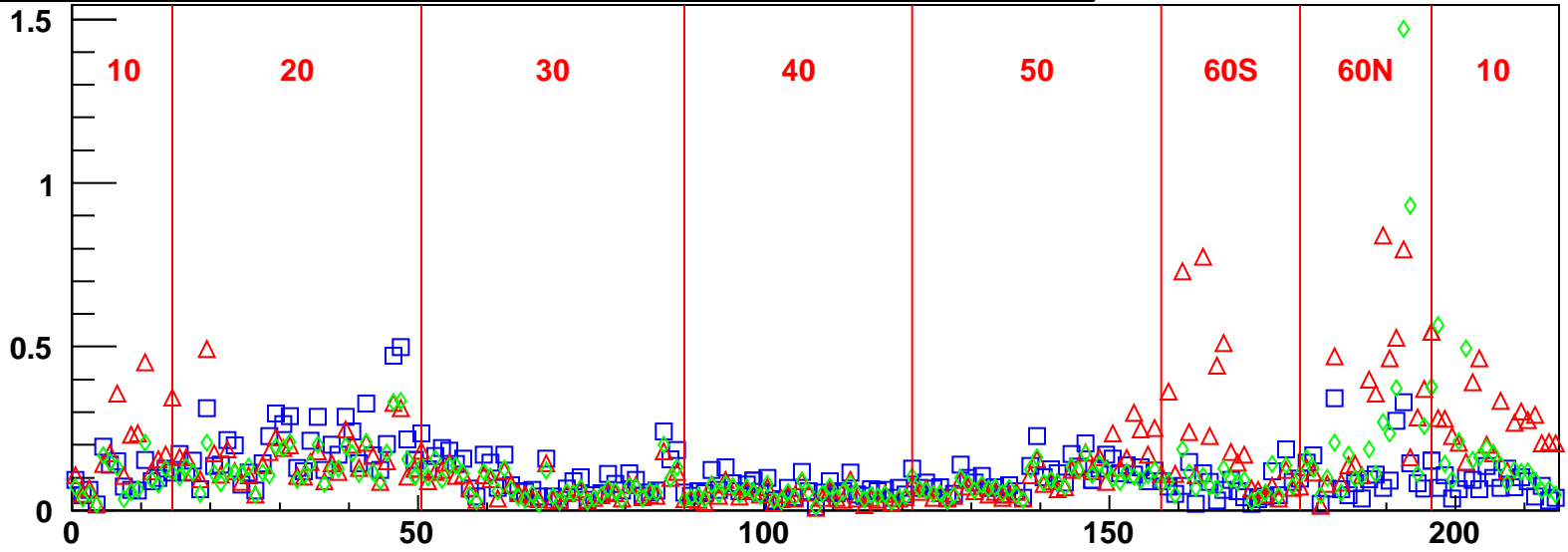
BG/S of B 2.5 MHz Component for all BPMs, Shot 1
