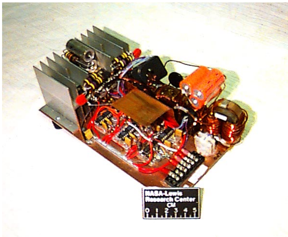
Figure 2. Miniaturized arcjet PPU breadboard.
