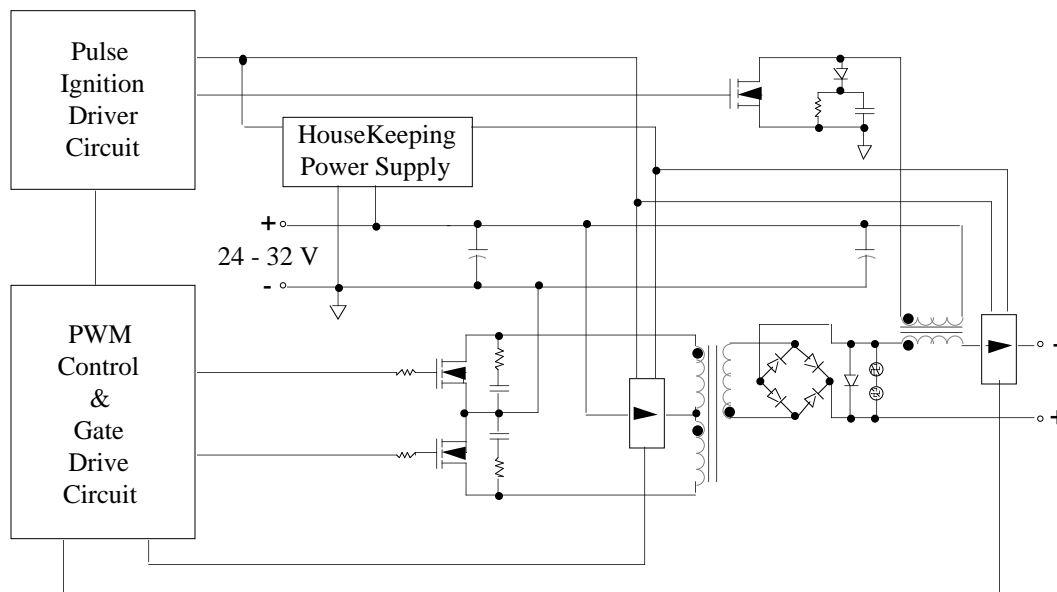
Figure 1. Miniaturized arcjet PPU schematic.
