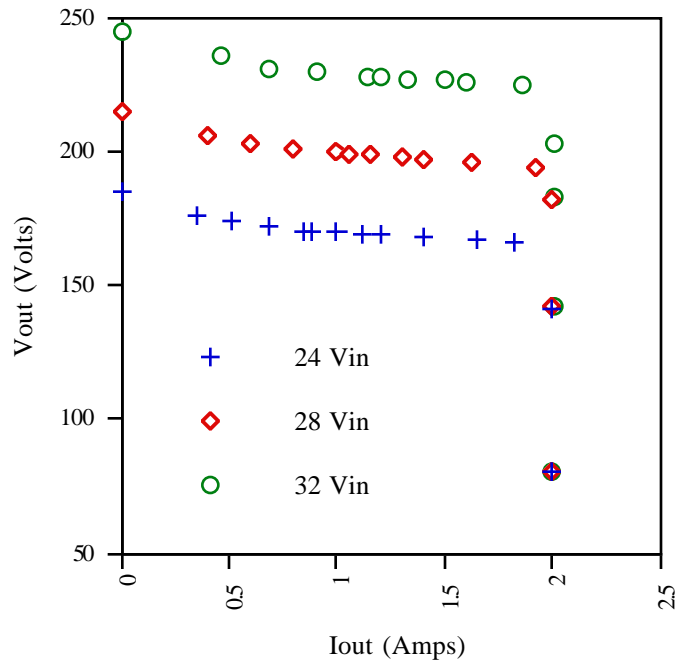
Figure 3. Miniaturized arcjet PPU output characteristics at 2.0 A output current and various input voltages.
