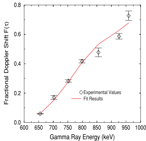
Figure 2. The experimental F(\tau) and the fit produced by the program FITFTAU for the transitions in TSD1.
