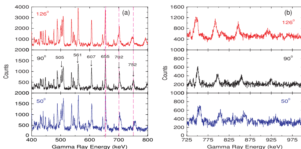
Figure 1. The Doppler shift of transitions in TSD1 observed at 50^\circ , 90^\circ and 126^\circ ( 122^\circ and 130^\circ combined), respectively. The spectra (a) show the transitions from lower spin states and (b) show the transitions from higher spin states in TSD1.
