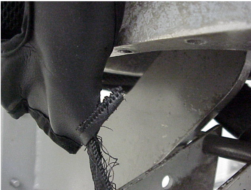
Helmet Photograph 10. Retention Water Immersed Vance Leather, 200, M
