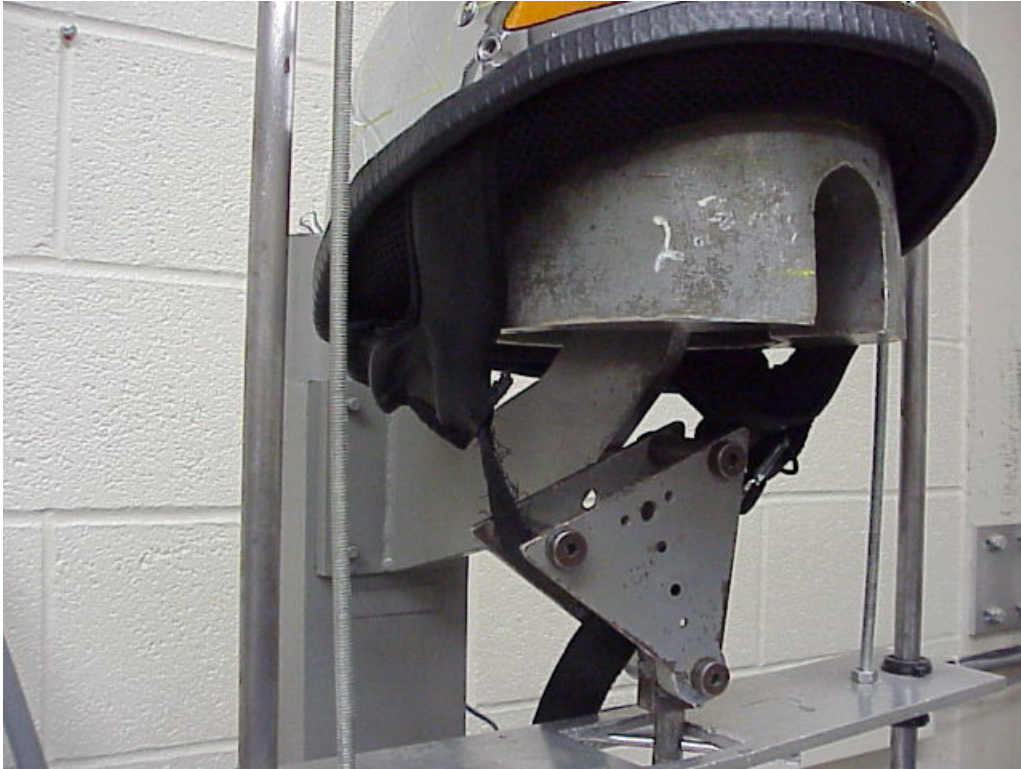
Helmet Photograph 9. Retention Water Immersed Vance Leather, 200, M
